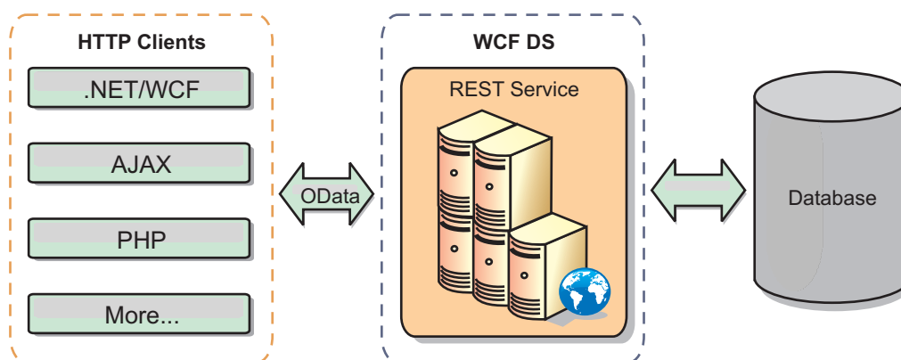
Figura 39. Microsoft WCF Data Services
