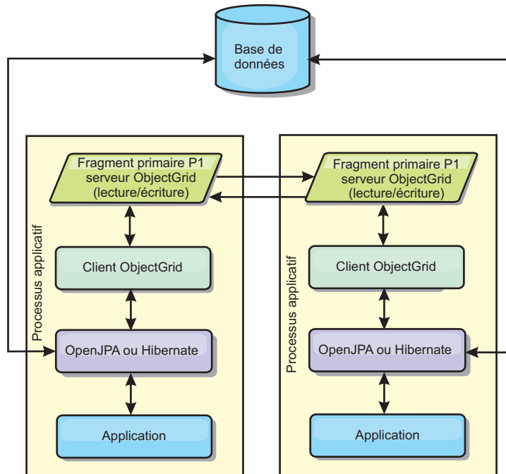
Figure 40. Topologie intra-domaine JPA
