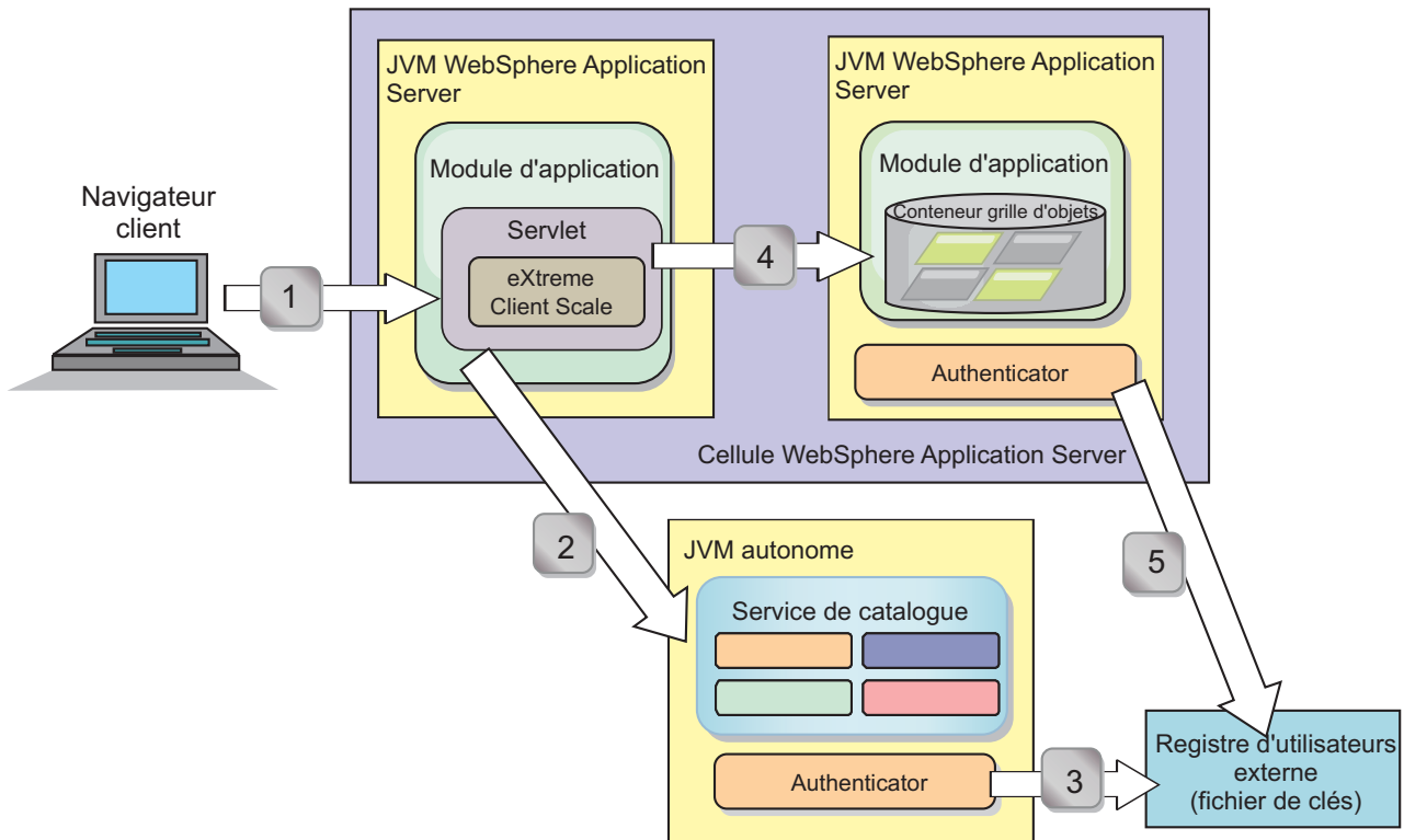
Figure 21. Flux d'authentification
