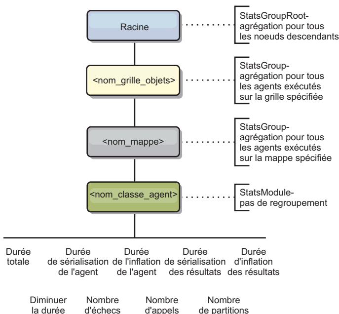
Figure 64. Structure agentManagerModule
