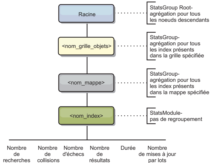
Figure 62. structure de module hashIndexModule
