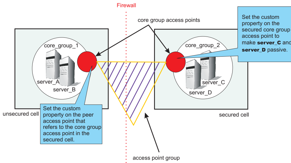
Figure 11. Configuring the FW_PASSIVE_MEMBER custom property
