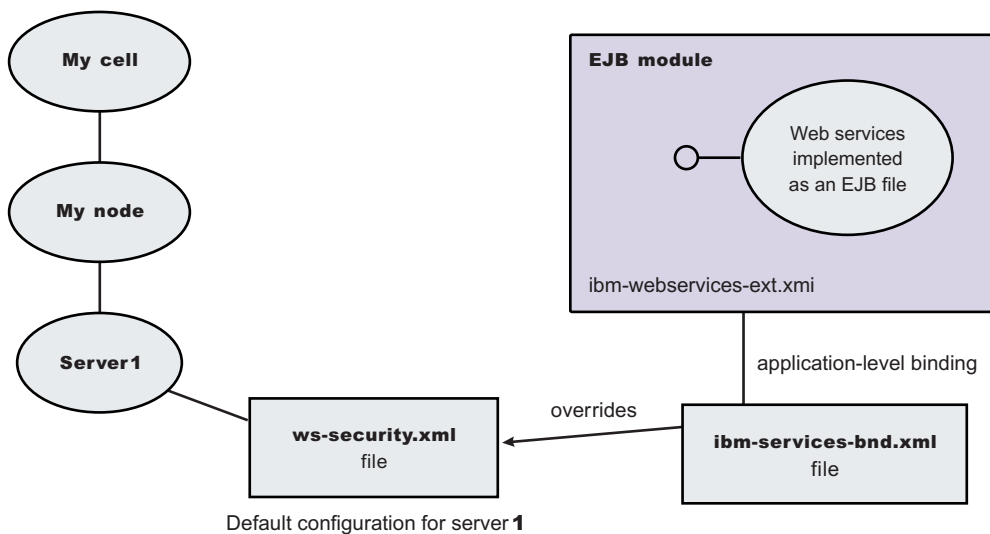
Figure 17. Configuration when using the addNode command
