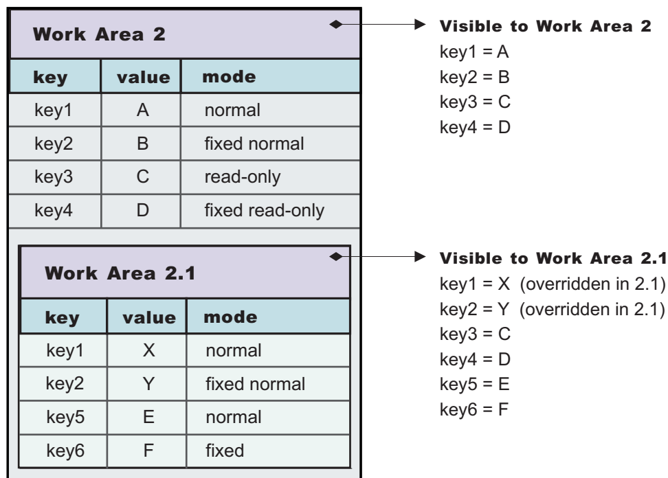
Figure 30. Redefining existing properties in nested work areas
