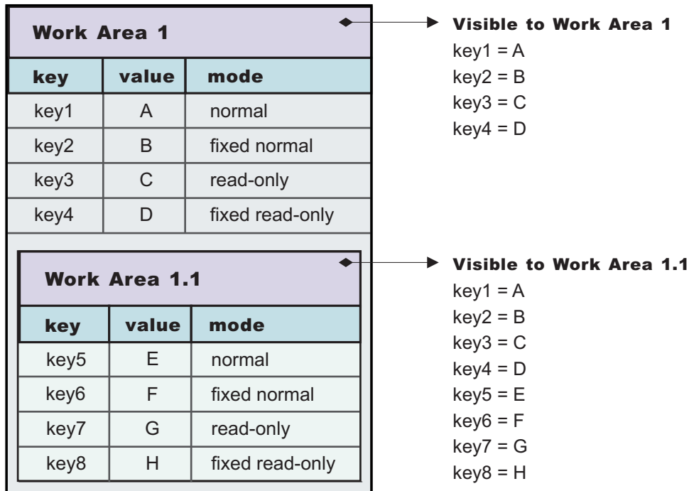
Figure 29. Defining new properties in nested work areas
