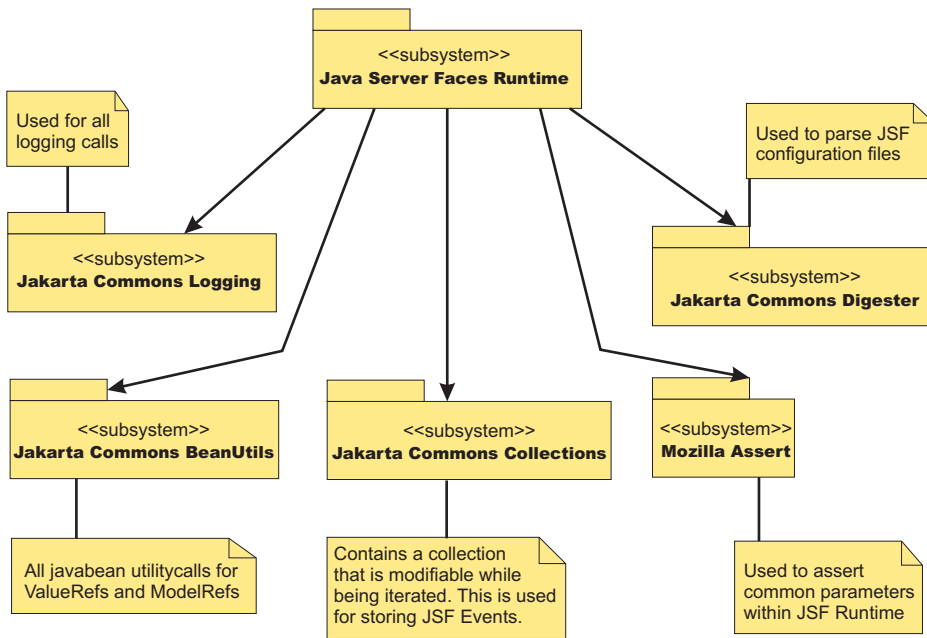
Figure 3. Current external API dependencies from the Sun based JSF runtime
