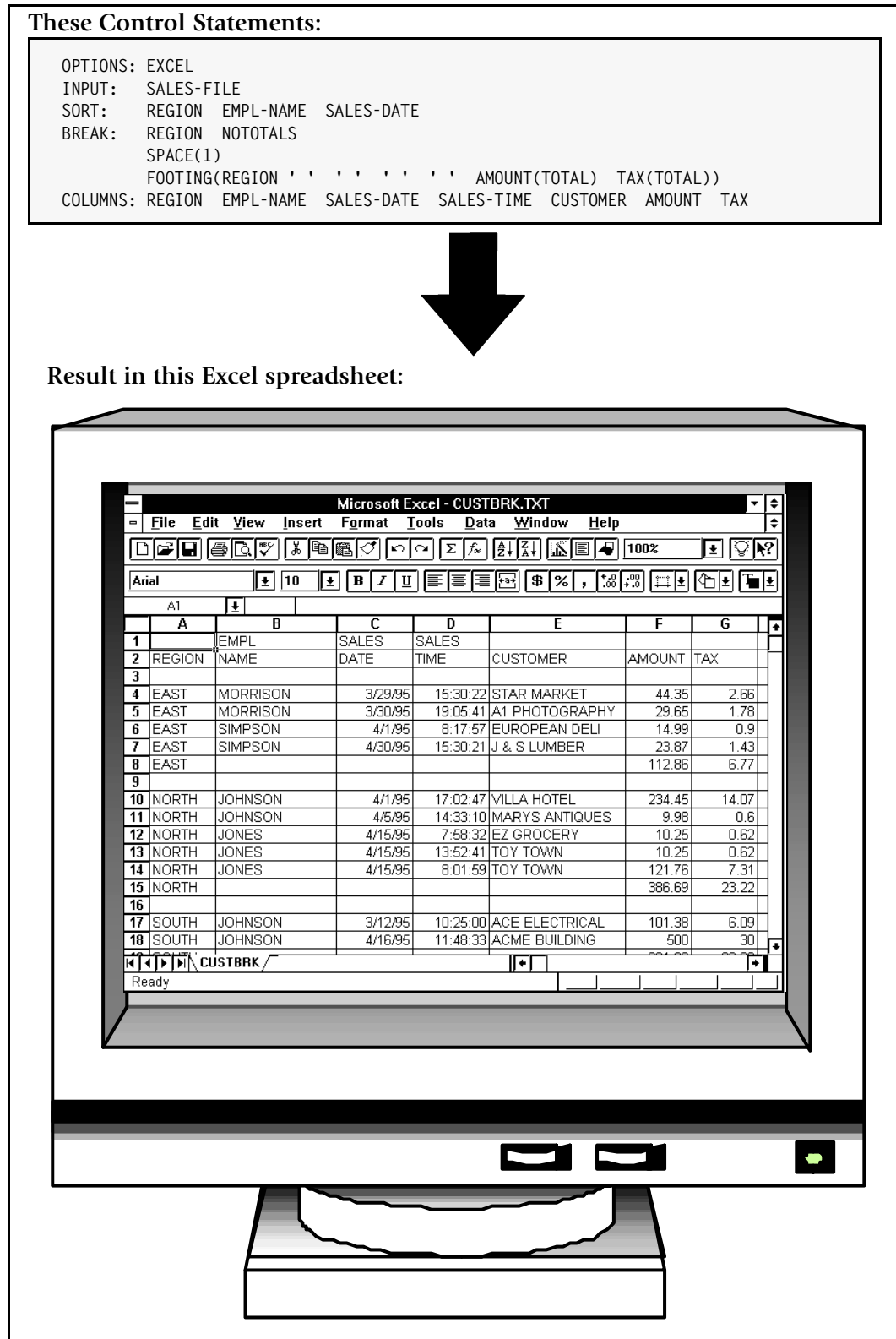
Figure 3-10 • Using FOOTING parms to customize the total row and create blank rows
