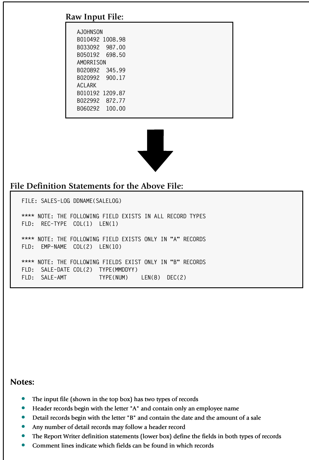
Figure 4-43 • An input file with header and detail records, and its definition statements
