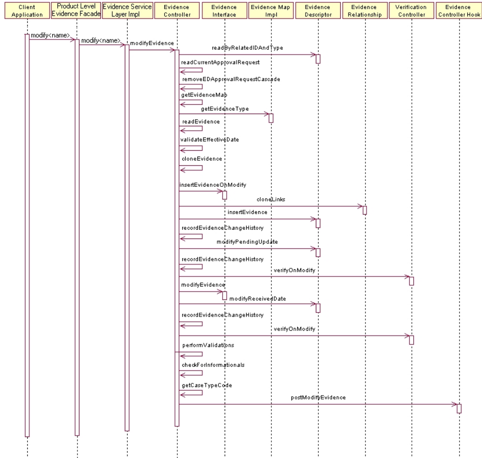
Figure 3.2 Sequence Diagram for Modifying Evidence
