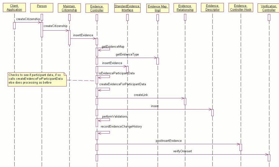
Figure 4.3 Participant Evidence Sequence
