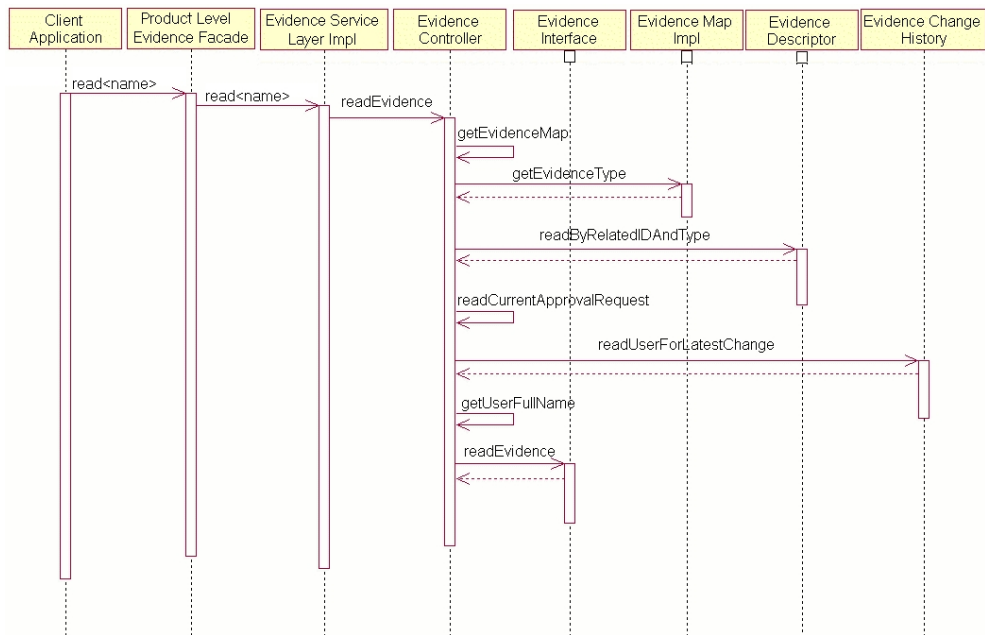
Figure 3.3 Sequence Diagram for Viewing Evidence
