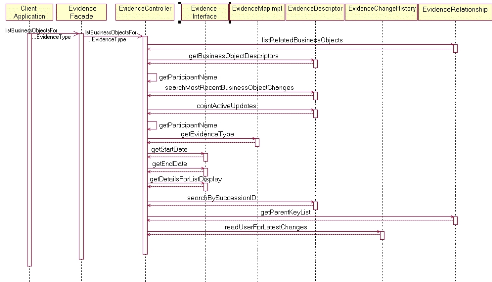
Figure 3.4 Sequence Diagram for Listing Evidence
