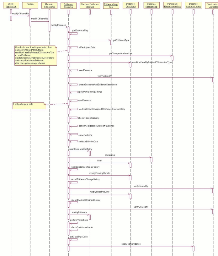
Figure 4.5 Modify participant
