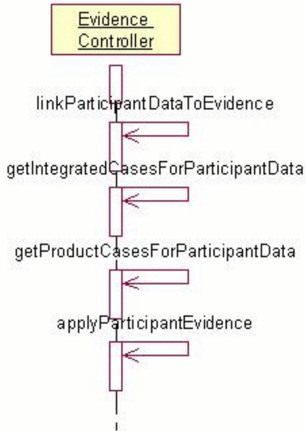
Figure 4.4 Evidence Sequence Diagram
