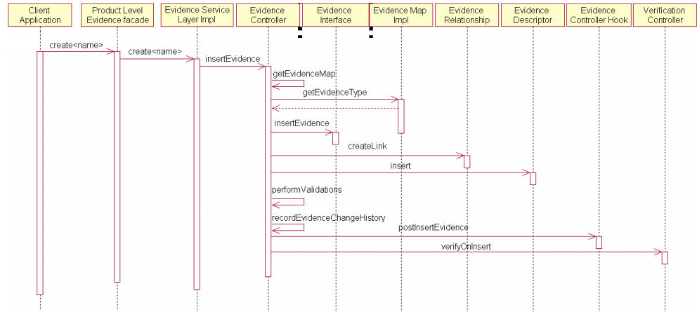
Figure 3.1 Sequence Diagram for Creating Evidence
