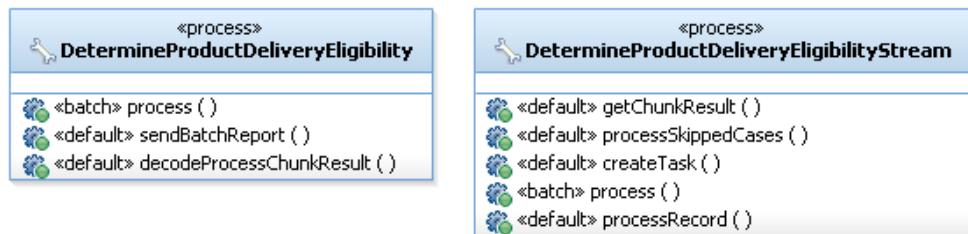
Figure 4.1 UML Model for Example Streamed Batch Program
