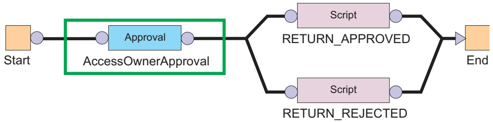
Figure 9. Sample workflow for access request
