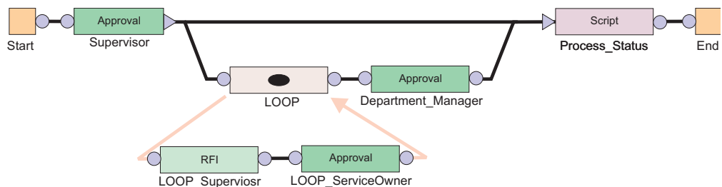
Figure 6. Sample workflow: multiple approvals with loop processing
