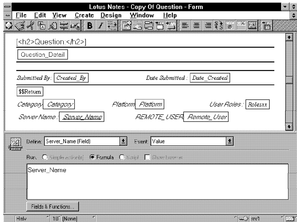
Figure 9. CGI Variables
