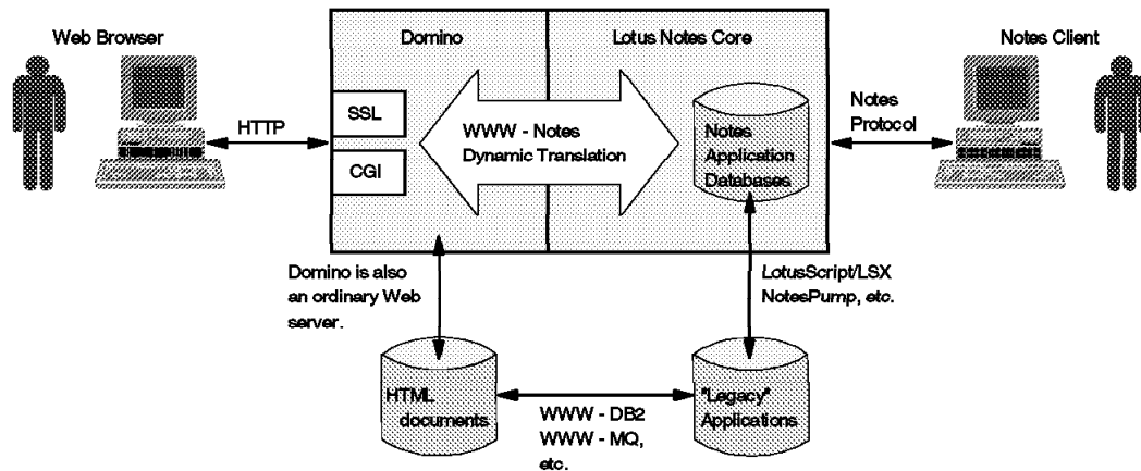
Figure 1. Domino Server
