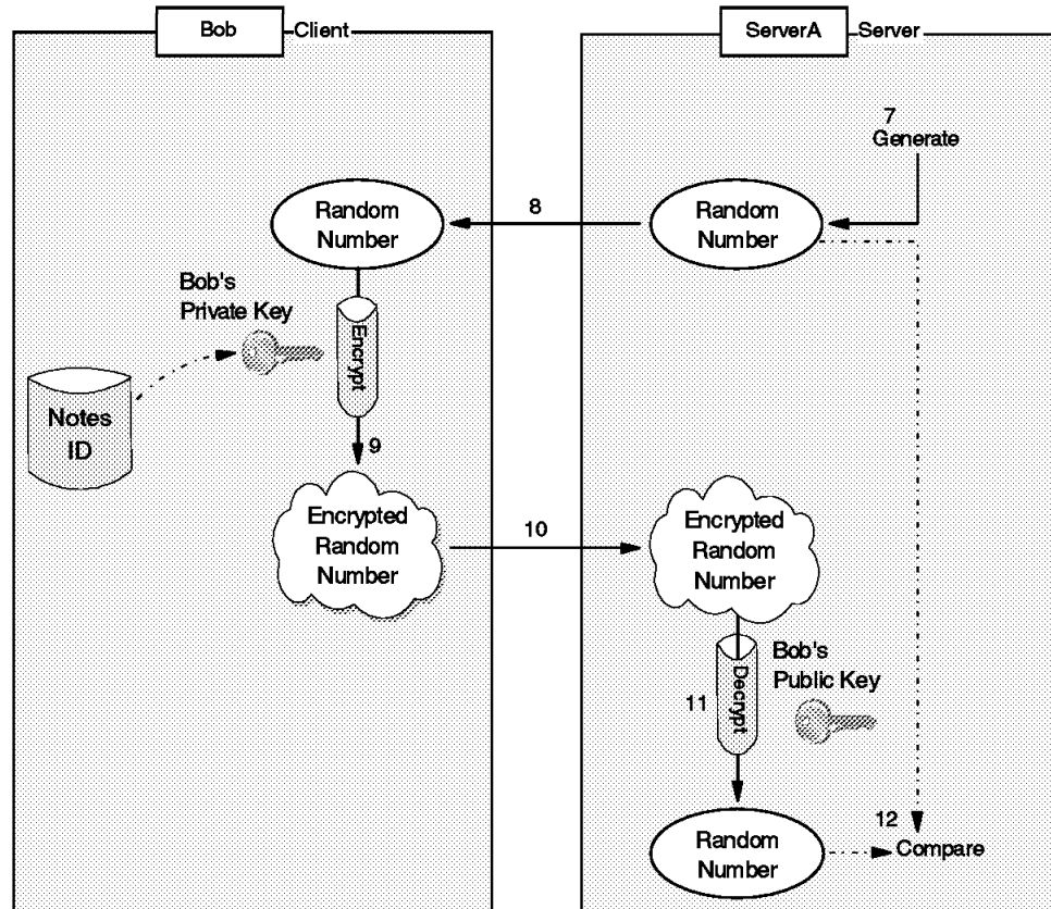
Figure 17. Authentication
