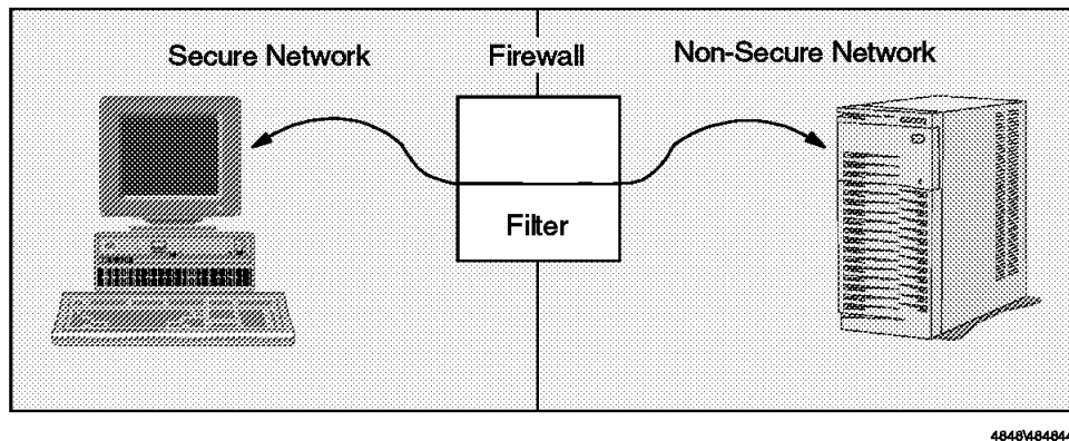
Figure 127. Filter Firewall
