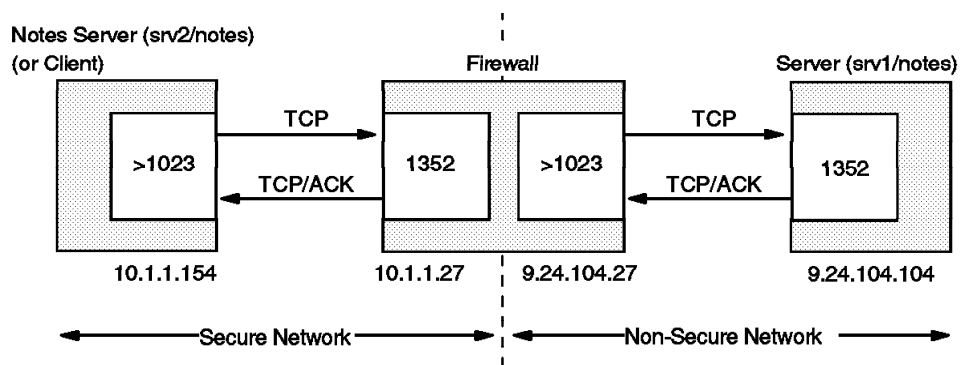
Figure 137. Filter Consideration on Our Proxy Firewall
