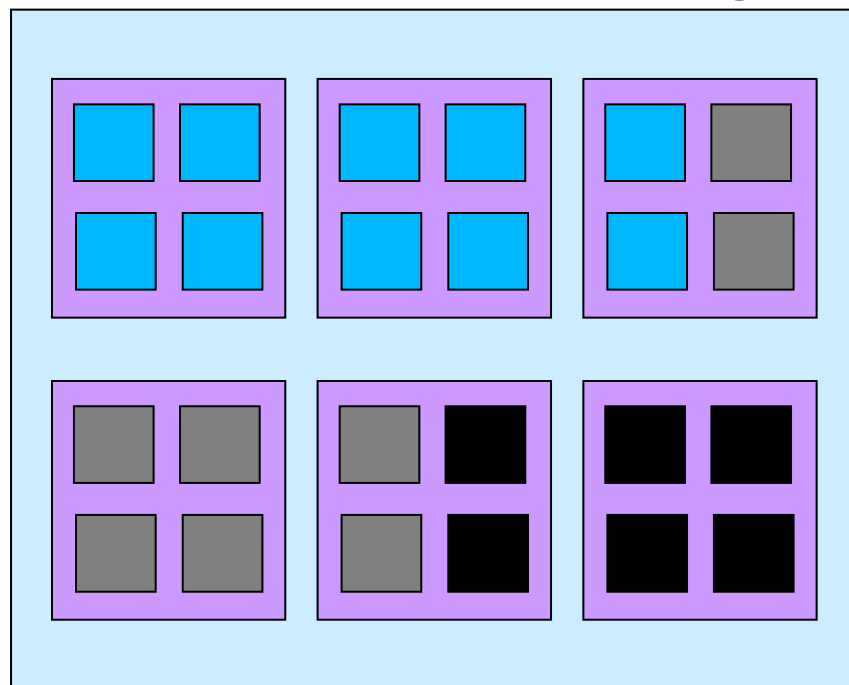
One z196 Book with 6 Processing Units
