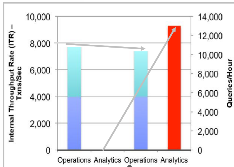
Data kept in sync real-time with minimal degradation in transaction ITR (3%)
