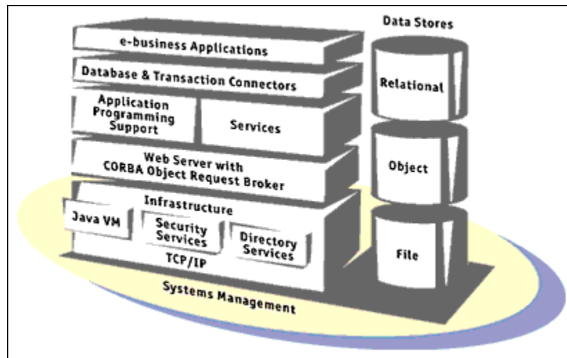
Figure 4: IBM Network Computing Framework (NCF) Structure
