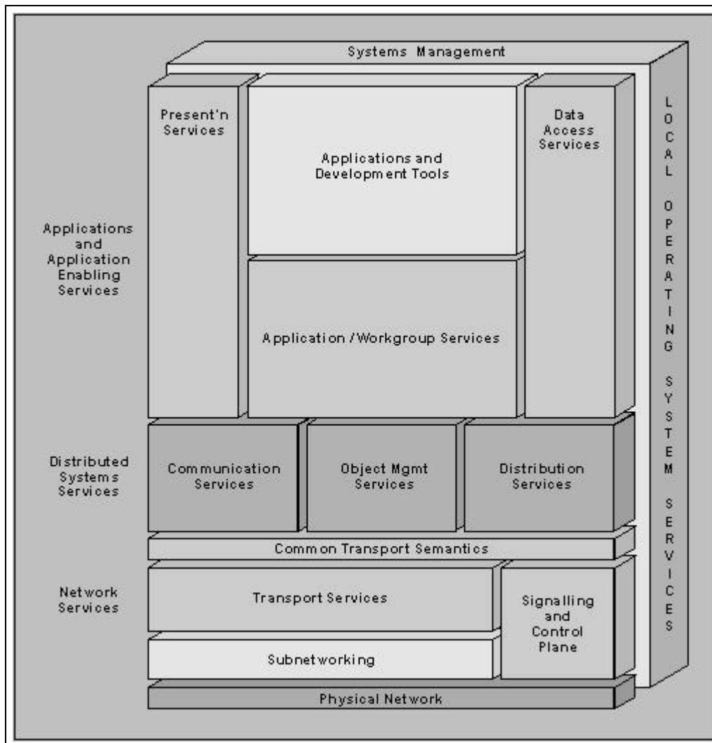
Figure 1: The Open Blueprint Structure
