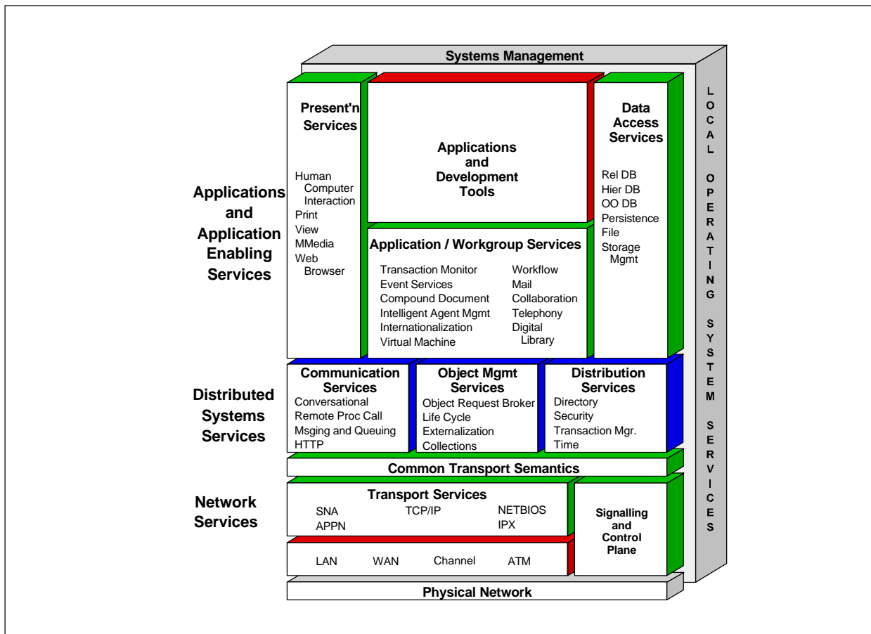
The Open Blueprint Structure
