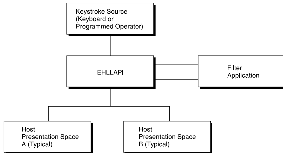
Figure 1. Keystroke Flow
