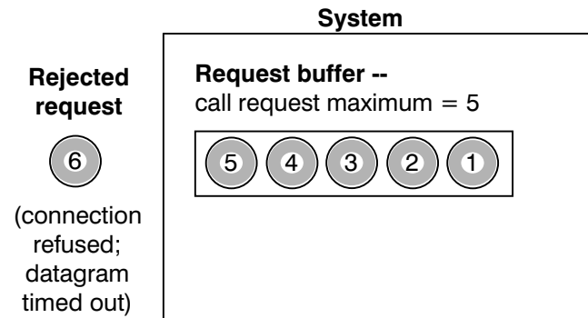
Figure 55. A Request Buffer at Full Capacity
