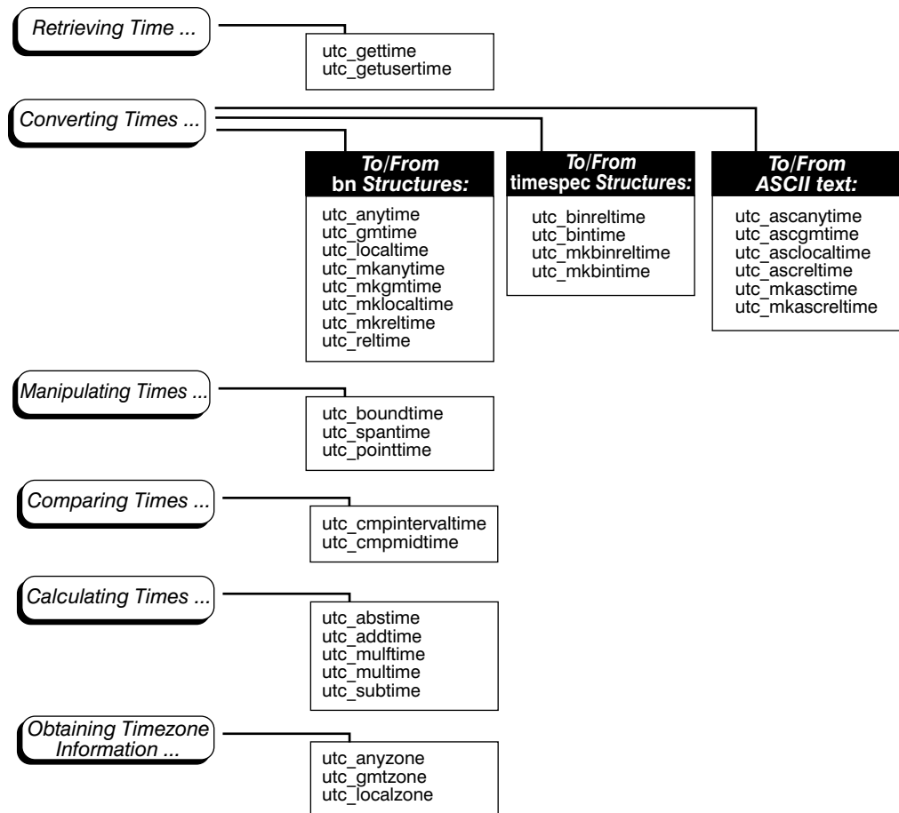
Figure 62. DTS API Routines Shown by Functional Grouping
