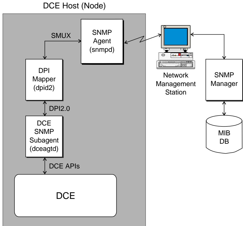
Figure 89. SNMP Network Management System component relationships
