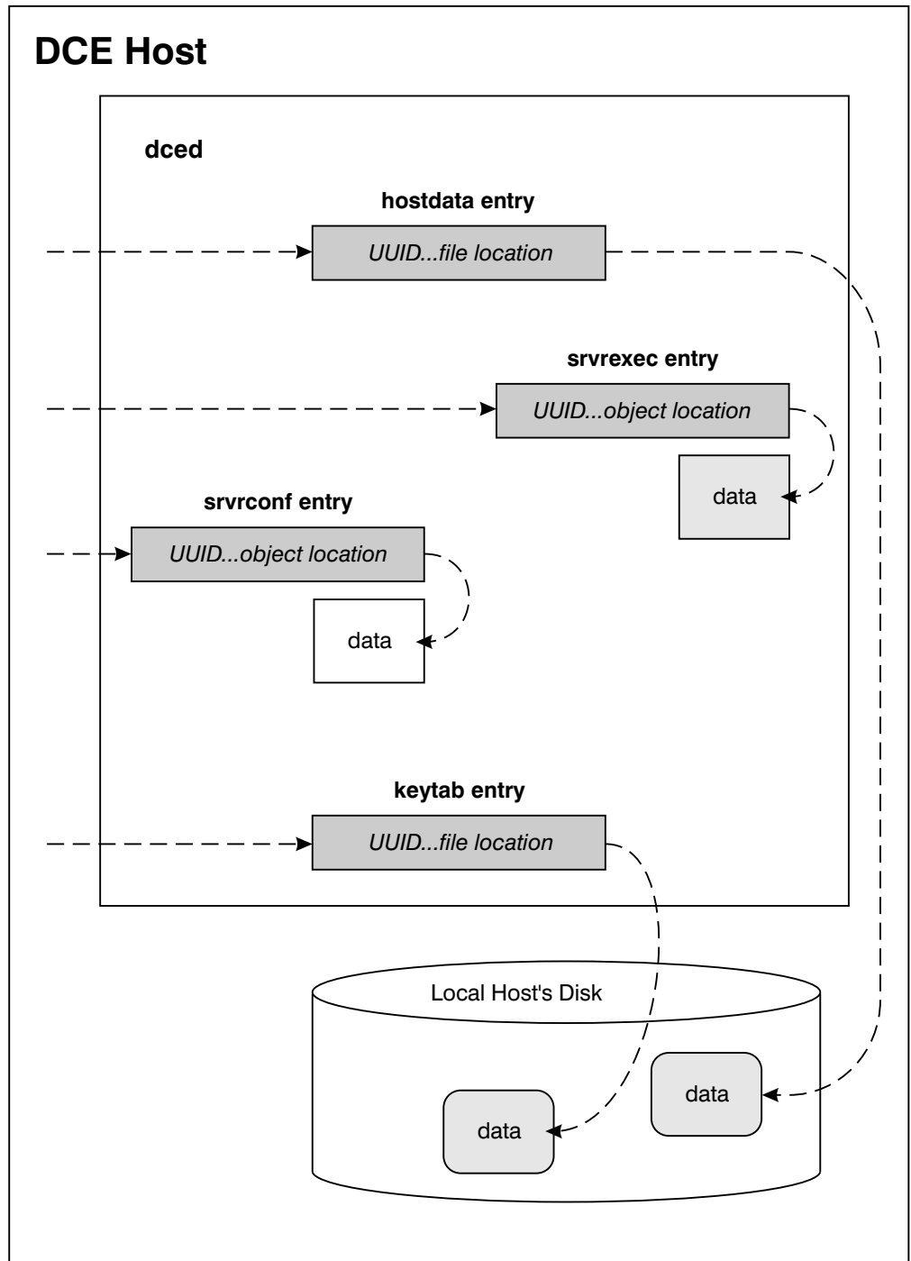
Figure 3. Accessing Hostdata
