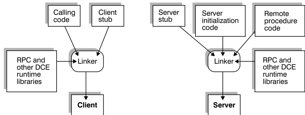
Figure 19. Building a Simple Client and Server
