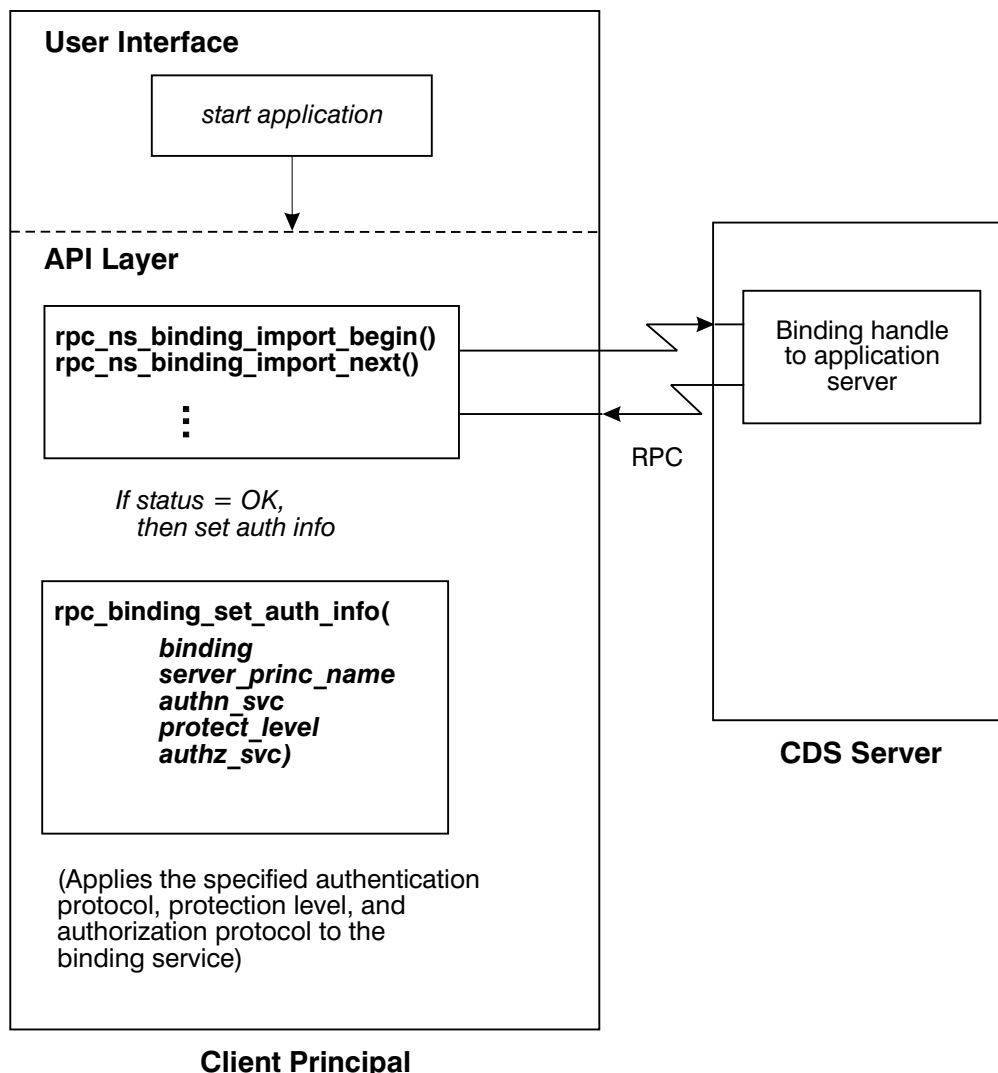
Figure 72. Client Sets Authentication and Authorization Information
