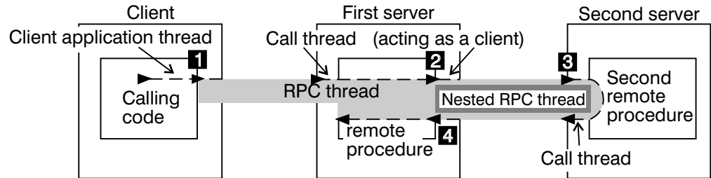
Figure 50. Phases of a Nested RPC Call
