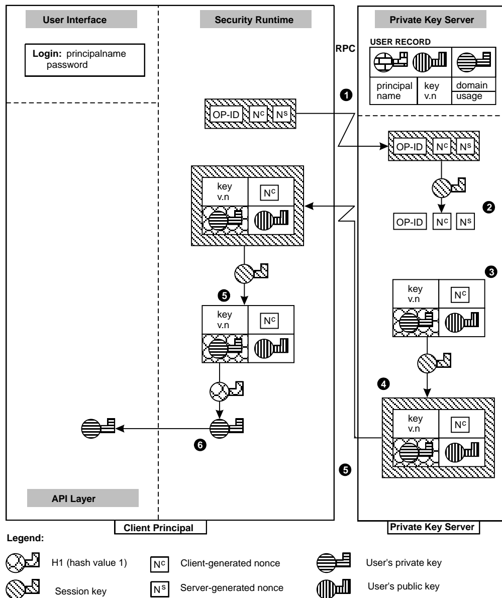
Figure 68. Client Acquisition of Private Key from PKSS
