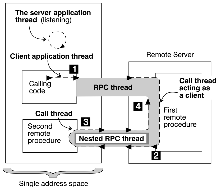
Figure 51. Phases of a Nested RPC Call to Client Address Space
