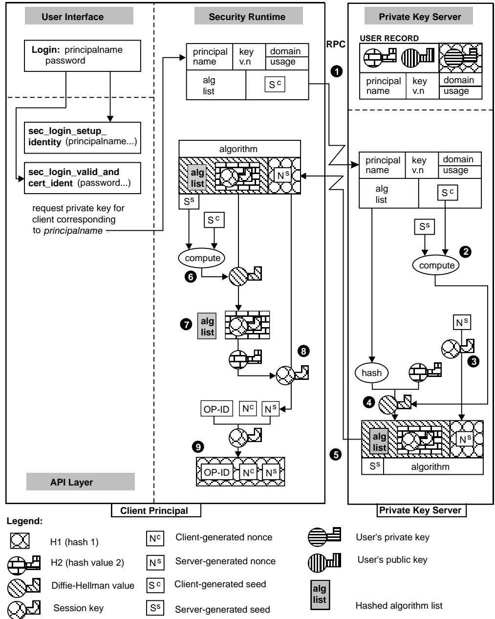
Figure 67. Client Initiation of Private Key Acquisition
