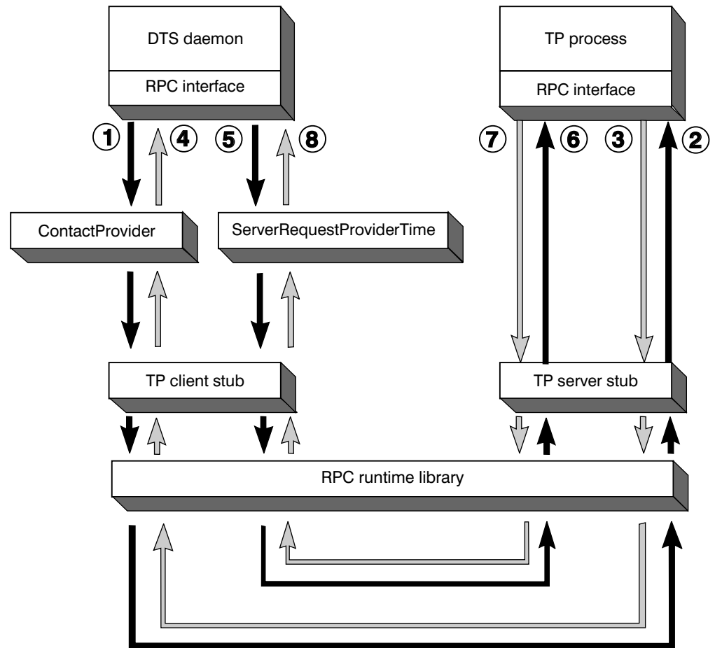
Figure 63. DTS/Time-Provider RPC Calling Sequence
