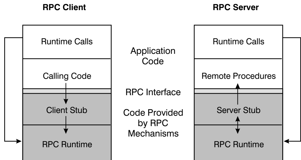
Figure 15. The Parts of an RPC Application
