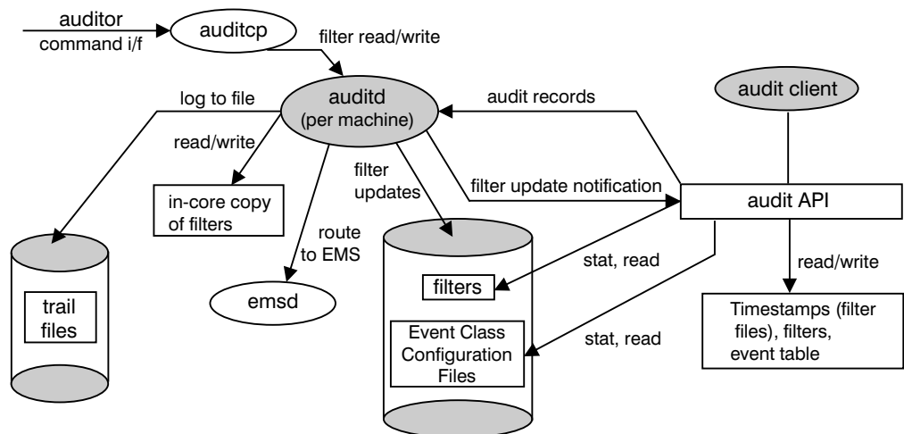
Figure 82. Overview of the DCE Audit Service
