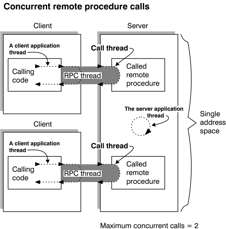
Figure 30. Concurrent Call Threads Executing in Shared Address Space
