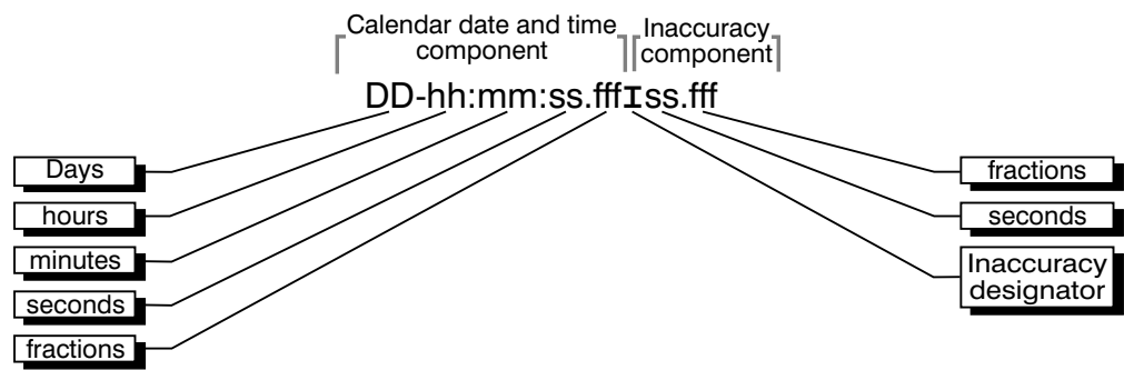
Figure 60. Full Syntax for a Relative Time
