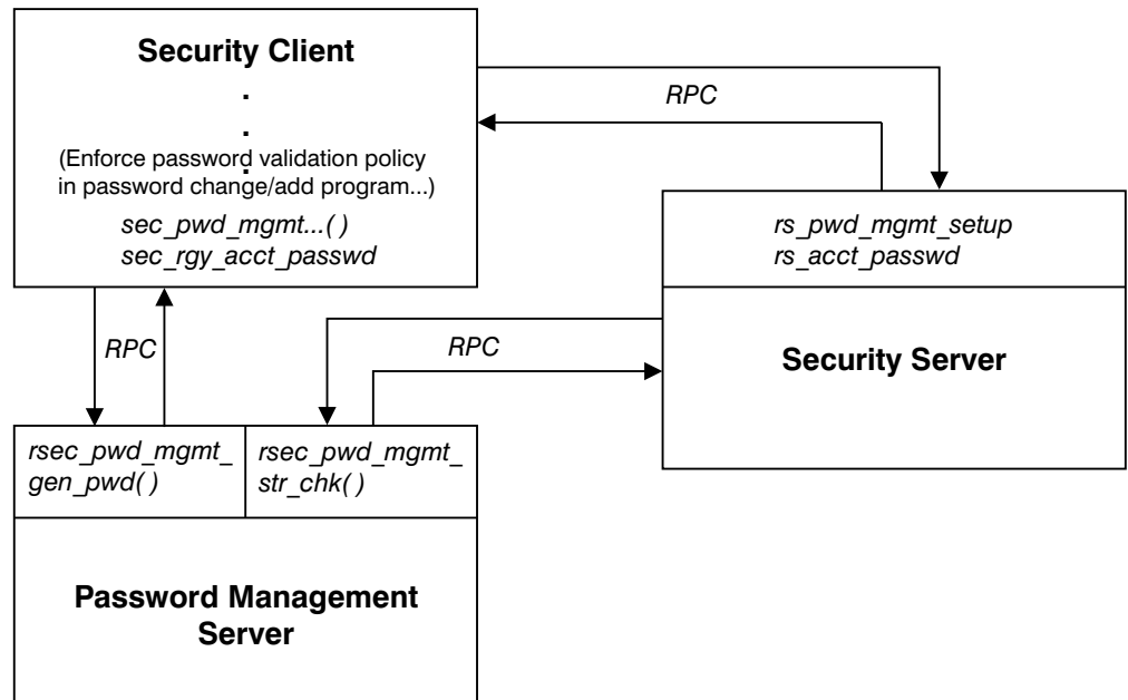
Figure 83. Use of Password Management Facility APIs
