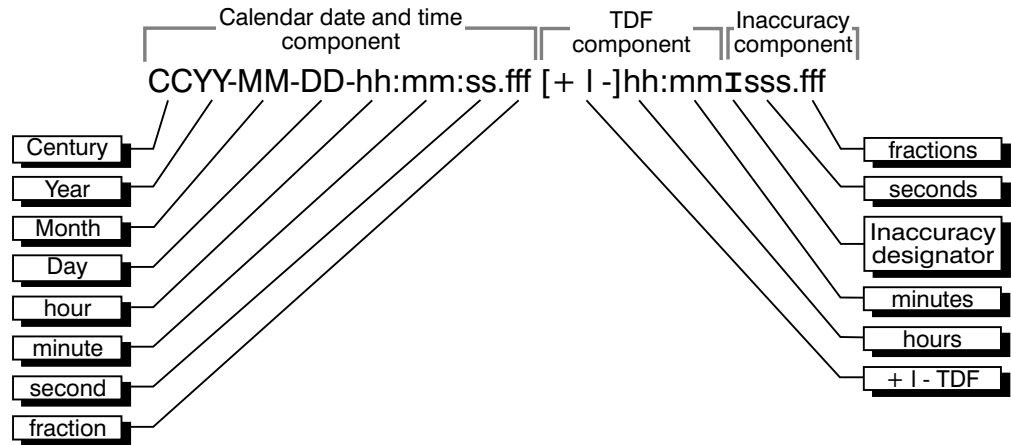
Figure 58. ISO Format for Time Displays
