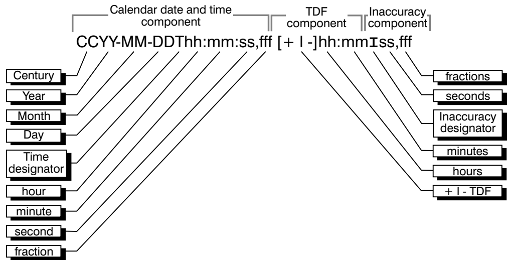
Figure 59. Variations to the ISO Time Format
