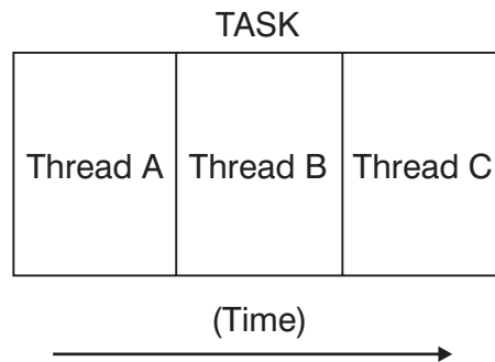
Figure 7. Pipelining Model
