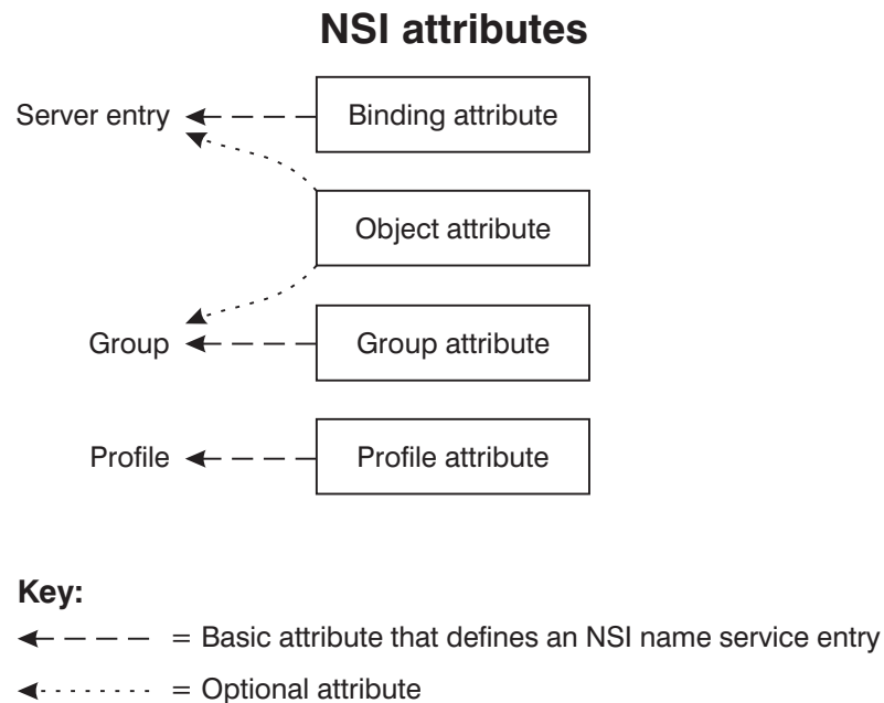
Figure 33. NSI Attributes
