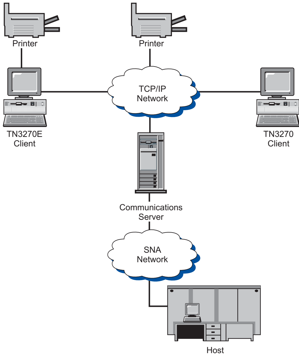
Figure 6. TN3270E Server Connections
