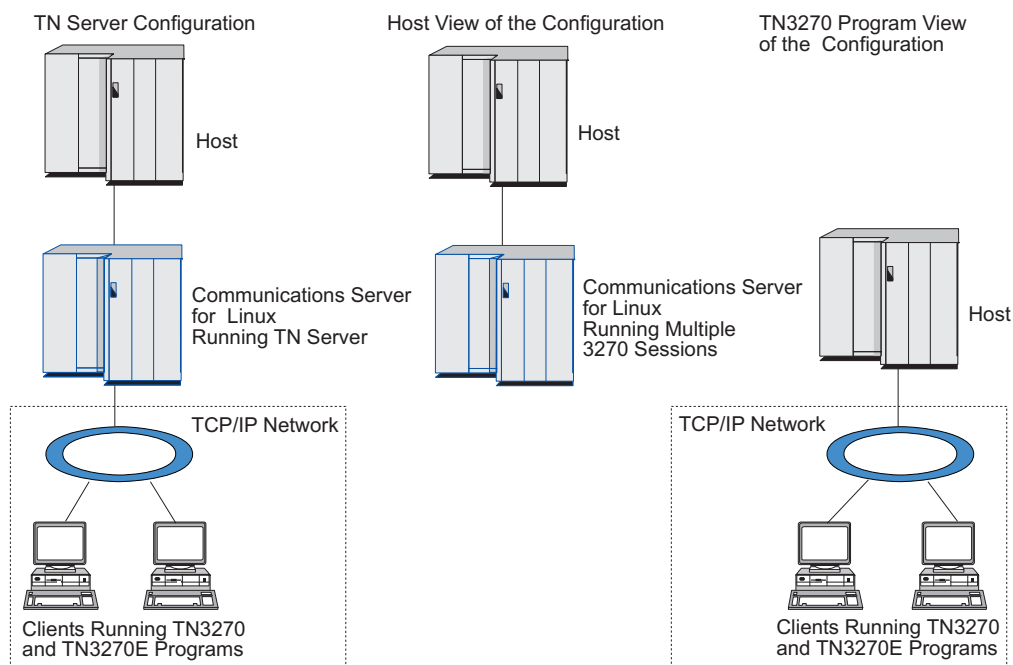
Figure 4. TN Server
