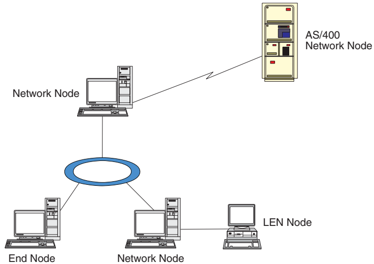
Figure 7. CS/AIX Nodes in an APPN Network
