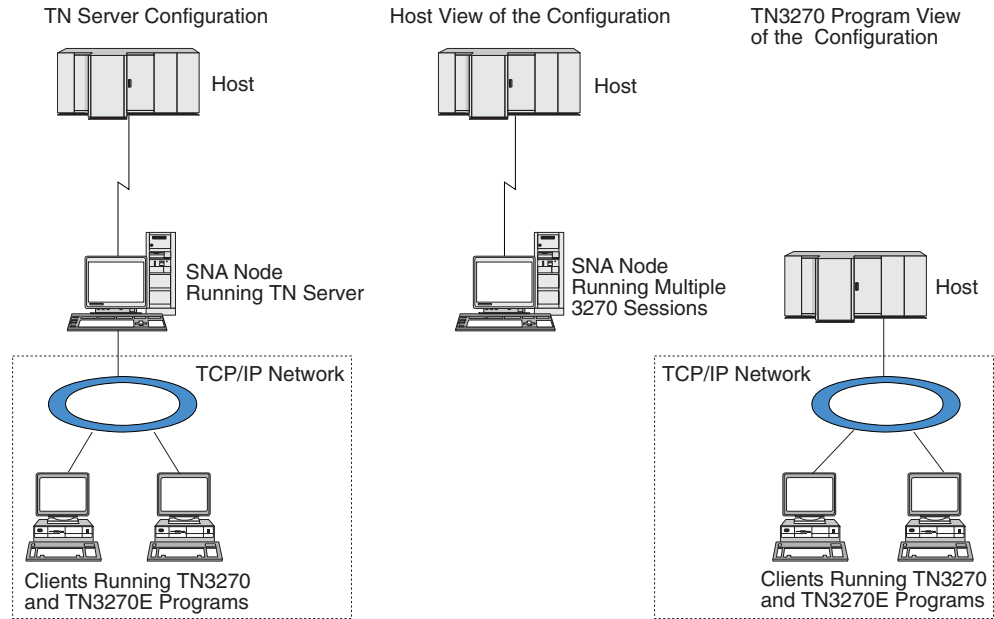
Figure 3. TN Server
