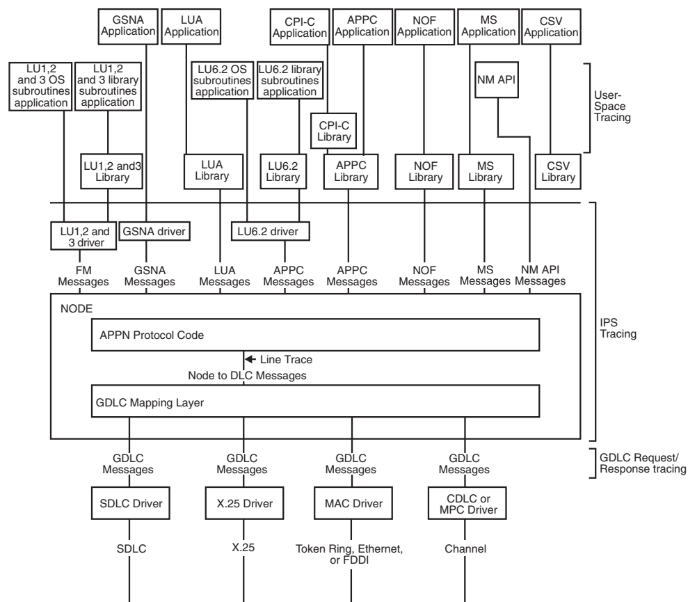
Figure 2. Overall Structure of CS/AIX
