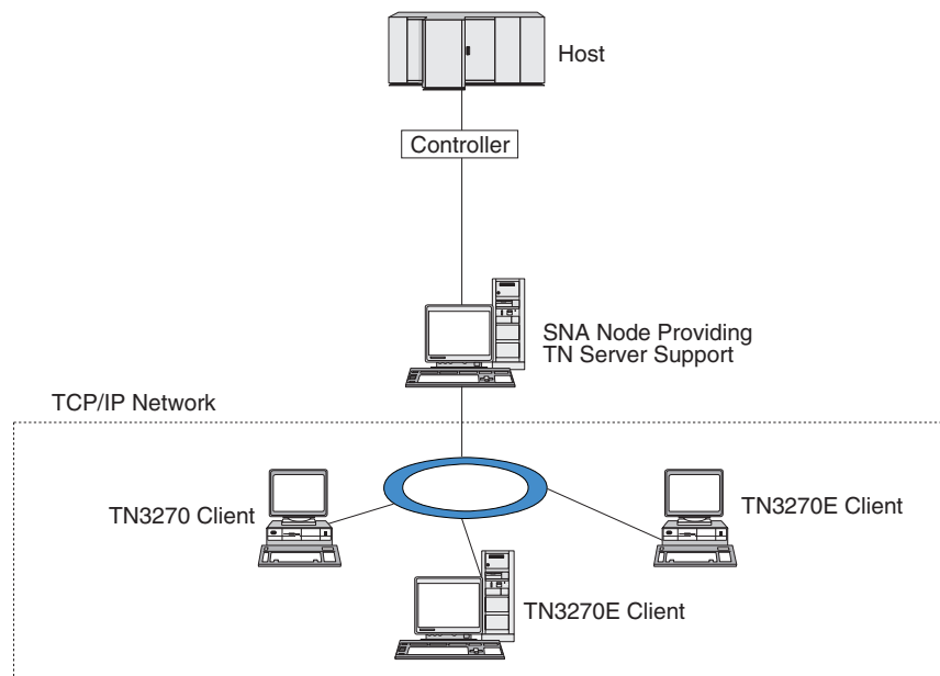
Figure 10. CS/AIX Node Configured for TN Server
