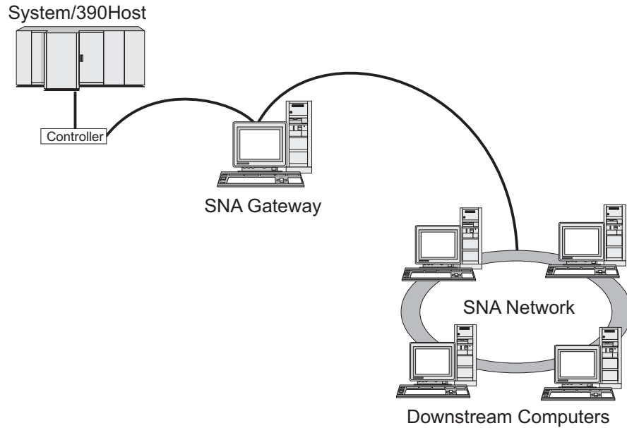
Figure 1. SNA Gateway Linking Multiple Downstream AIX Computers to a Host Computer
