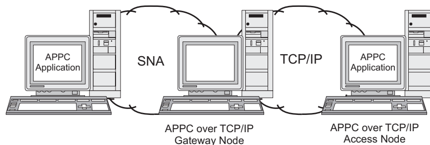
Figure 13. AnyNet APPC over TCP/IP Gateway
