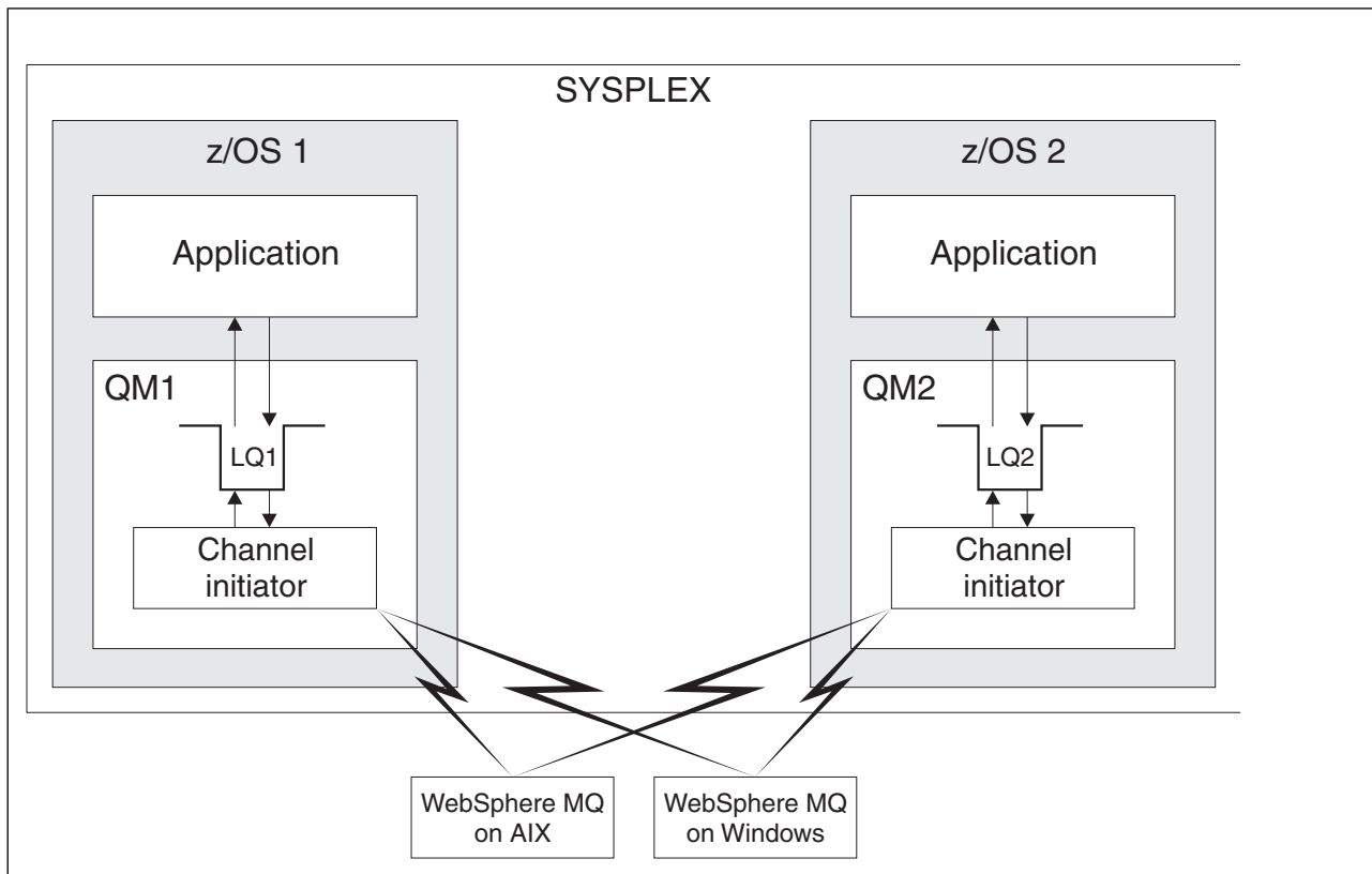
Figure 41. Communication between queue managers
