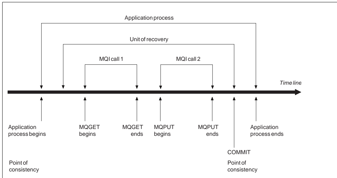
Figure 59. A unit of recovery within an application program. Typically, the unit of recovery consists of more than one MQI call. More than one unit of recovery can occur within an application program.
