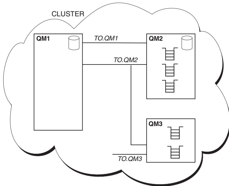
Figure 16. A cluster of queue managers
