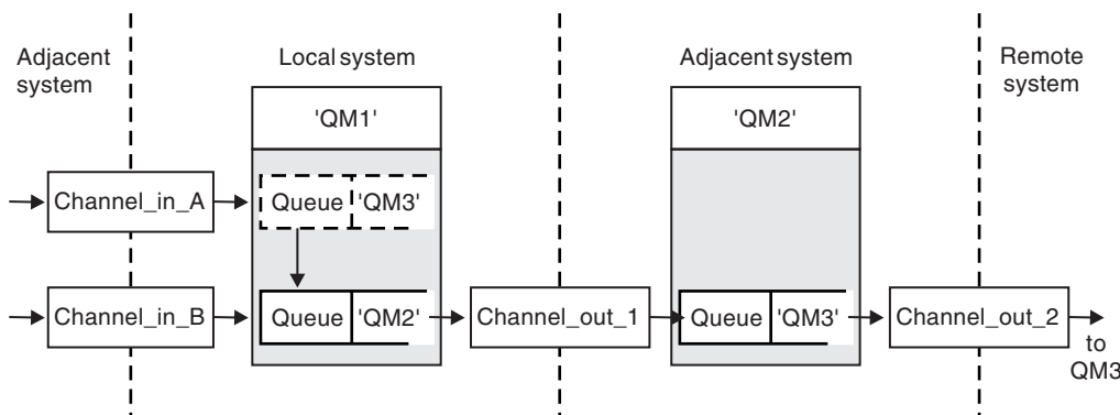
Figure 24. Queue manager alias
