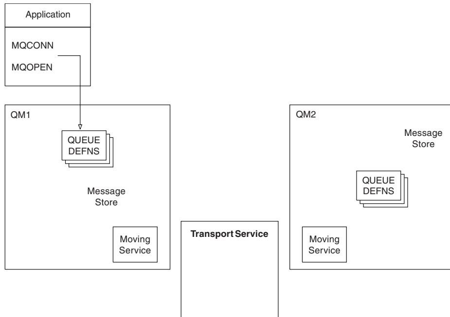
Figure 13. Overview of the components of distributed queuing
