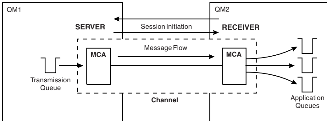
Figure 18. A requester-server channel
