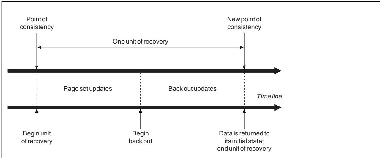
Figure 60. A unit of recovery showing back out
