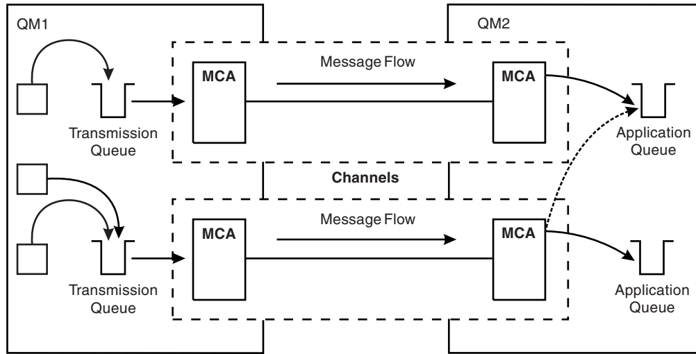
Figure 23. Using multiple channels
