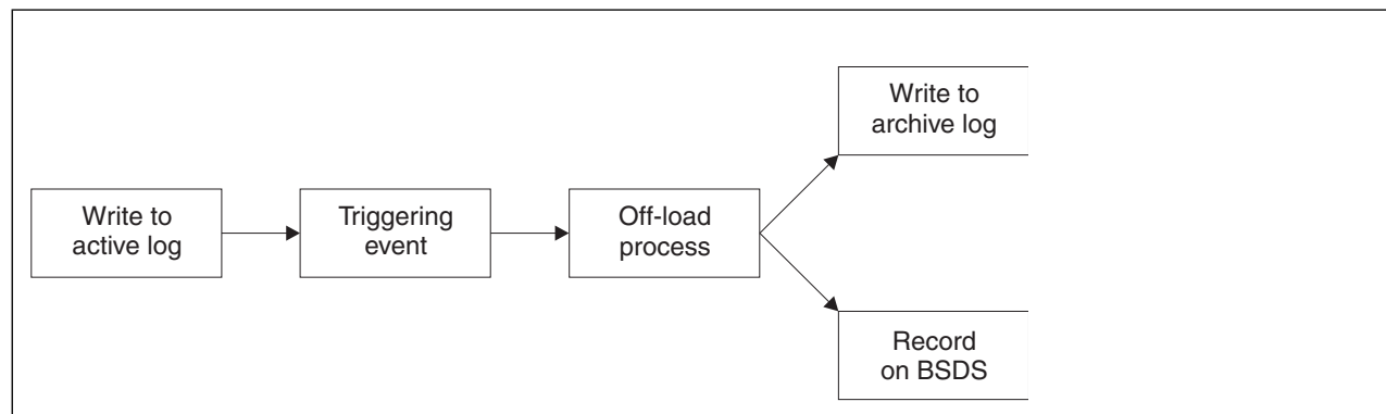
Figure 58. The offloading process
