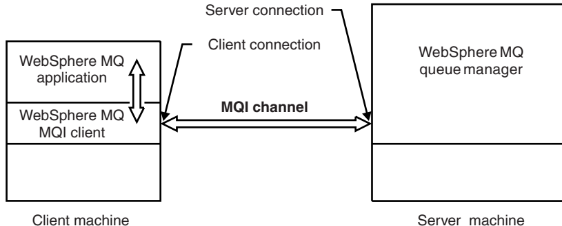
Figure 37. Client-connection and server-connection on an MQI channel
