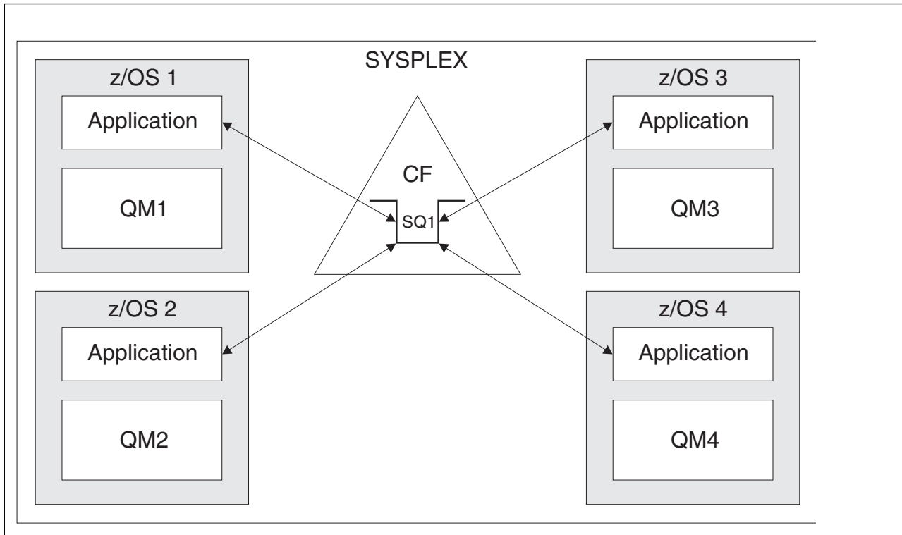
Figure 44. Multiple instances of an application servicing a shared queue
