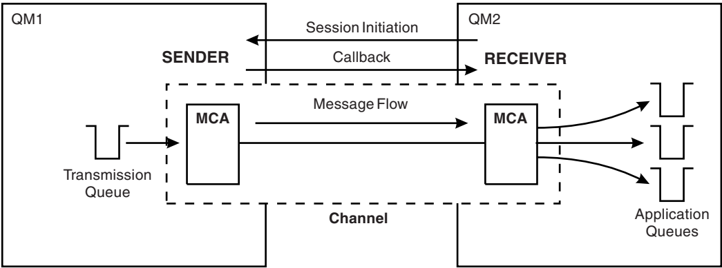
Figure 19. A requester-sender channel
