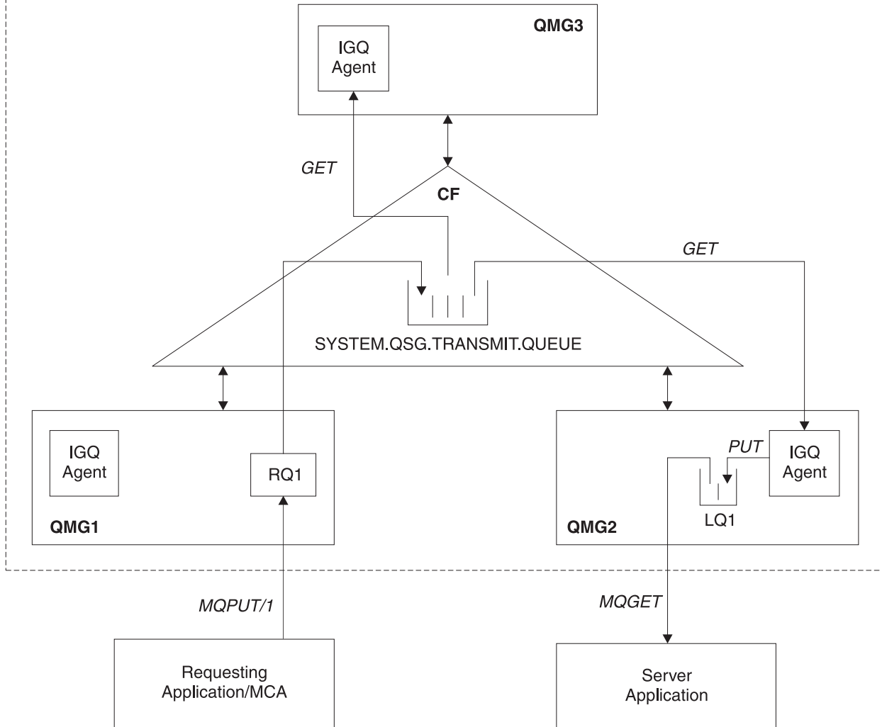
Figure 51. An example of intra-group queuing
