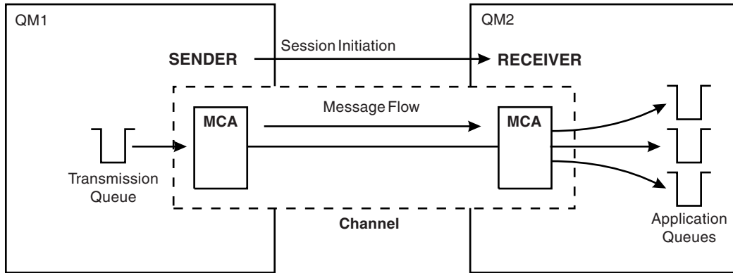
Figure 17. A sender-receiver channel
