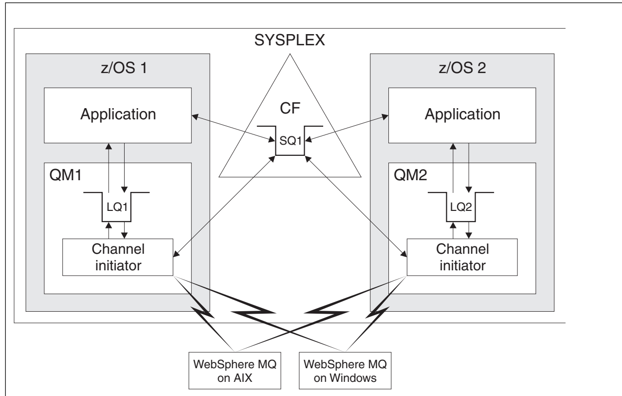
Figure 49. Distributed queuing and queue-sharing groups
