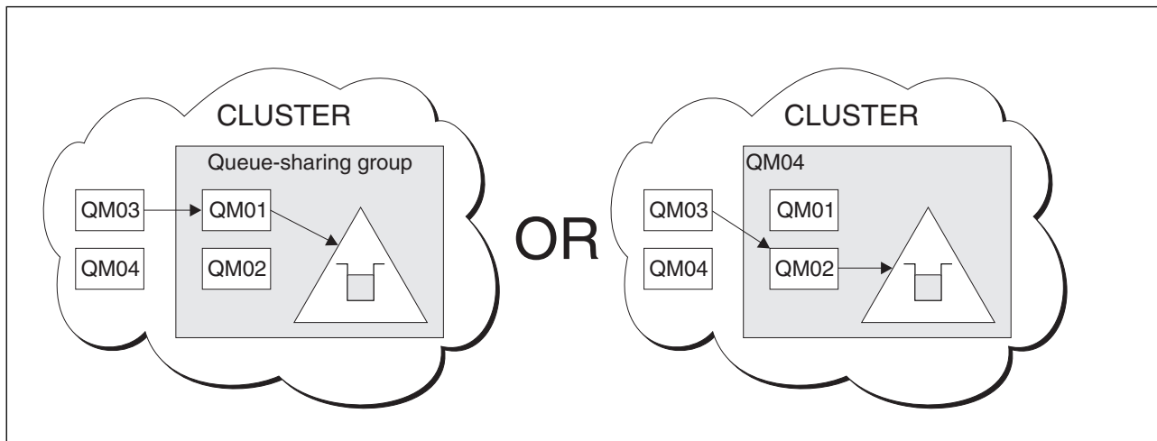
Figure 50. A queue-sharing group as part of a cluster
