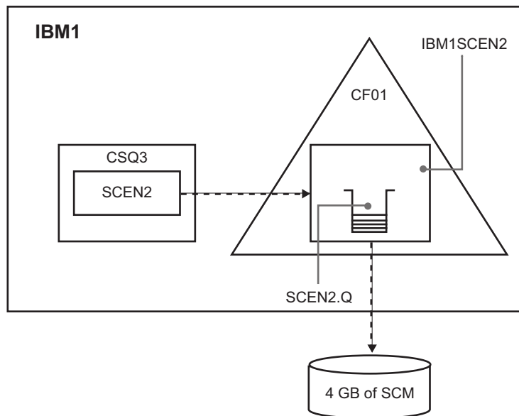
Figure 48. Configuration adding SCM for improved performance
