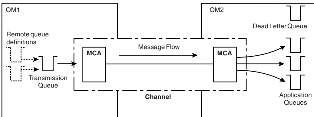
Figure 22. Sharing a transmission queue
