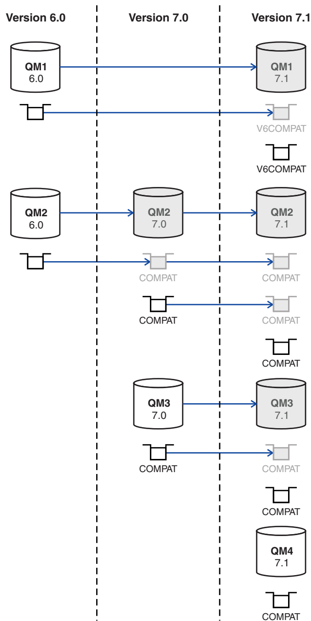
Figure 11. Migration and creation of queues with default PROPCTL attribute setting
