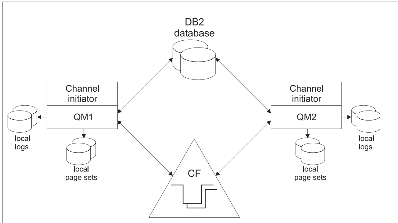
Figure 43. The components of queue managers in a queue-sharing group
