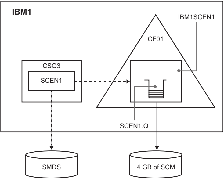
Figure 46. Configuration adding SMDS and SCM for emergency storage
