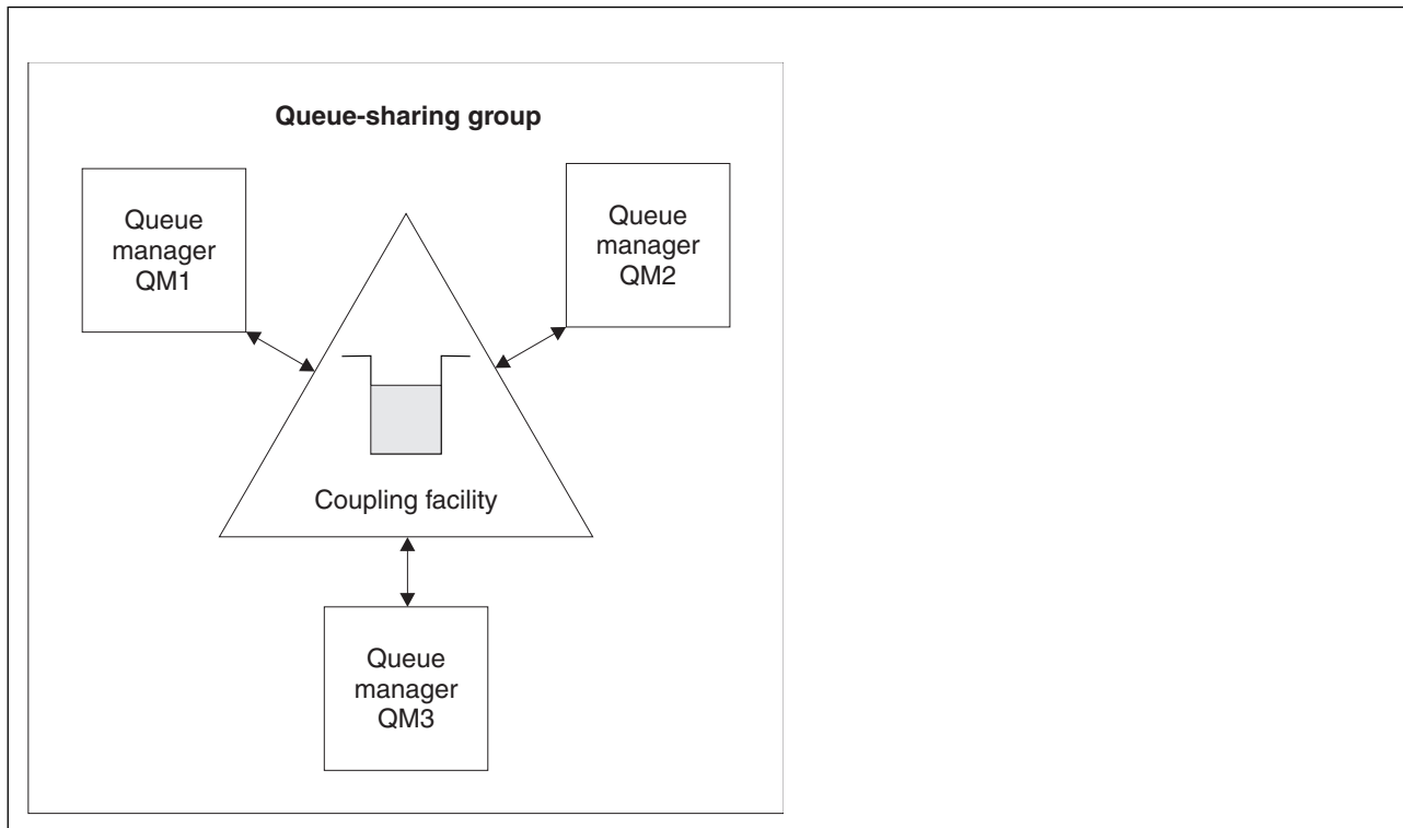
Figure 42. A queue-sharing group
