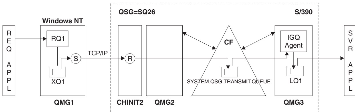
Figure 52. An example of migration support
