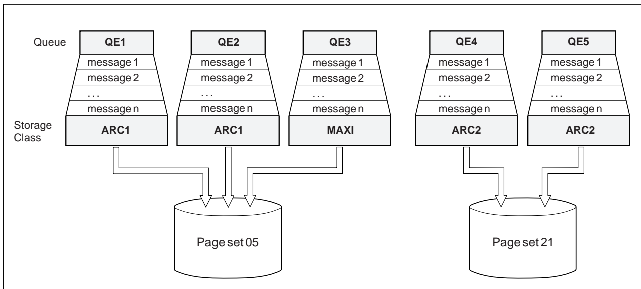
Figure 55. Mapping queues to page sets through storage classes
