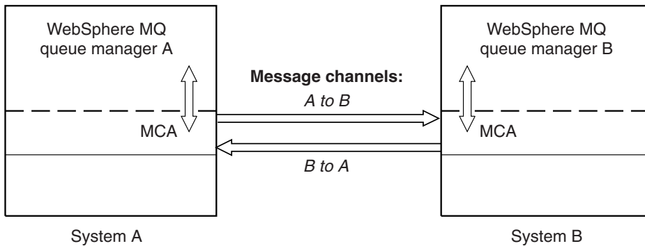
Figure 36. Message channels between two queue managers
