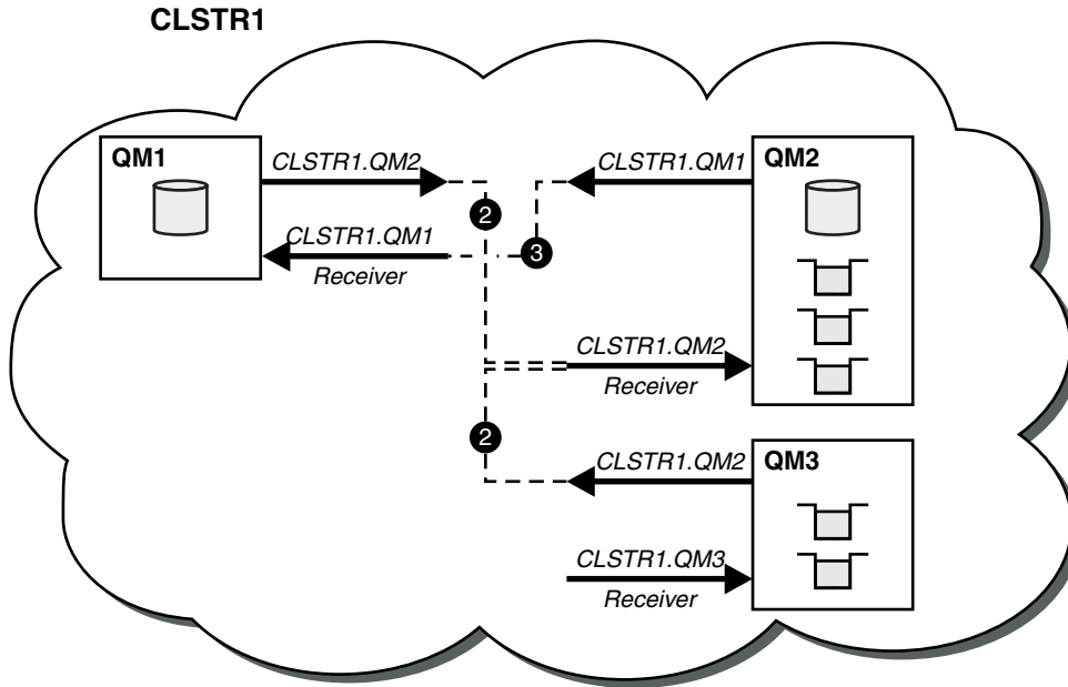
Figure 27. A cluster of queue managers with sender channels
