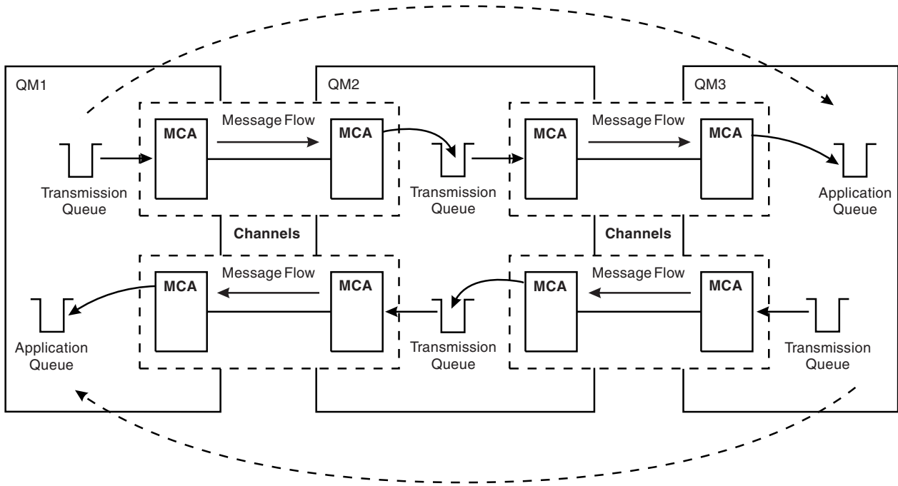
Figure 21. Passing through intermediate queue managers
