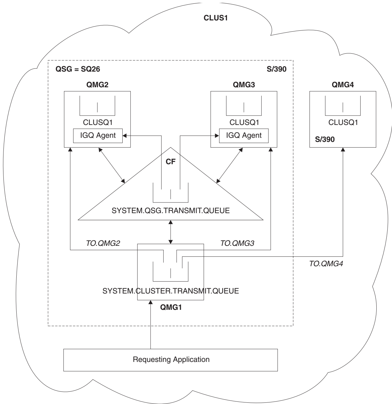
Figure 54. An example of clustering with intra-group queuing
