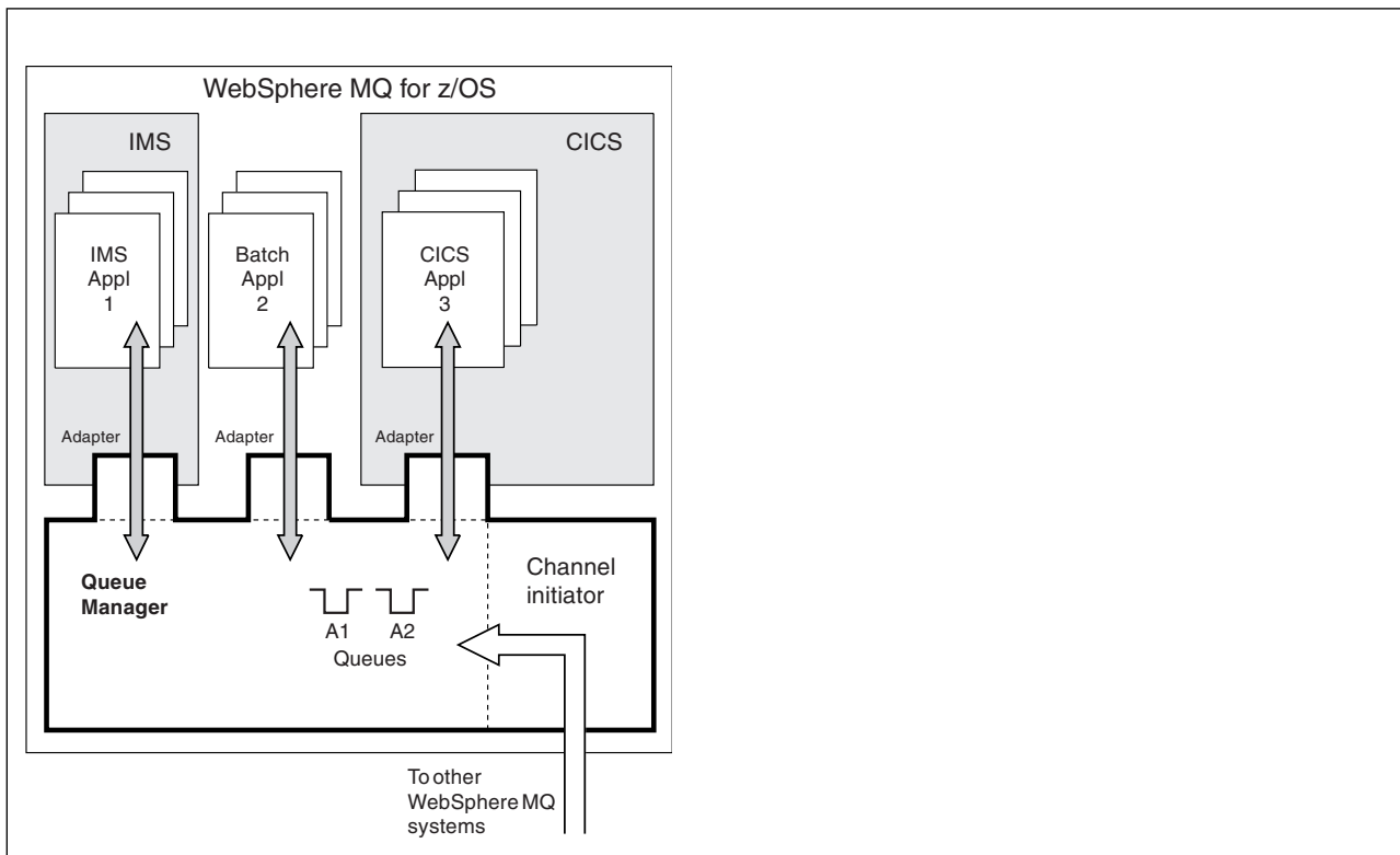
Figure 40. Overview of WebSphere MQ for z/OS
