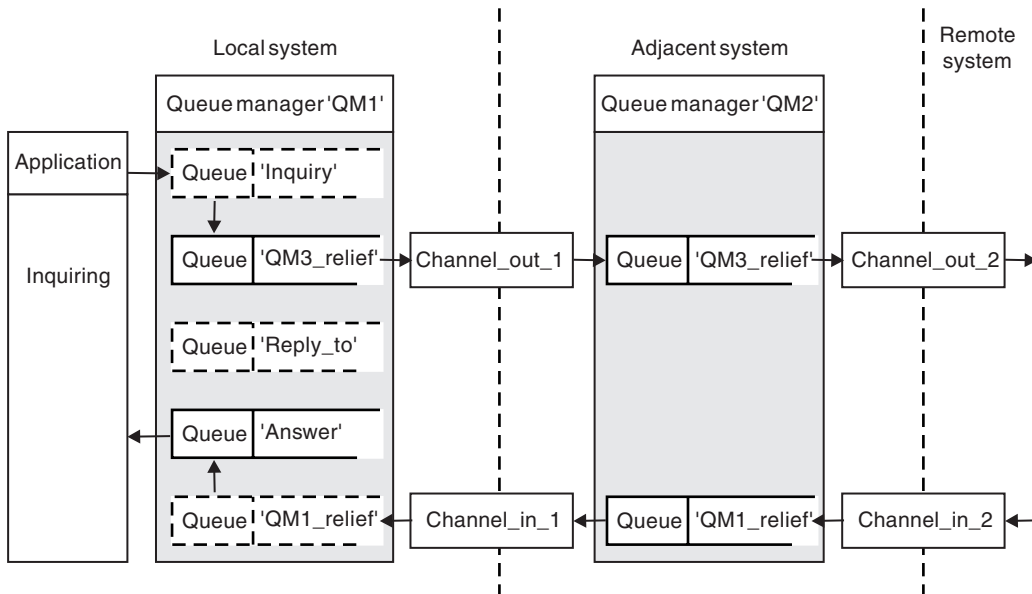
Figure 25. Reply-to queue alias used for changing reply location
