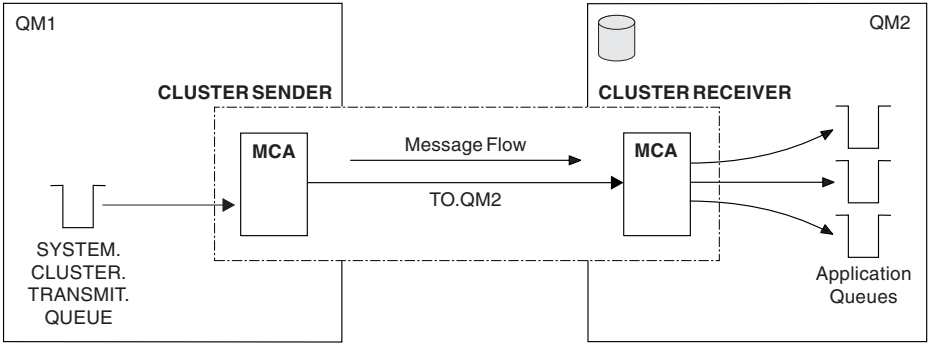
Figure 20. A cluster-sender channel
