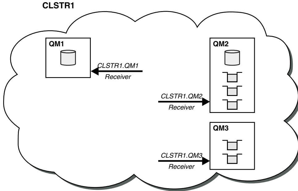
Figure 26. A cluster of queue managers
