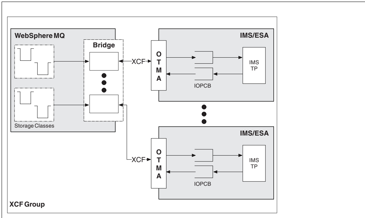
Figure 62. The WebSphere MQ-IMS bridge
