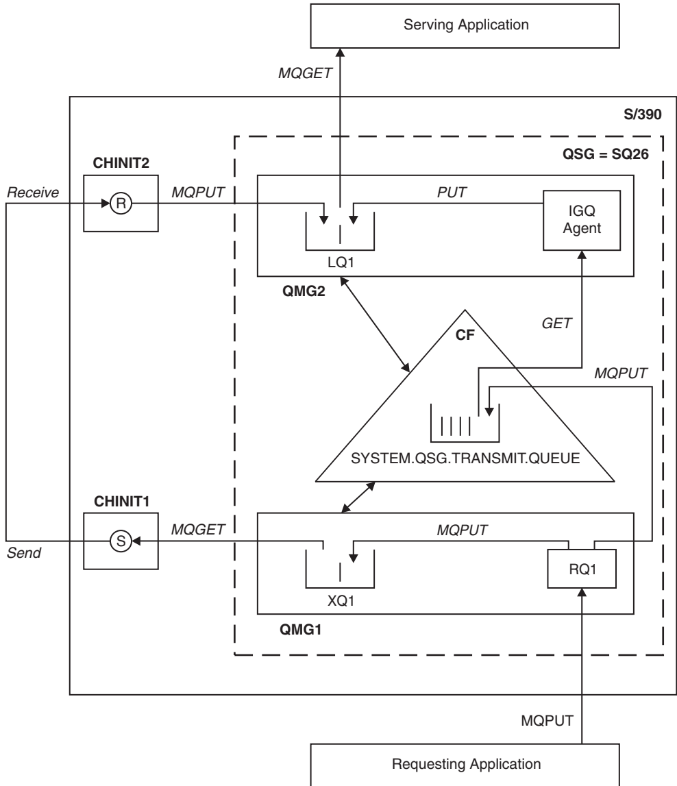
Figure 53. An example configuration
