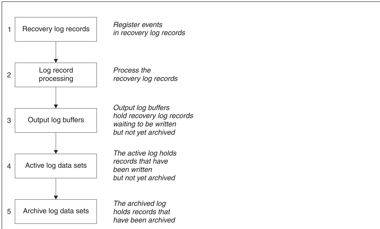
Figure 57. The logging process
