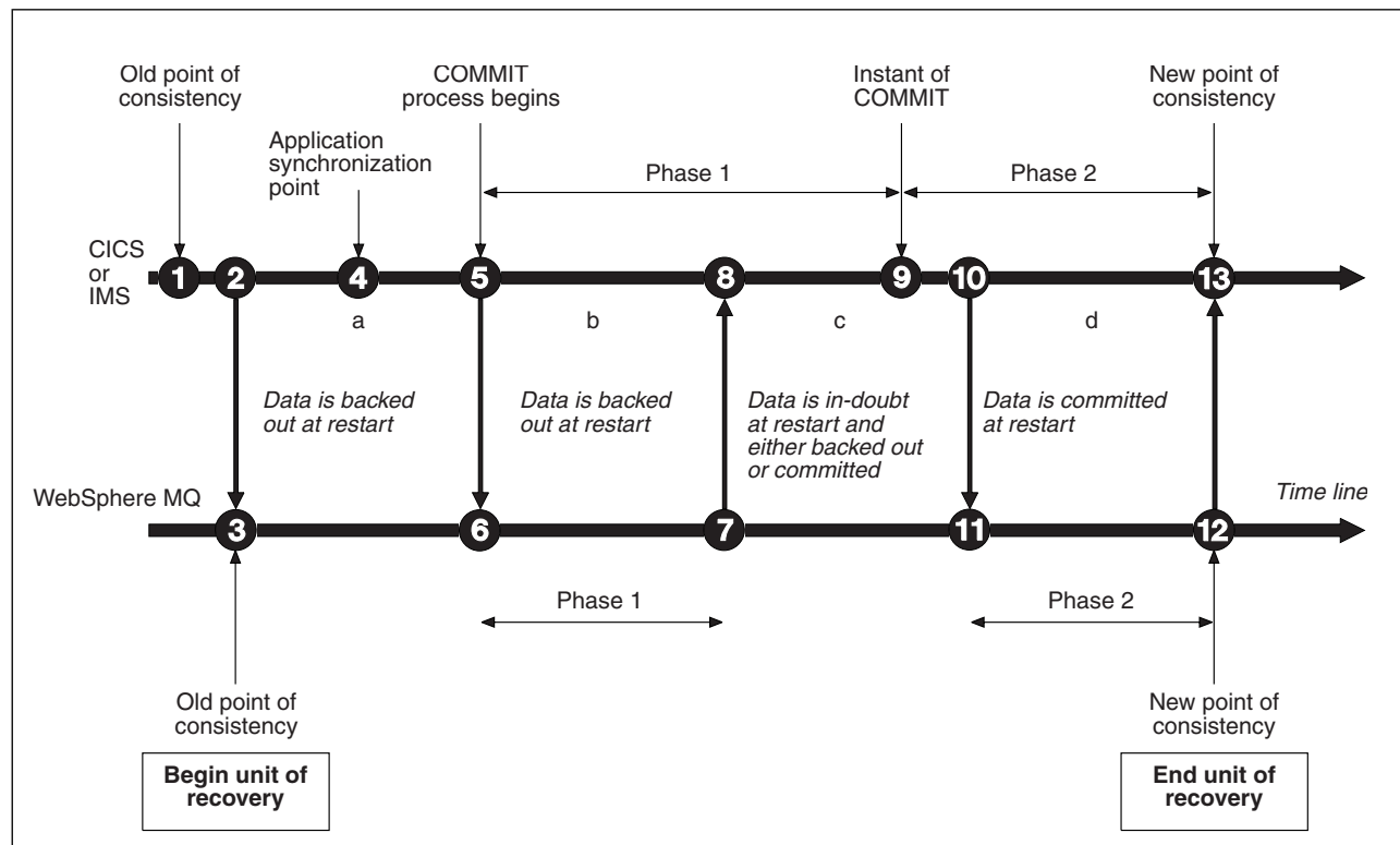
Figure 61. The two-phase commit process
