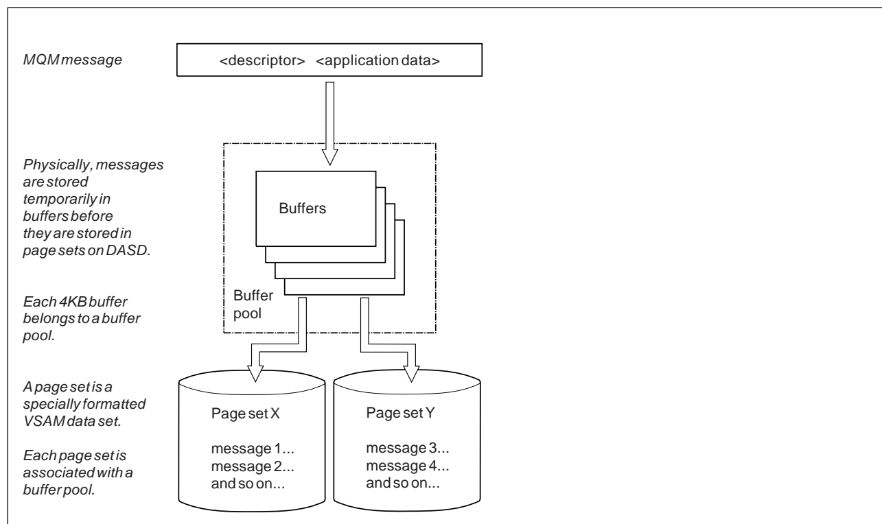
Figure 56. Buffers, buffer pools, and page sets
