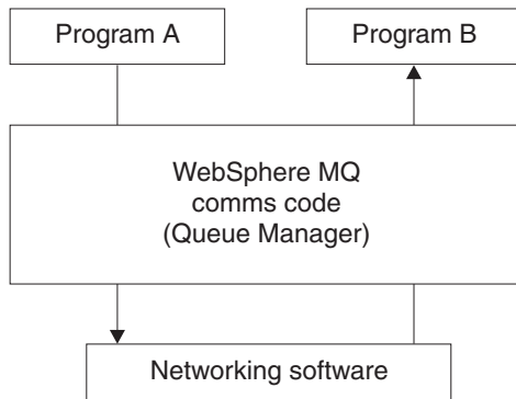
Figure 12. Message queuing compared with traditional communication
