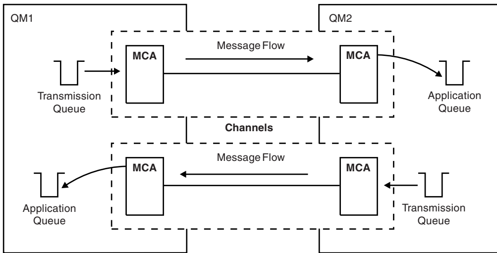
Figure 15. Sending messages in both directions
