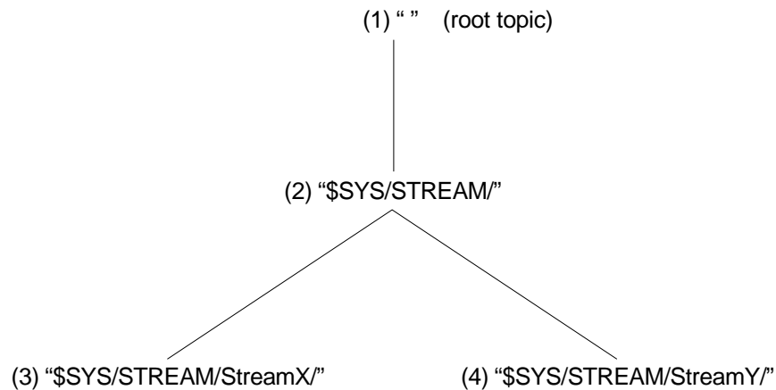
Figure 21. Stream authorities
