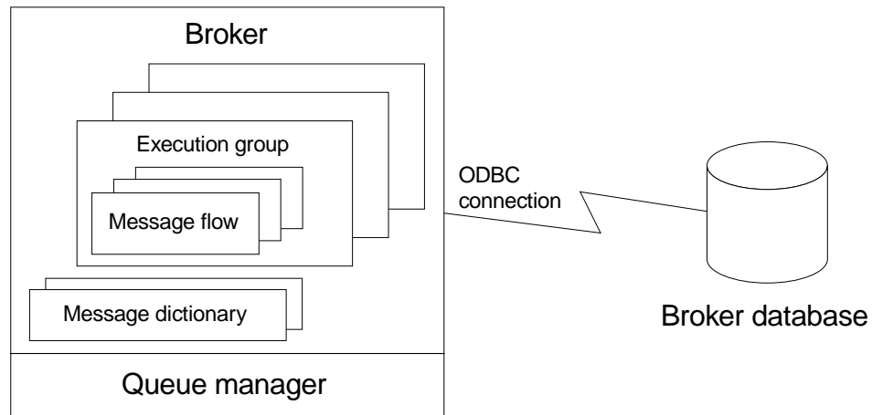
Figure 2. The broker
