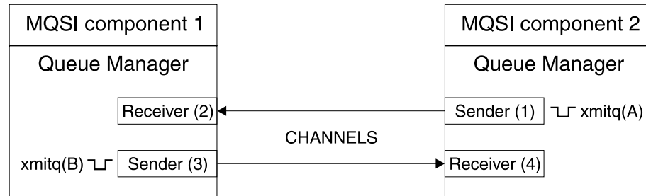
Figure 1. Connecting two MQSeries Integrator components
