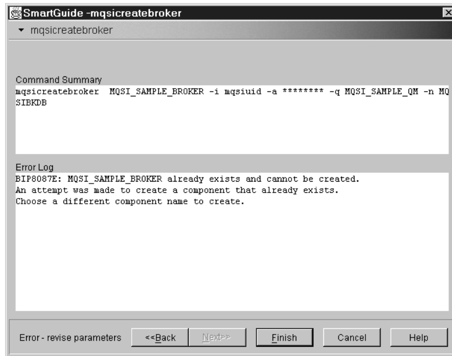
Figure 13. Create broker.: error response
