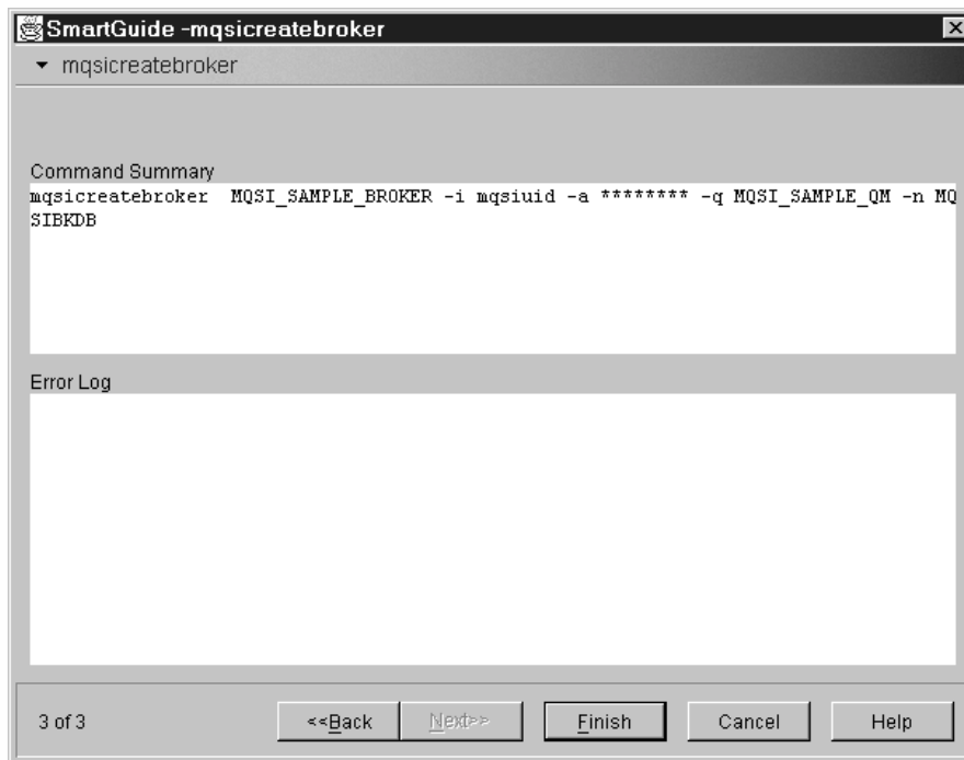
Figure 8. Create broker: screen 3
