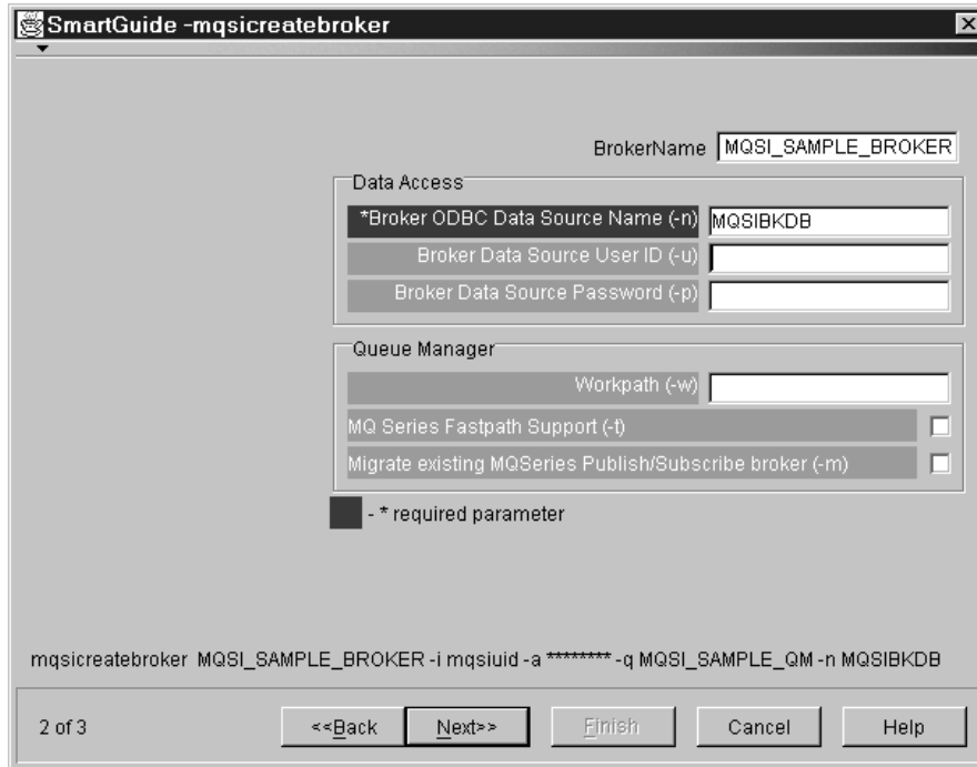
Figure 7. Create broker: screen 2
