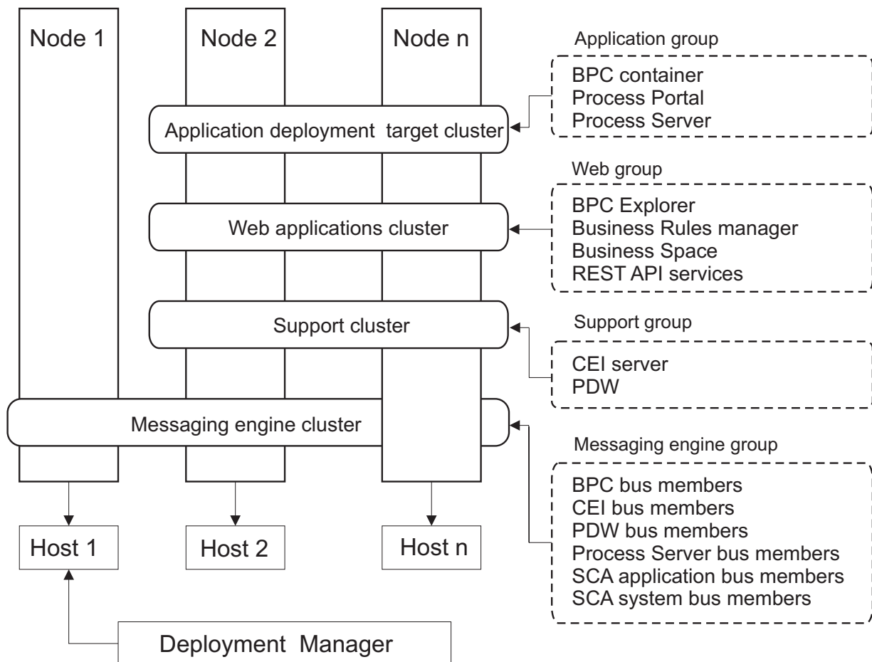
Figure 7. Remote Messaging, Remote Support, and Web topology pattern
