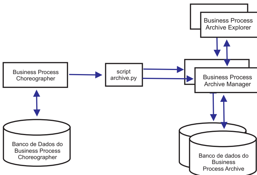
Figura 9. Business Process Choreographer usando dois Business Process Archives
