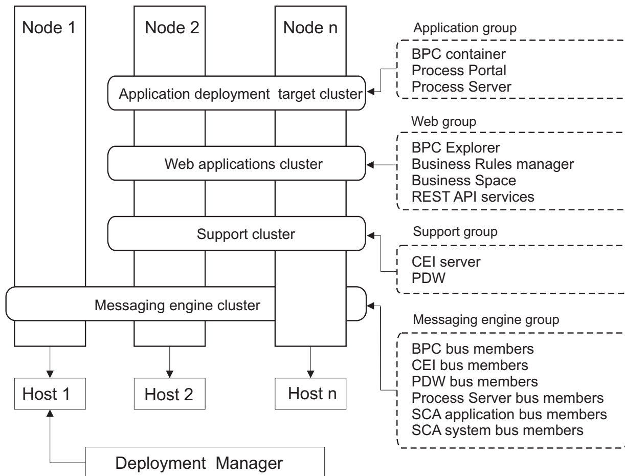
Figure 7. Remote Messaging, Remote Support, and Web topology pattern
