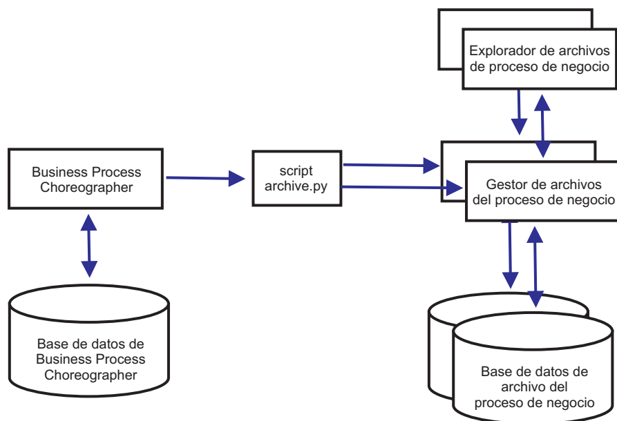
Figura 12. Business Process Choreographer con dos Business Process Archive
