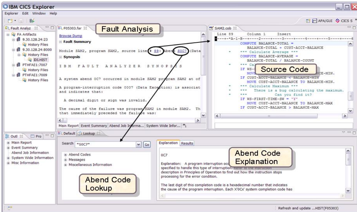
Figure 4: Fault Analyzer GUI Plug-in with CICS Explorer
