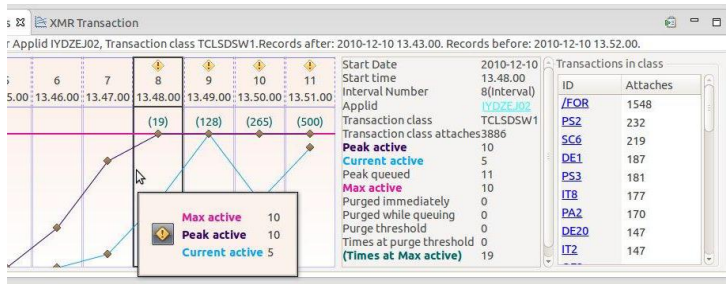
Figure 2 CICS Performance Analyzer statistics alert visualization
