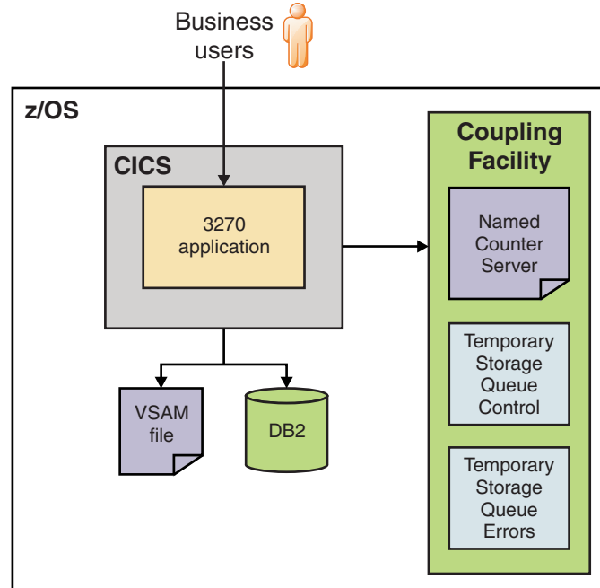
Figure 1. Initial CICS application configuration
