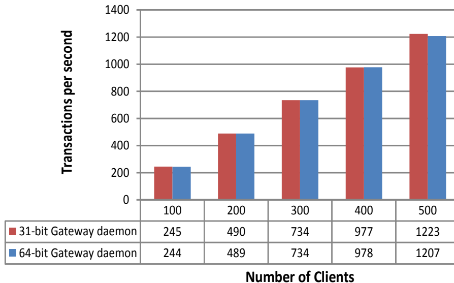
Illustration 5: "IPIC scaling clients TPS with 4K payload"
