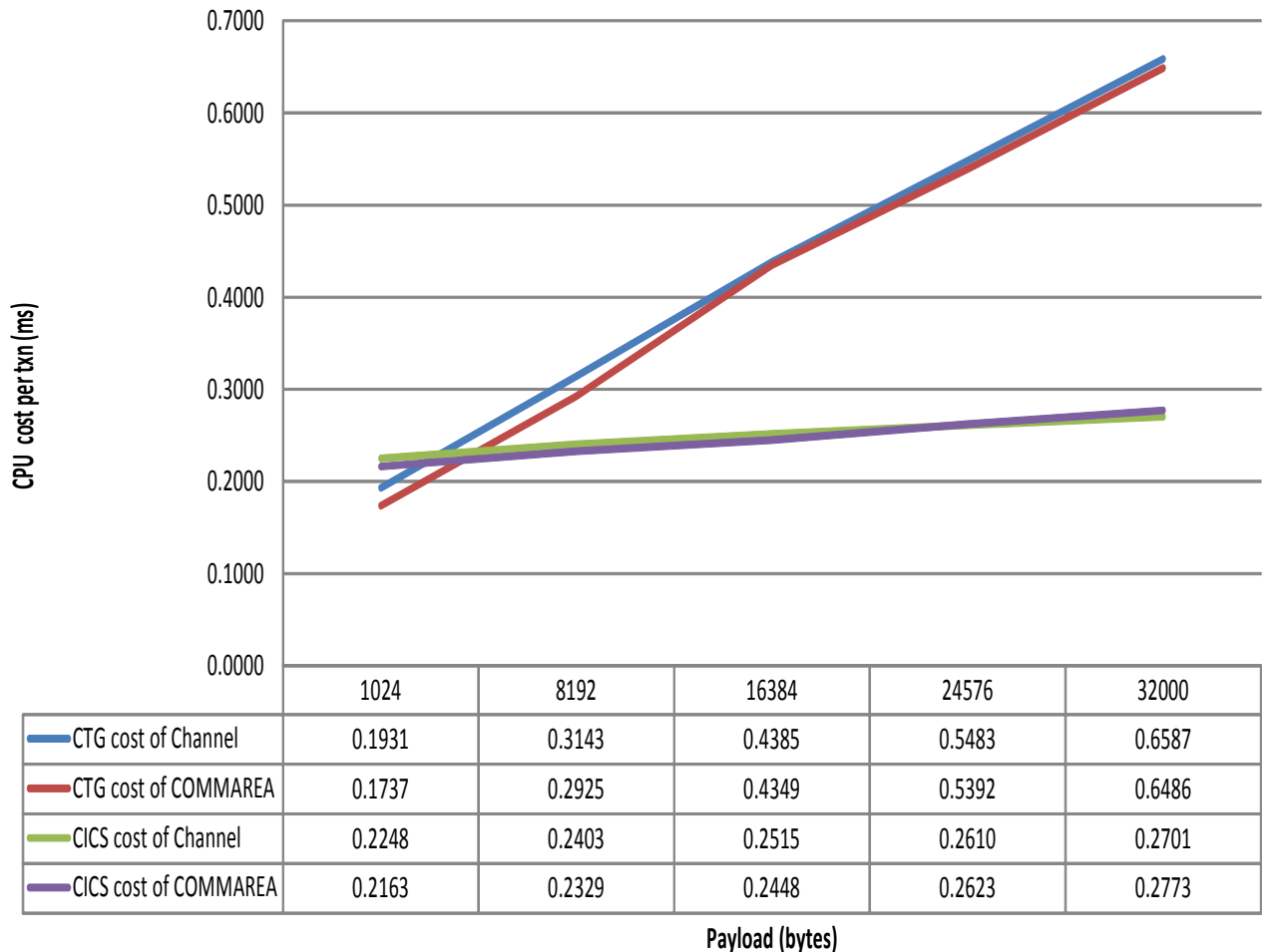
Illustration 4: “COMMAREA vs channel cost of CPU per transaction – 64-bit Gateway daemon” demonstrates the scenario using a 64-bit Gateway daemon.
