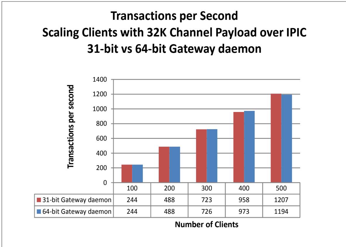
Illustration 7: “Scaling clients comparing 31-bit & 64-bit Gateway daemon”
