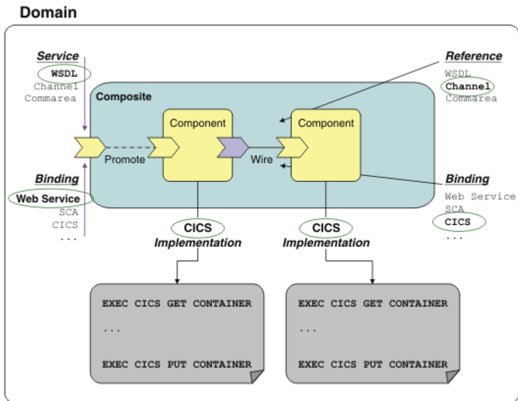
Fig 3: the same component as in Fig 2 but with the external service now implemented in CICS as a channel linkable program and bound to the original component with the CICS binding.
