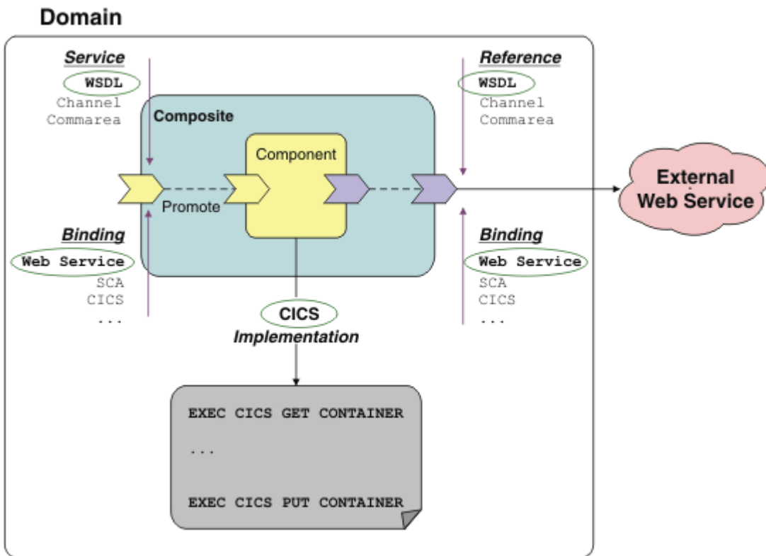
Fig 2: a simple CICS SCA component which makes use of an external Web Service using the web services binding.
