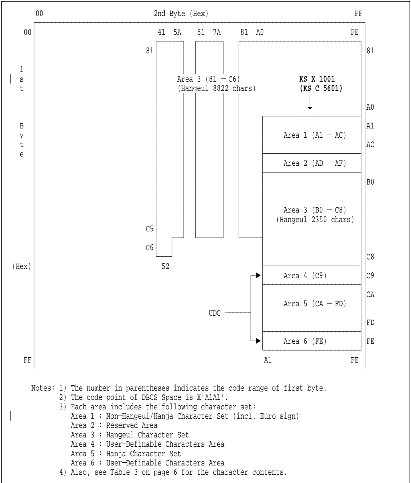
Figure 1. Code Structure for DBCS-PC
