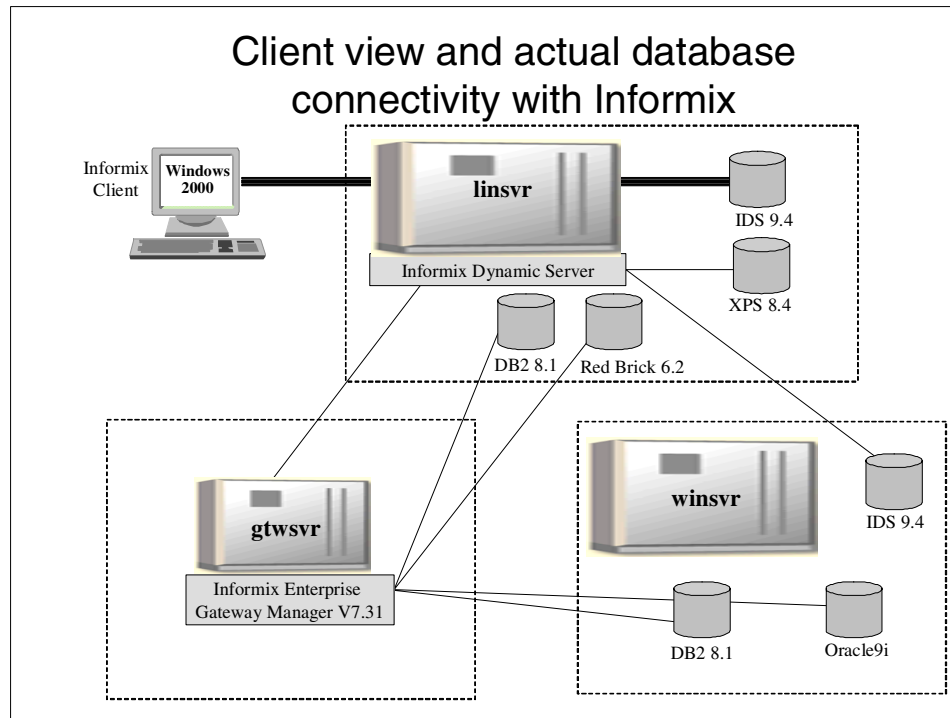
Figure 2-3 Client view of federated database and actual connectivity with Informix Database Server and Informix Enterprise Gateway Manager
