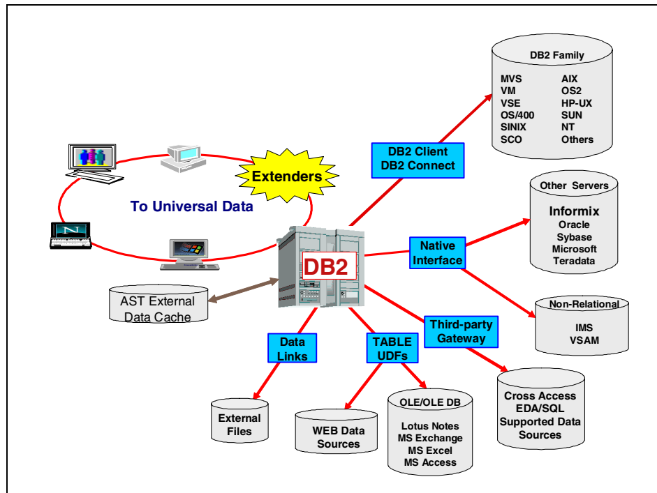
Figure 1-3 DB2 data federation
