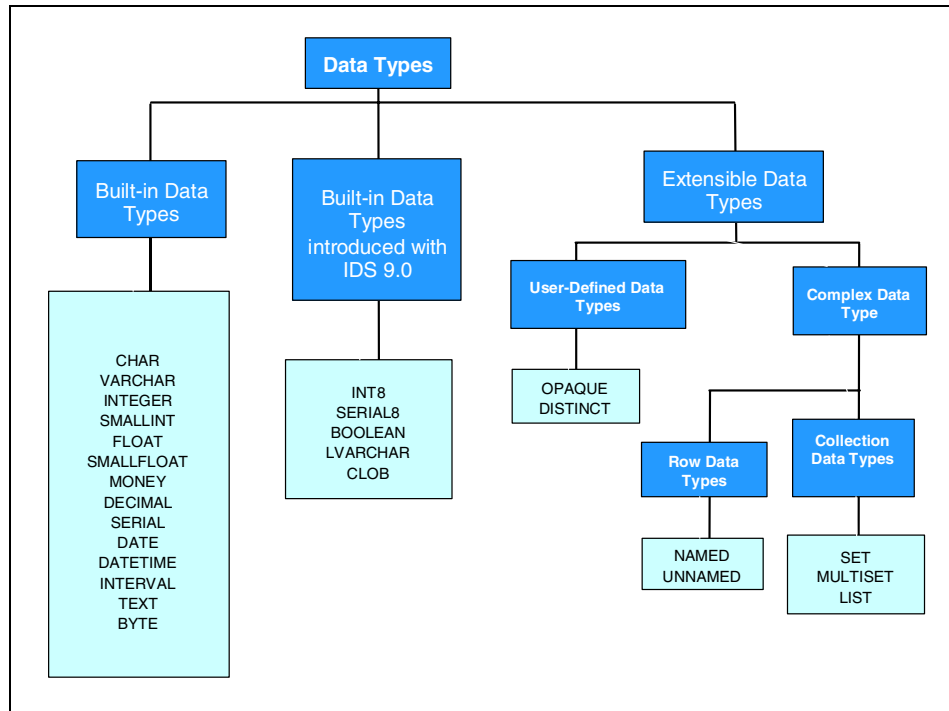
Figure 3-4 Data types
