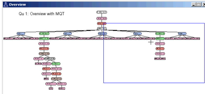
Figure 7-15 DB2 interactive explain graph for Query 1 with MQT
