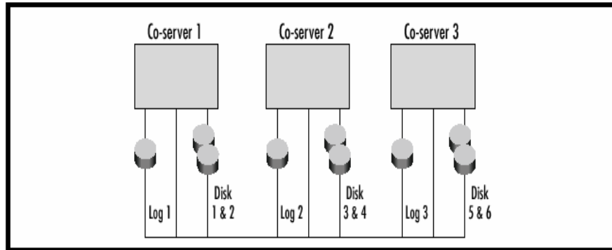
Figure 3-5 XPS architecture
