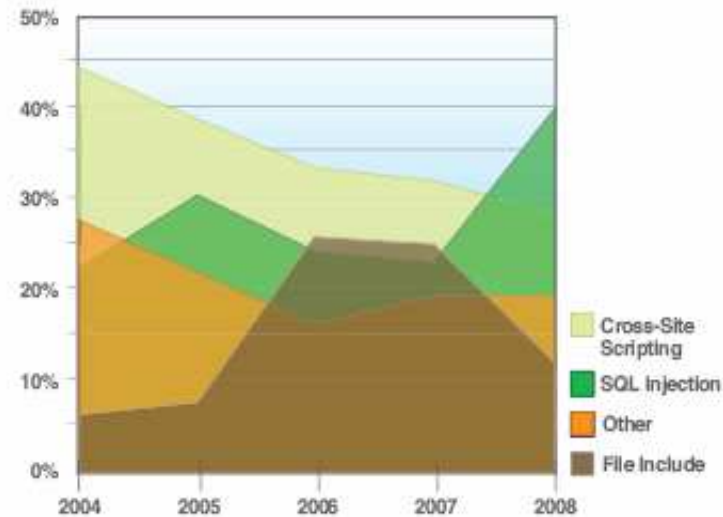
Figure 19: Web Application Vulnerabilities by Attack Technique, 2004 - 2008
