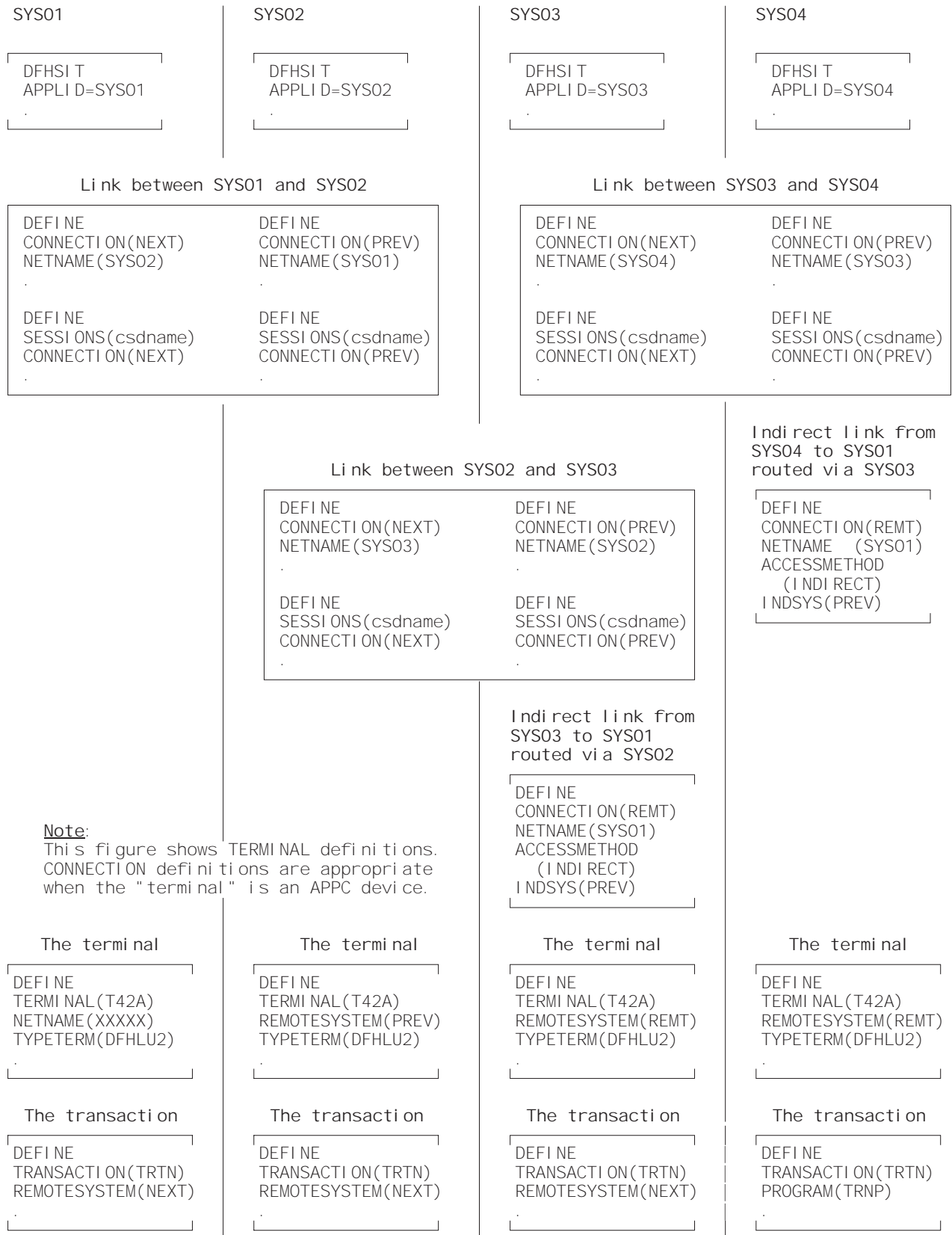
Figure 39. Defining indirect links for transaction routing. Because the remote terminal definitions in SYS04 and SYS03 do not specify the REMOTESYSNET option, indirect links are required.
