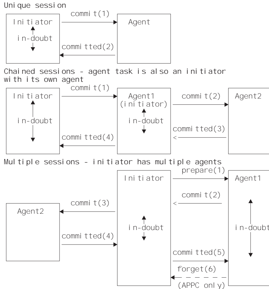
Figure 75. Syncpointing flows
