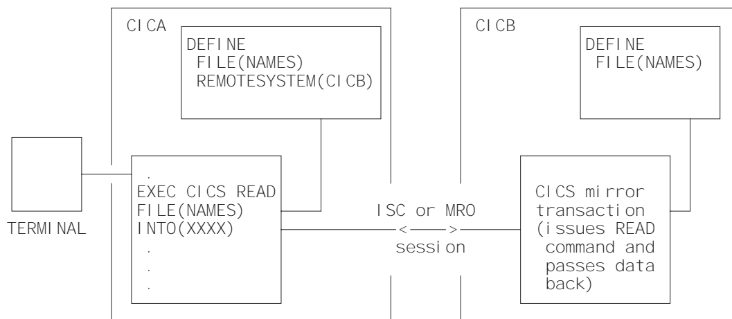
Figure 3. Function shipping
