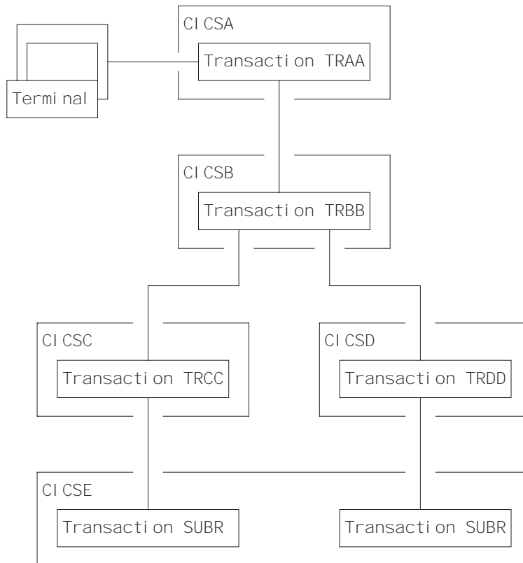
Figure 23. DTP in a multisystem configuration
