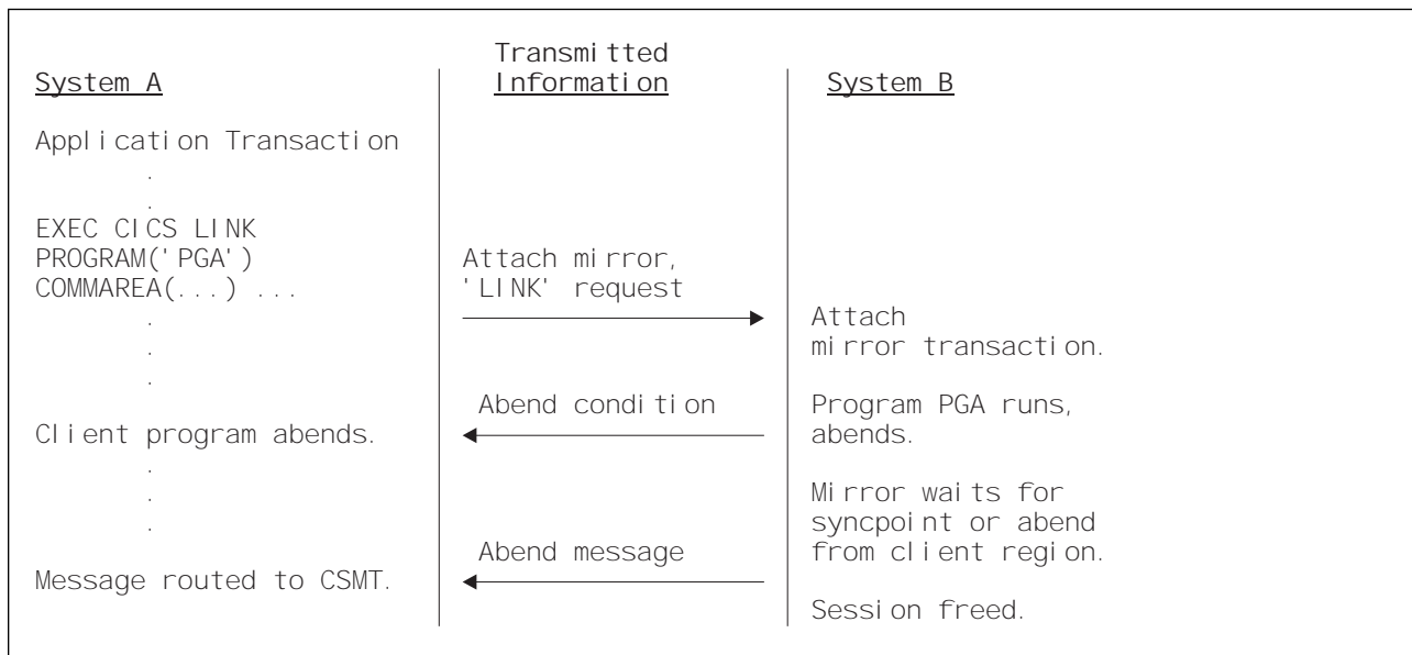
Figure 13. DPL with the server program abending
