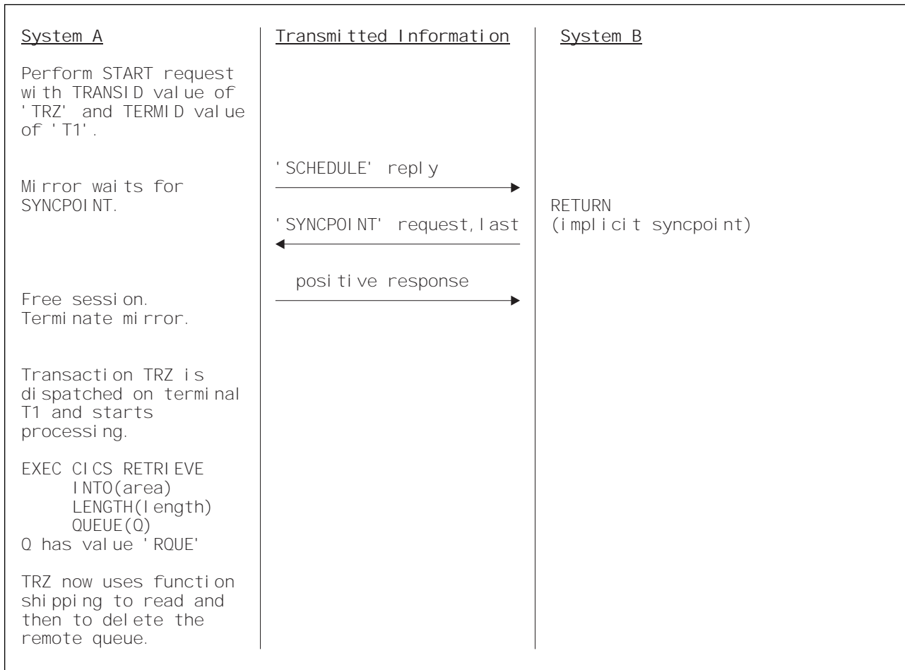
Figure 15 (Part 2 of 2). Asynchronous processing—remote transaction initiation. This example shows an MRO connection with long-running mirrors (MROLRM) specified for System A but not for System B. Note the different action of the mirror transaction on the two systems.
