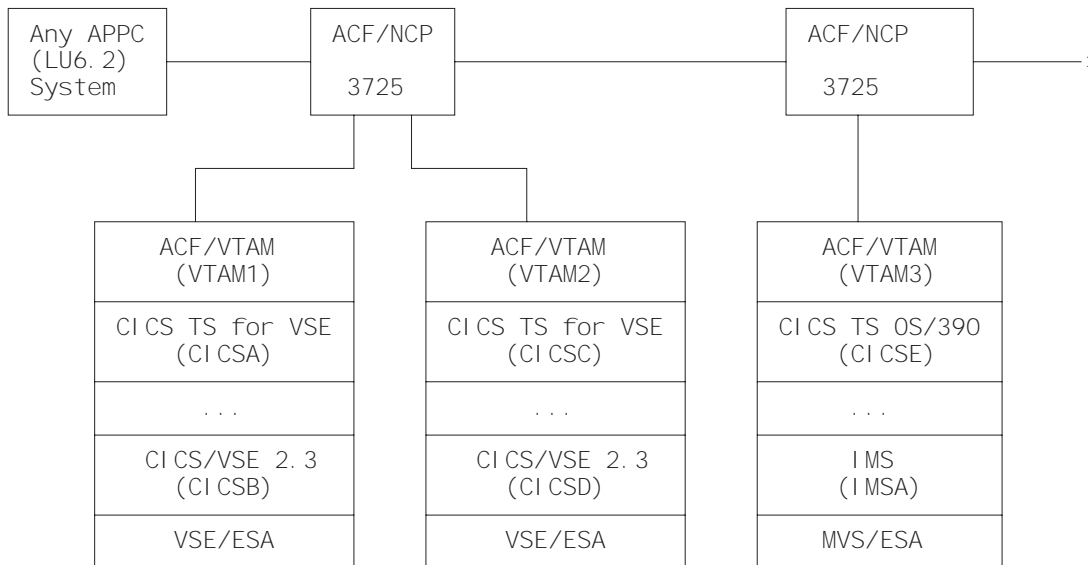
Figure 2. A possible configuration for intercommunicating systems
