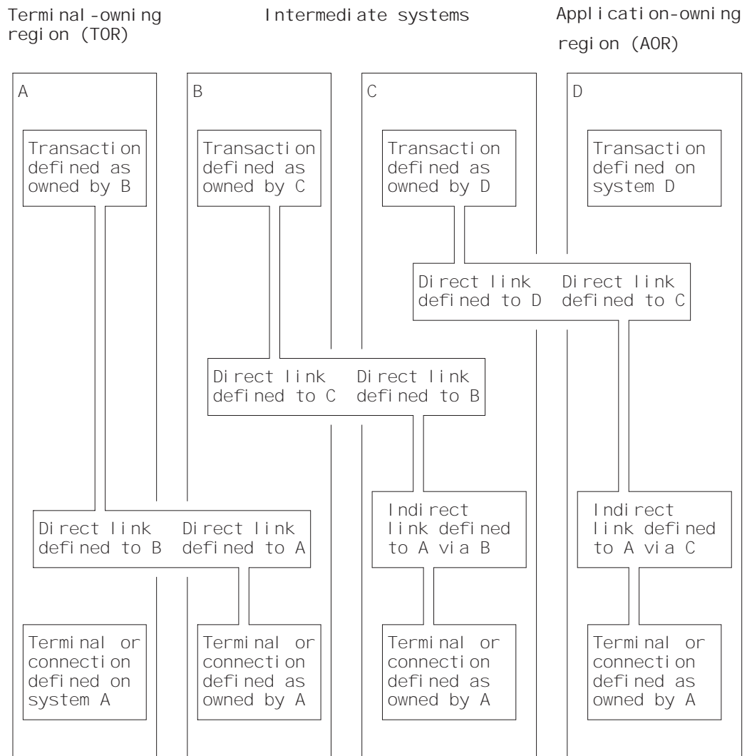
Figure 38. Indirect links for transaction routing
