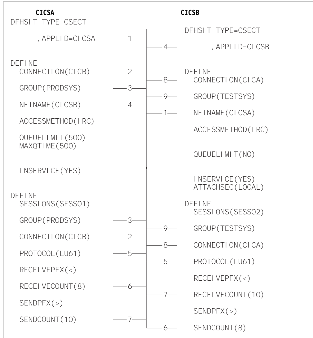
Figure 27. Defining compatible MRO nodes
