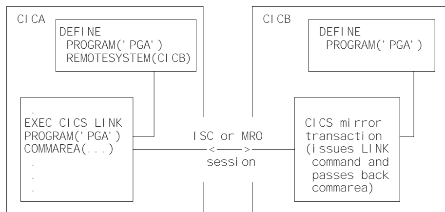
Figure 10. Distributed program link
