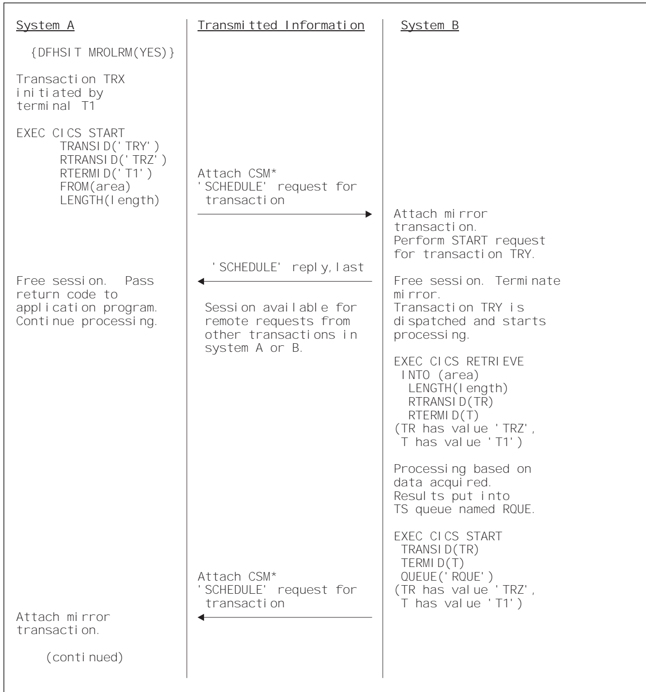
Figure 15 (Part 1 of 2). Asynchronous processing—remote transaction initiation
