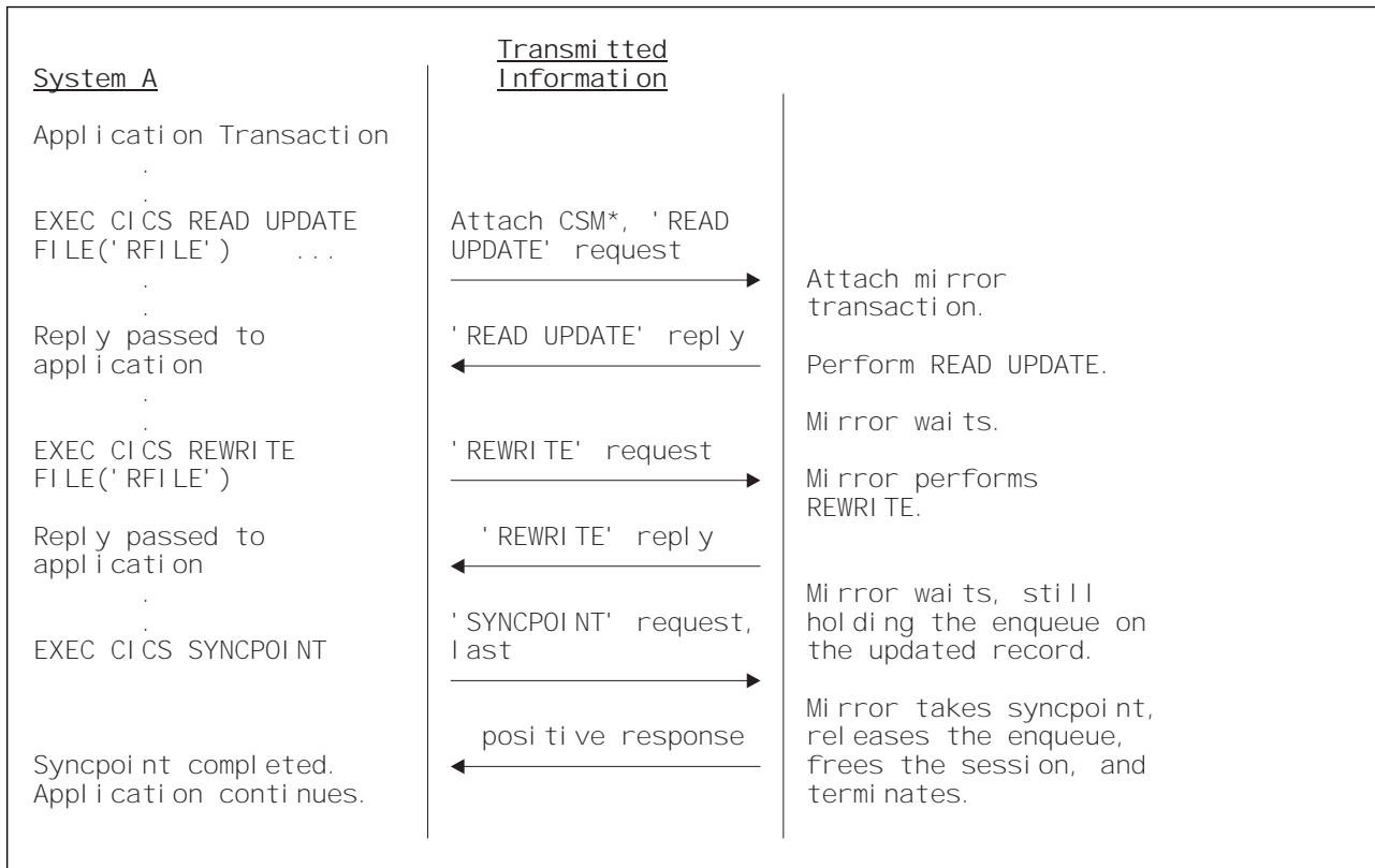
Figure 8. ISC or MRO function shipping—update. Because the mirror must wait for the REWRITE, it becomes long-running and is not terminated until SYNCPOINT is received. Note that the enqueue on the updated record would not be held beyond the REWRITE command if the file was not recoverable.
