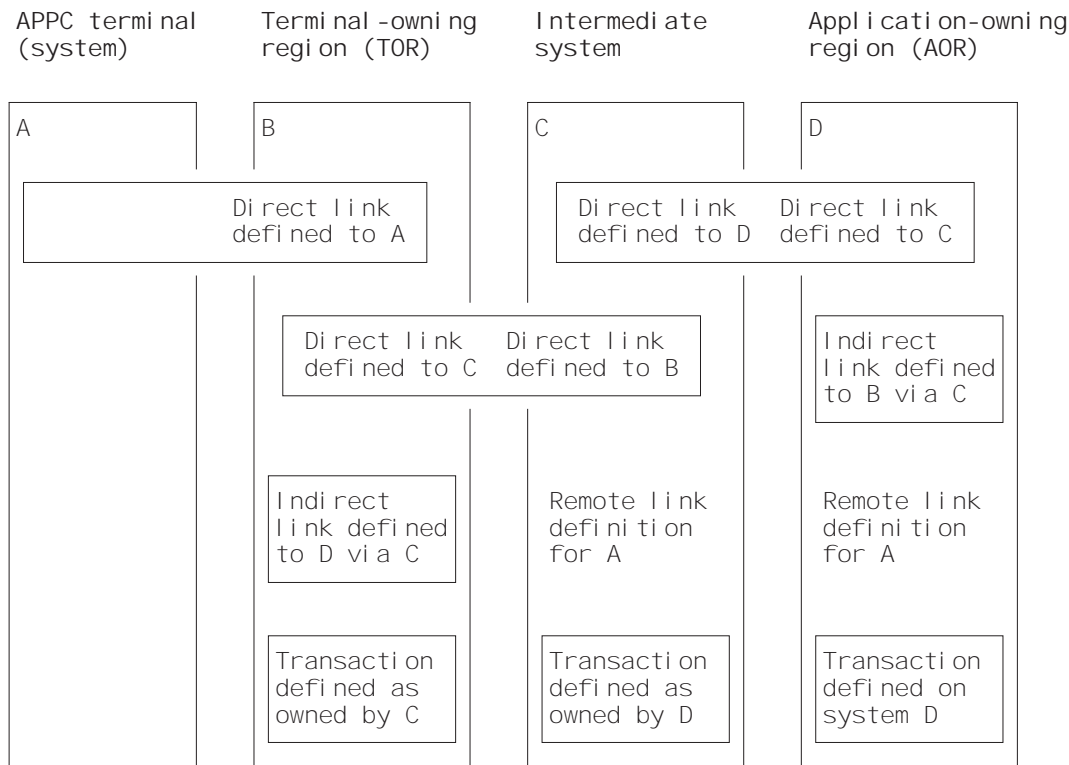
Figure 22. Transaction routing to an APPC terminal across daisy-chained systems
