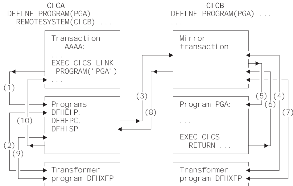
Figure 11. The transformer program and the mirror in DPL
