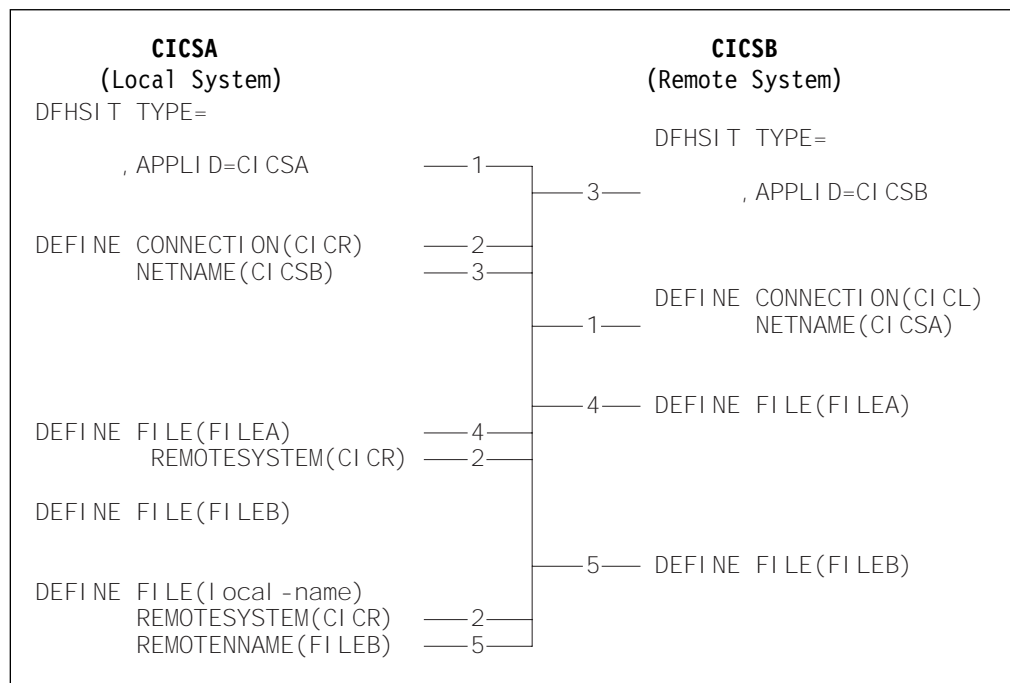
Figure 42. Local and remote resource names
