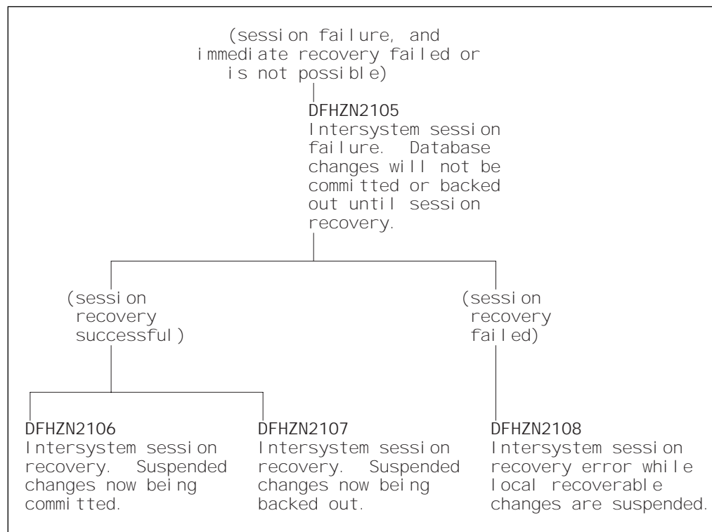
Figure 78. Session failure messages for INDOUBT(WAIT)
