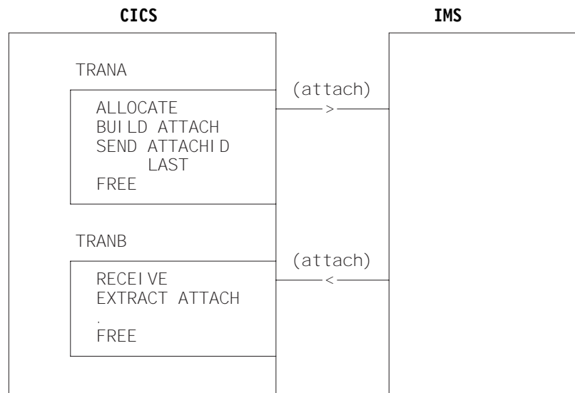
Figure 66. SEND and RECEIVE asynchronous processing – CICS front end
