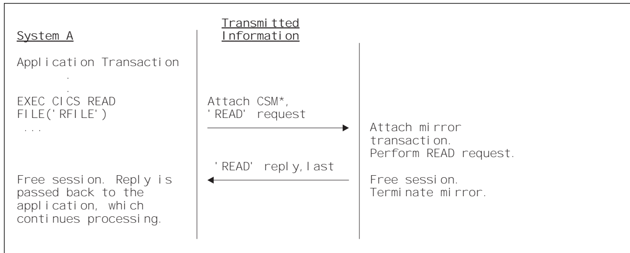
Figure 5. ISC function shipping—simple inquiry. Here no resource is being changed; the session is freed and the mirror task is terminated immediately.
