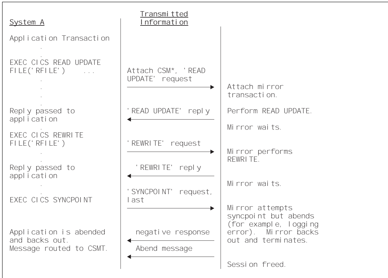
Figure 9. ISC or MRO function shipping—update with ABEND. This is similar to the previous example, except that an abend occurs during syncpoint processing.
