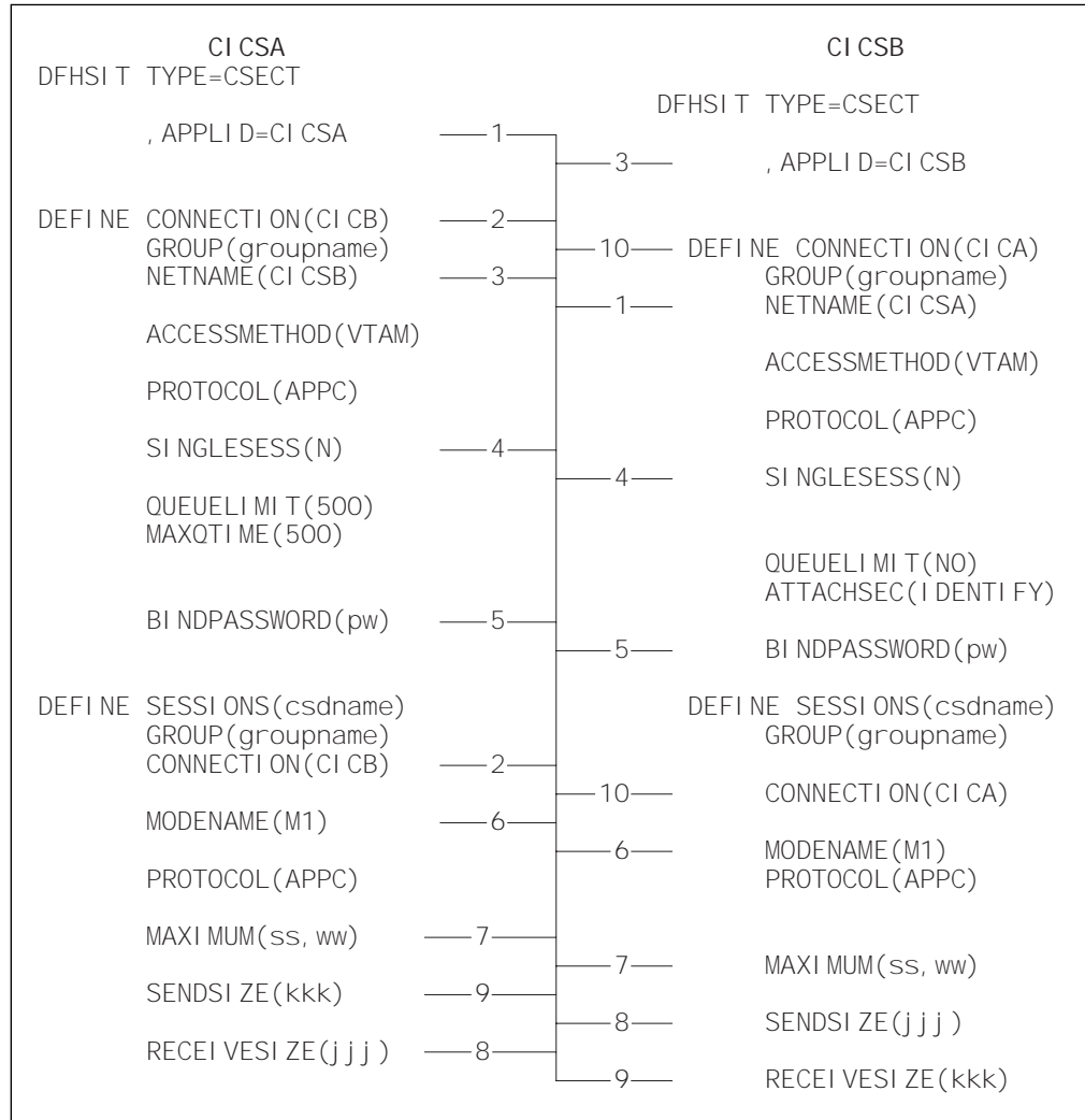
Figure 32. Defining compatible CICS APPC ISC nodes
