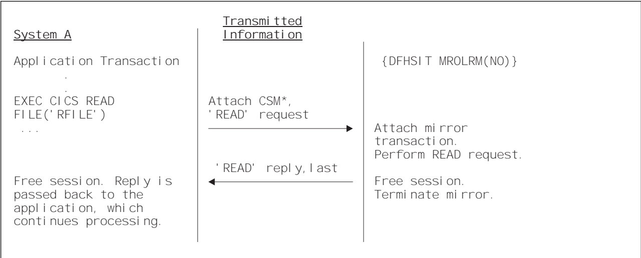
Figure 6. MRO function shipping—simple inquiry. Here no resource is being changed. Because long-running mirror tasks are not specified, the session is freed by System B and the mirror task is therefore terminated immediately.
