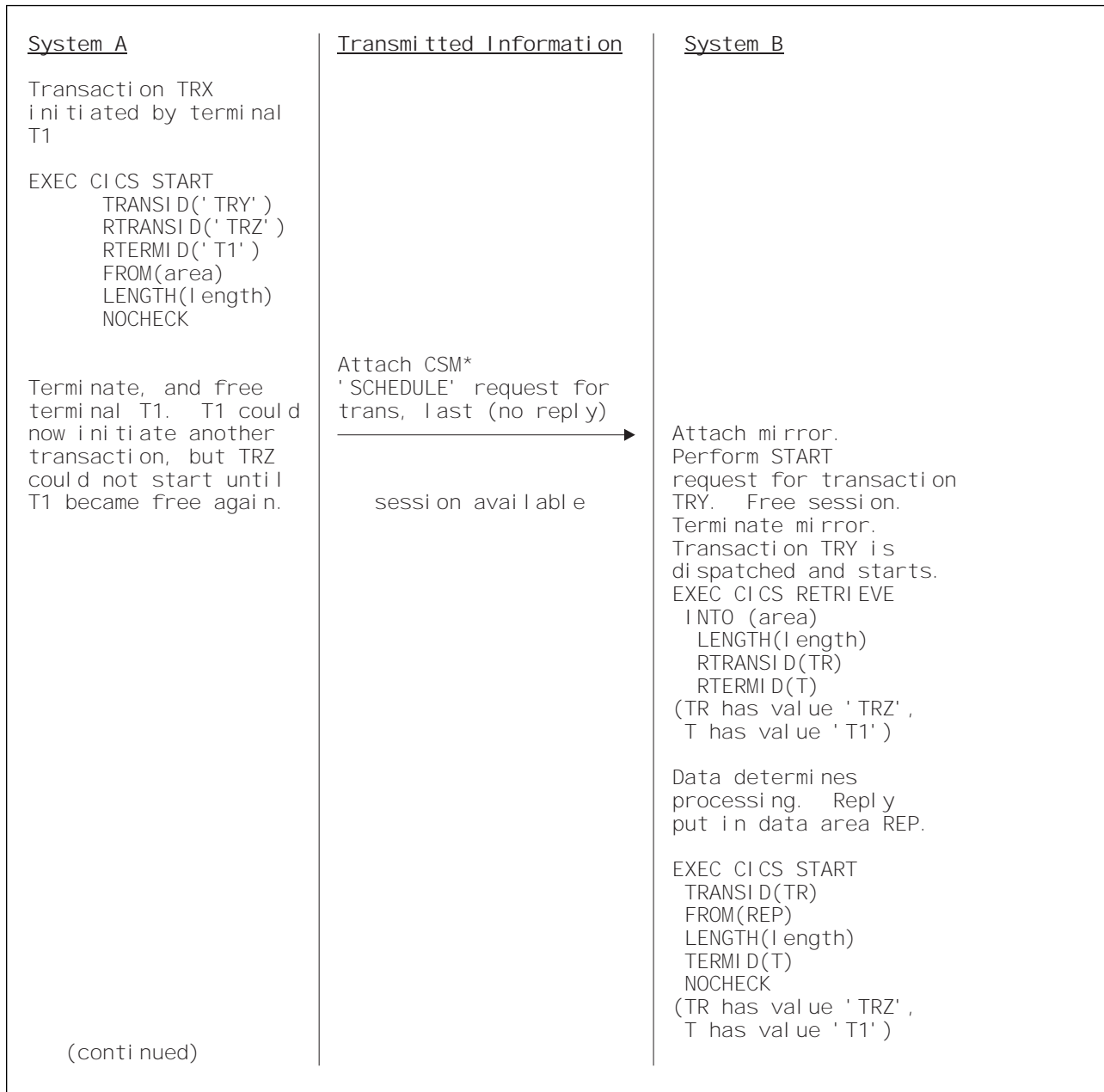
Figure 16 (Part 1 of 2). Asynchronous processing—remote transaction initiation using NOCHECK
