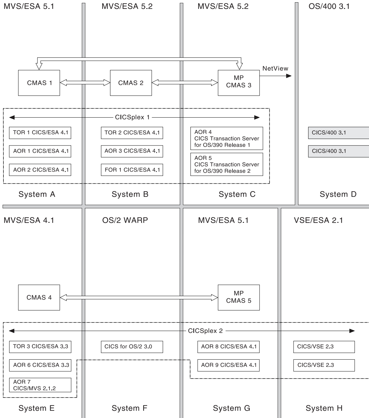
Figure 8. Adding CMAS-to-CMAS links to the example map. Eight links have been defined, giving full connectivity among CMASs managing the same CICSplexes.
