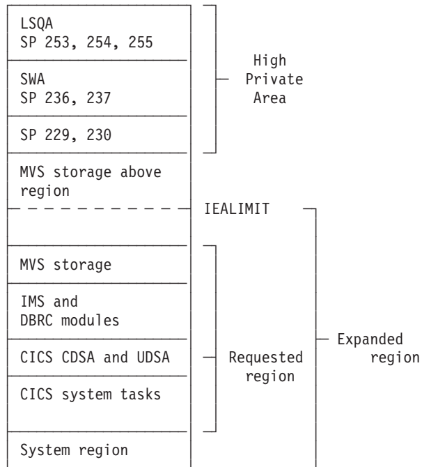
Figure 79. CICS private area immediately after system initialization
