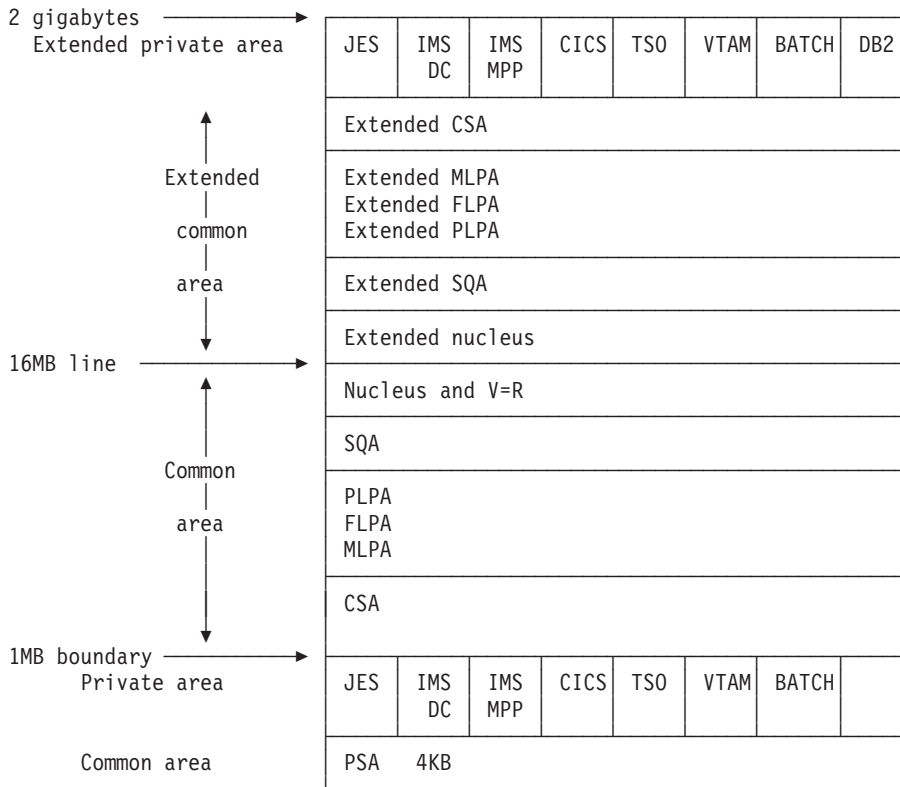
Figure 78. Virtual storage map for MVS/ESA
