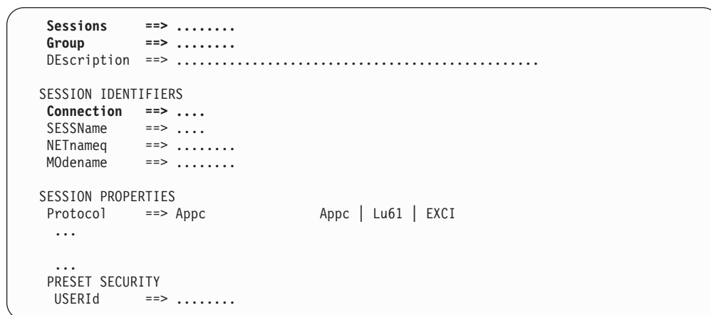
Figure 33. The DEFINE panel for SESSIONS
