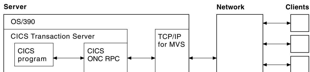
Figure 41. How CICS ONC RPC might be used
