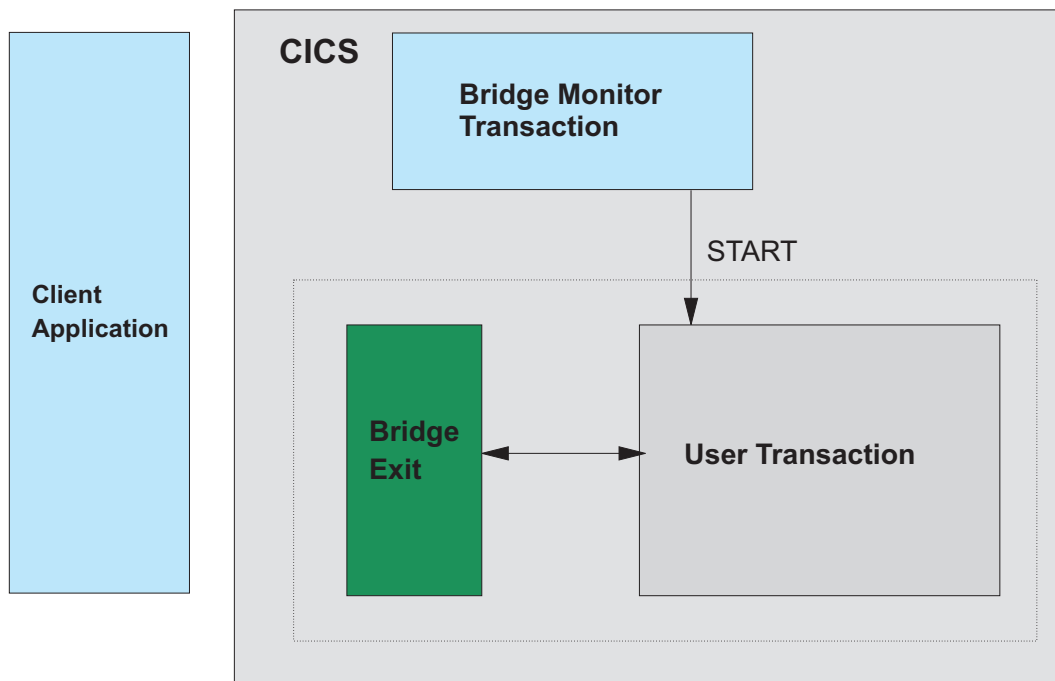
Figure 12. The two-task model
