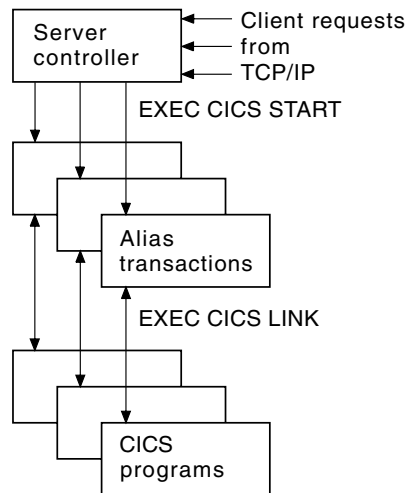
Figure 47. The server controller and alias transactions
