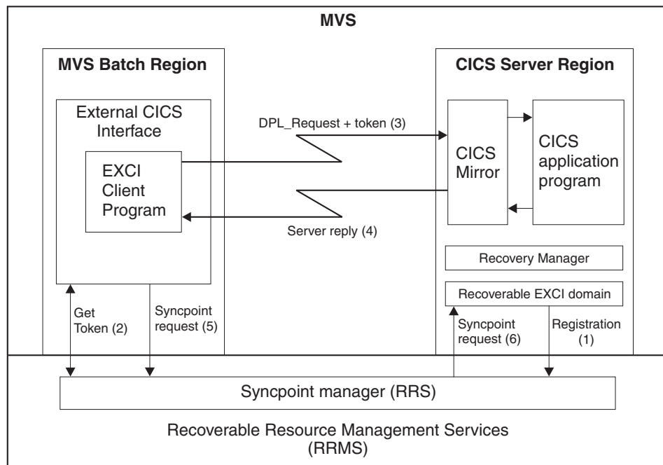
Figure 30. Conceptual view of EXCI client and CICS server region using RRMS. The main (numbered) steps within a unit-of-recovery are described in the list following the diagram
