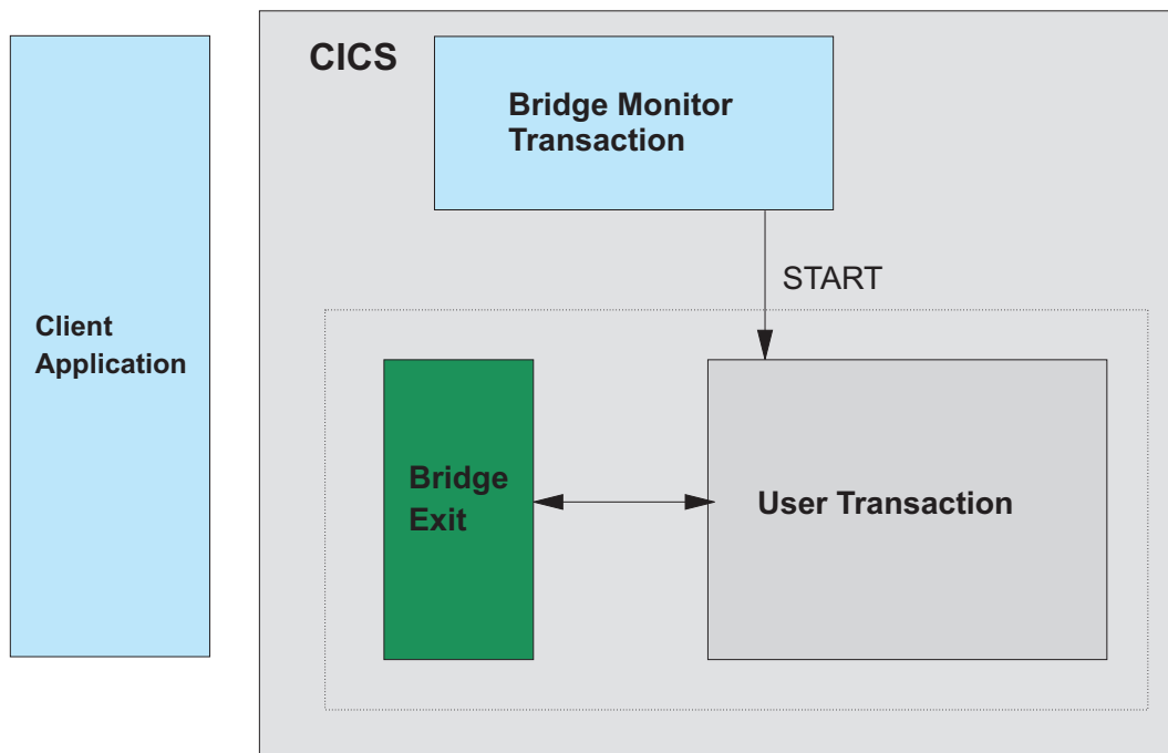
Figure 13. The single message model
