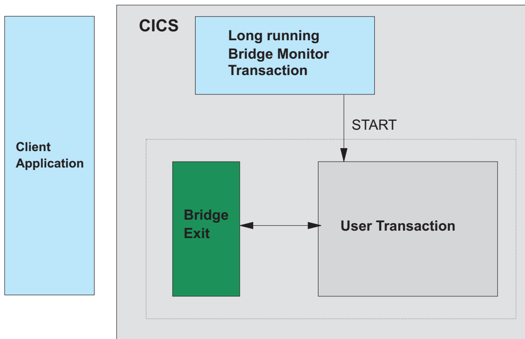
Figure 11. The long running monitor model
