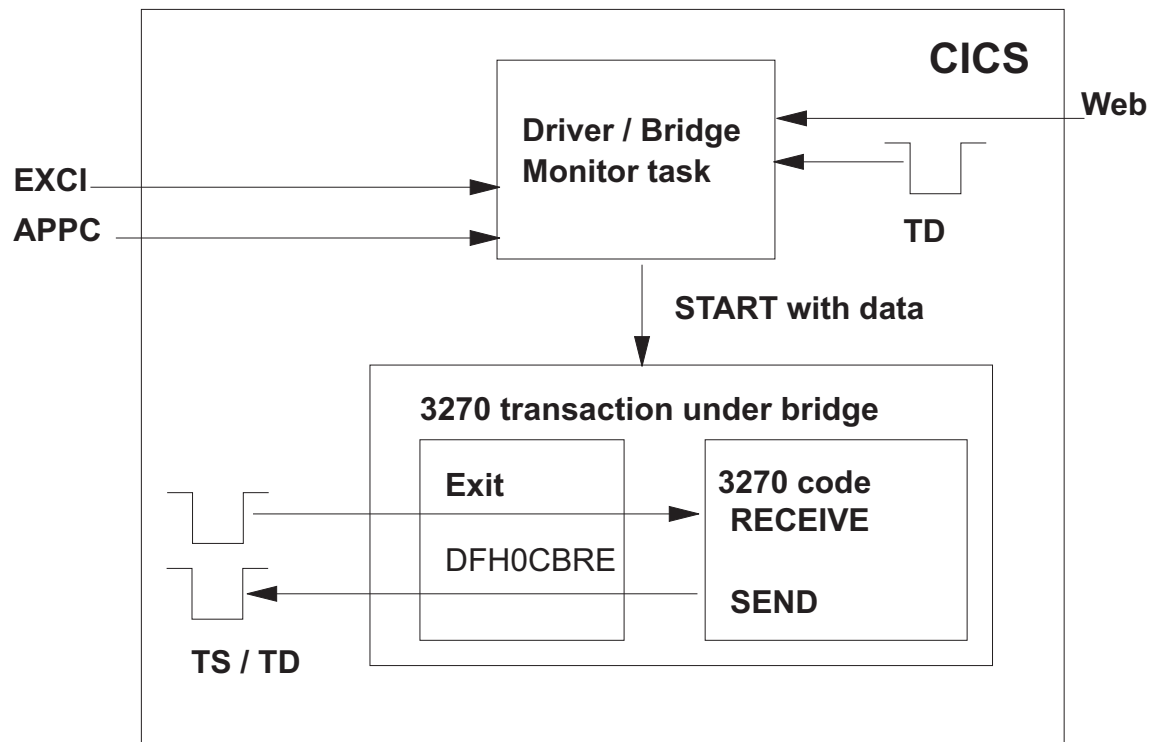
Figure 22. The supplied TS/TD bridge exit
