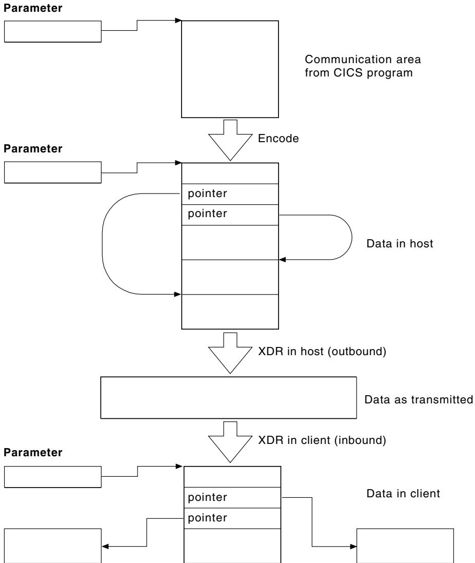
Figure 51. Data flow from CICS program to client
