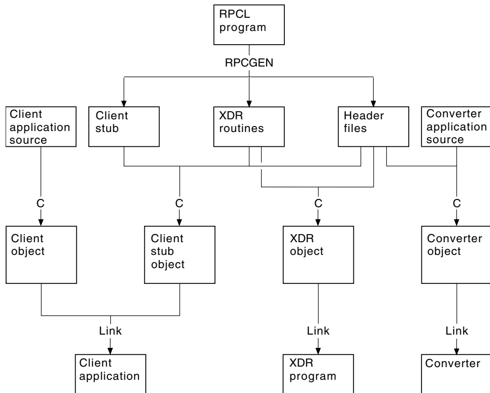
Figure 70. Program development with CICS ONC RPC
