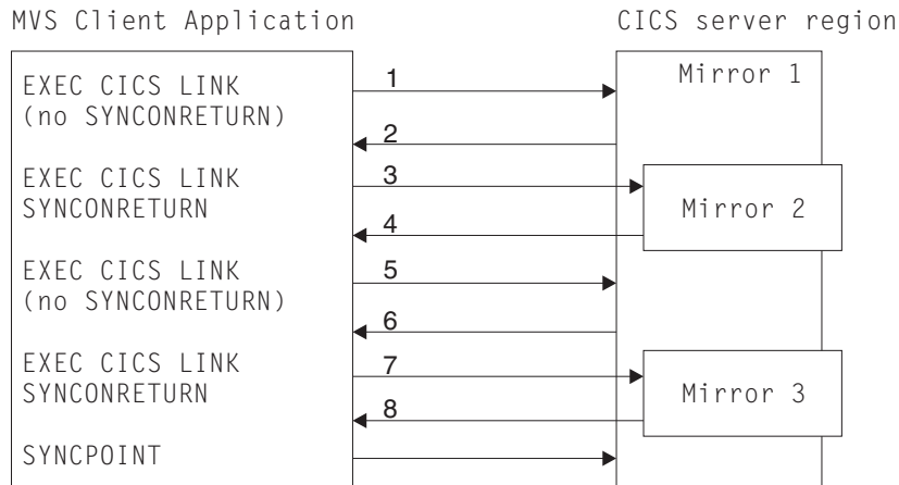
Figure 31. Effect of mixing DPL requests with and without SYNCONRETURN
