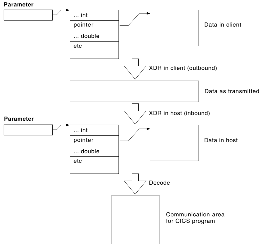
Figure 49. Data flow from client to CICS program
