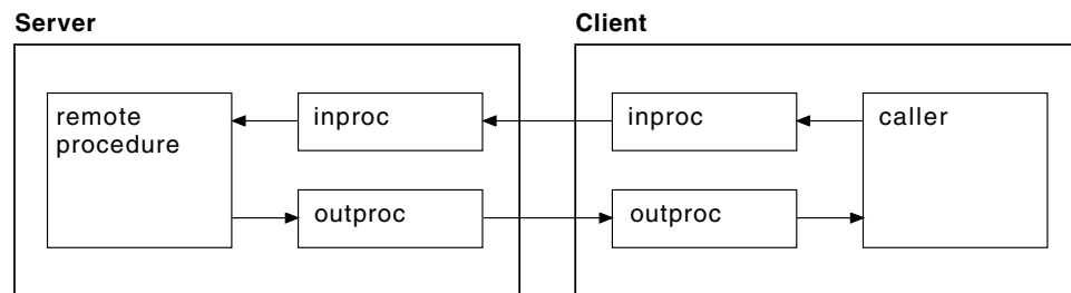
Figure 43. XDR routines used in a remote procedure call
