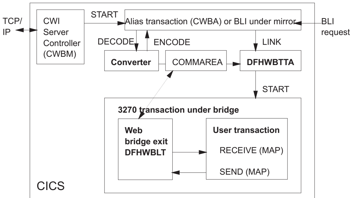
Figure 23. The Web supplied bridge exit
