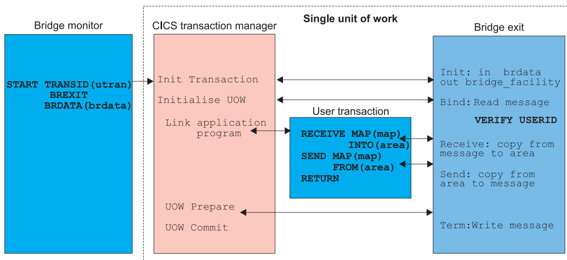
Figure 9. A simple terminal transaction
