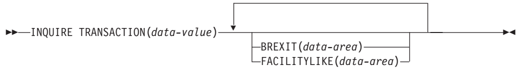
Figure 19. INQUIRE TRANSACTION (extract)
