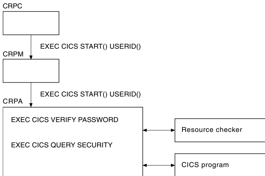
Figure 76. How CICS security interacts with CICS ONC RPC operations
