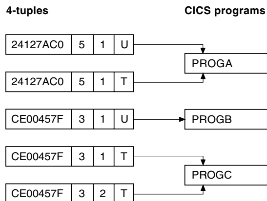
Figure 46. Remote procedures and CICS programs
