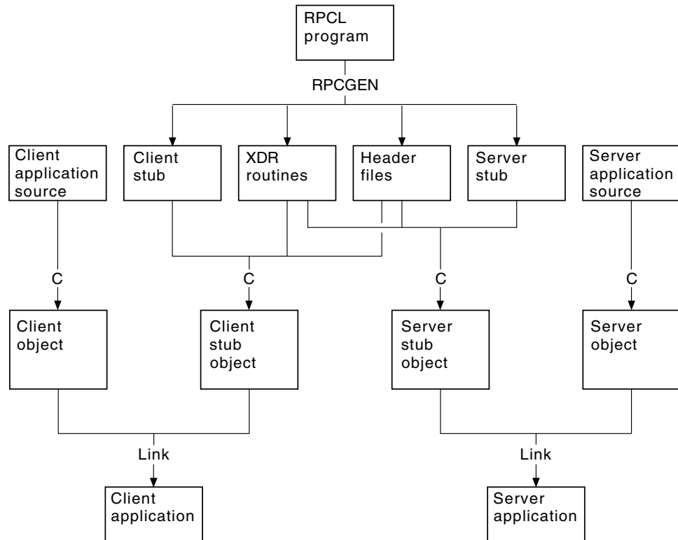
Figure 44. Using the RPCGEN compiler
