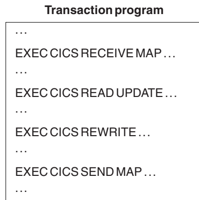
Figure 6. CICS functions in a single application program
