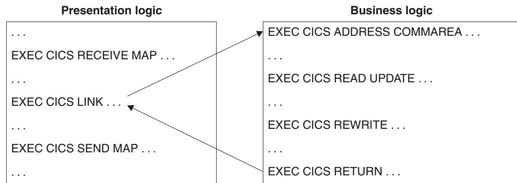
Figure 7. Separation of business and presentation logic
