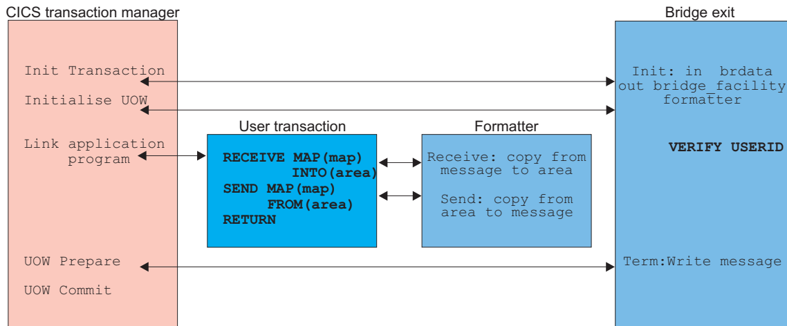
Figure 10. A simple terminal transaction using a formatter
