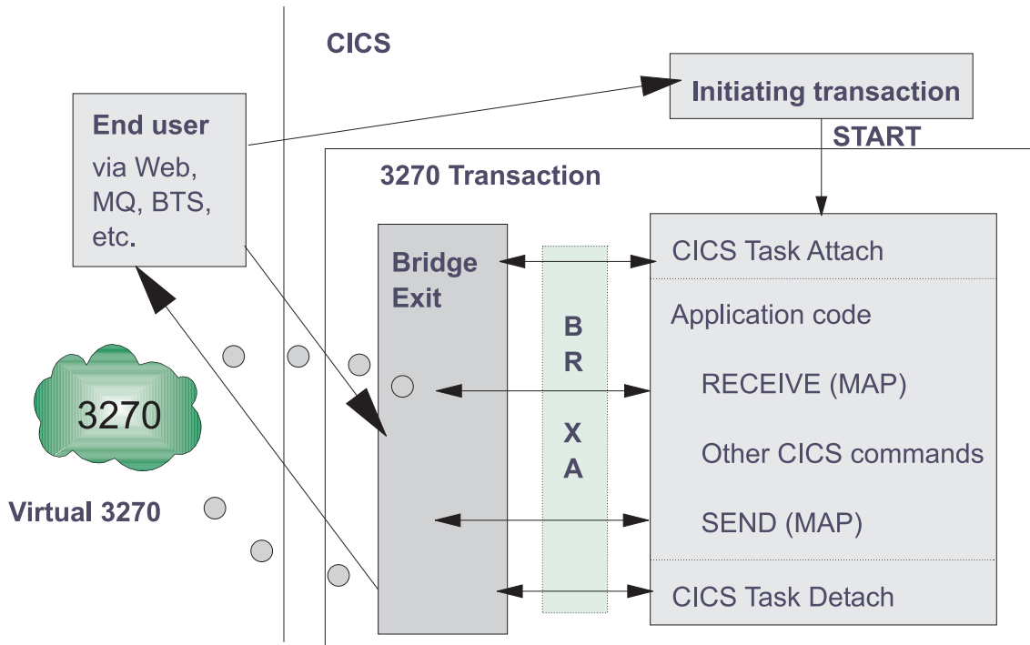
Figure 8. The 3270 bridge environment
