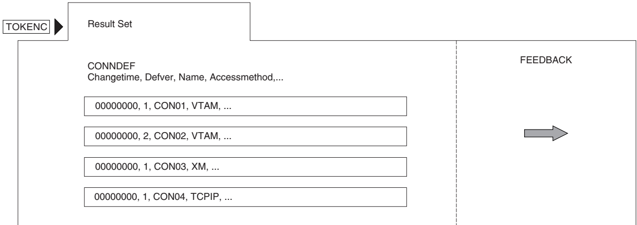
Figure 19. Using PERFORM OBJECT to install BAS definitions
