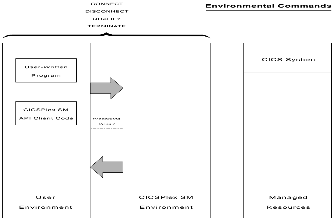
Figure 1. API commands involved in managing a thread
