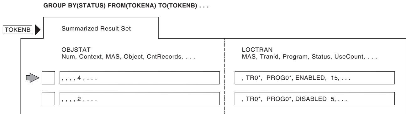
Figure 10. Using GROUP to summarize result set records
