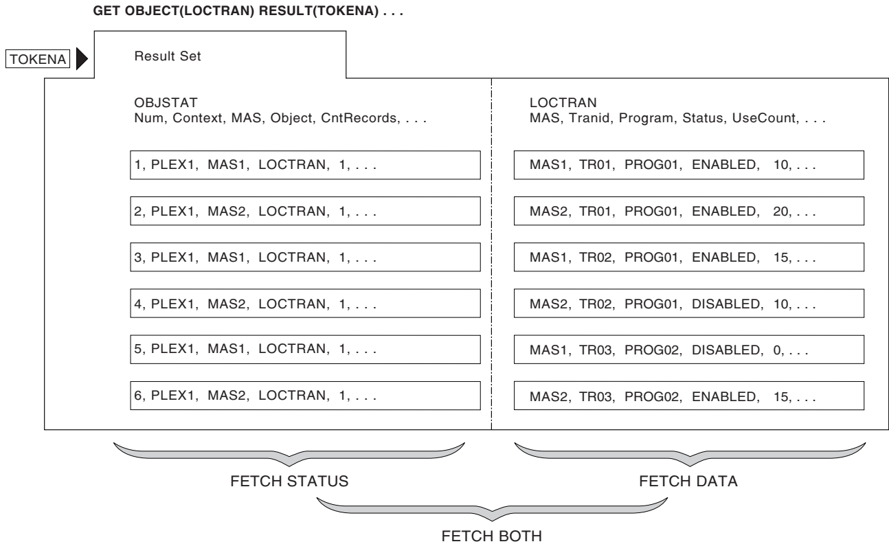
Figure 7. Using FETCH to retrieve result set records
