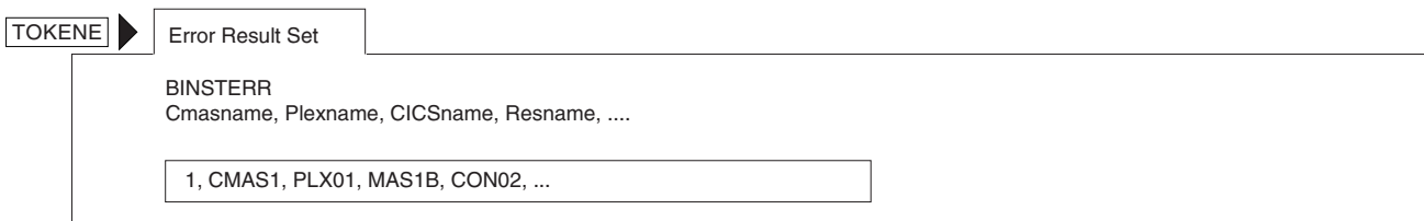
Figure 21. BINSTERR error result set
