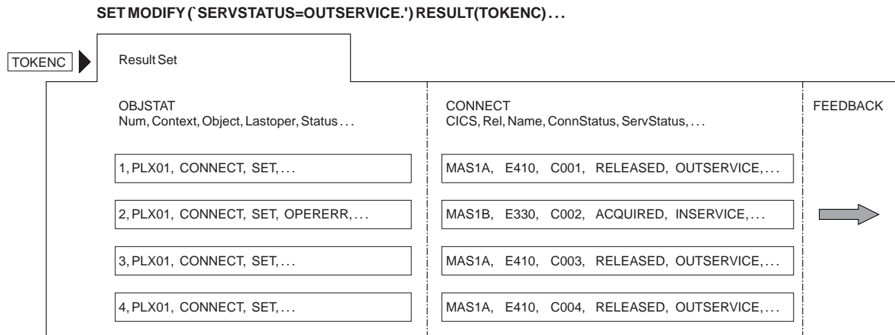
Figure 17. Using SET to modify result set records
