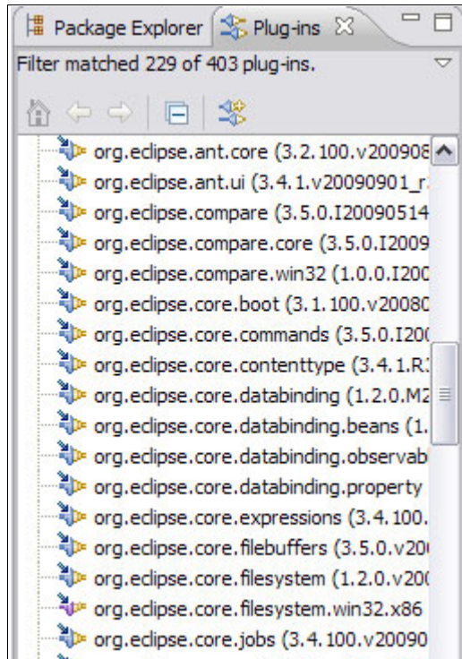
Figure 4-4 Plug-in view
