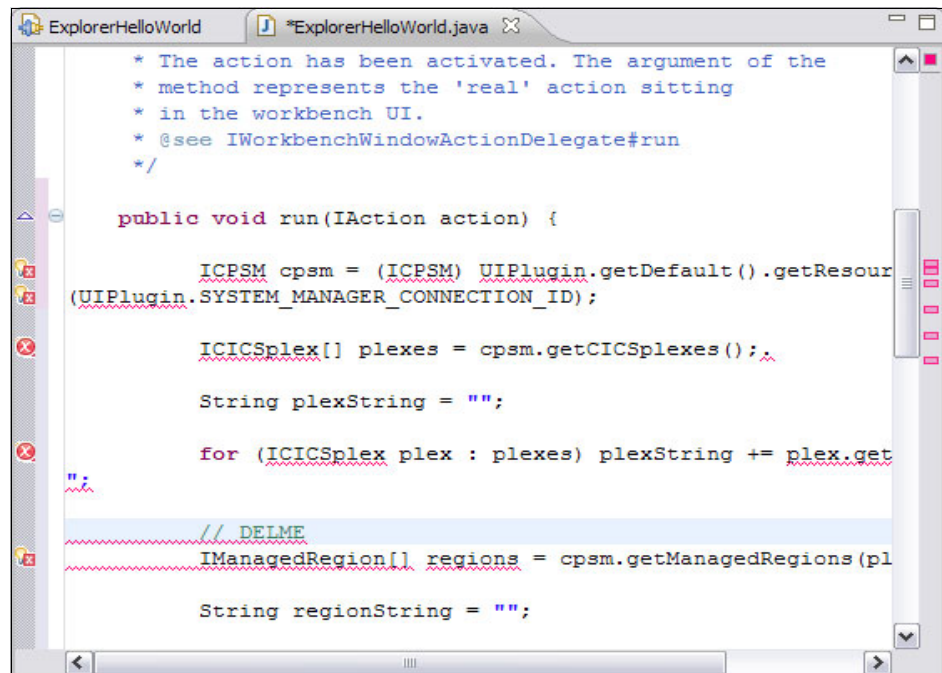
Figure 4-16 ExplorerHelloWorld dependencies
