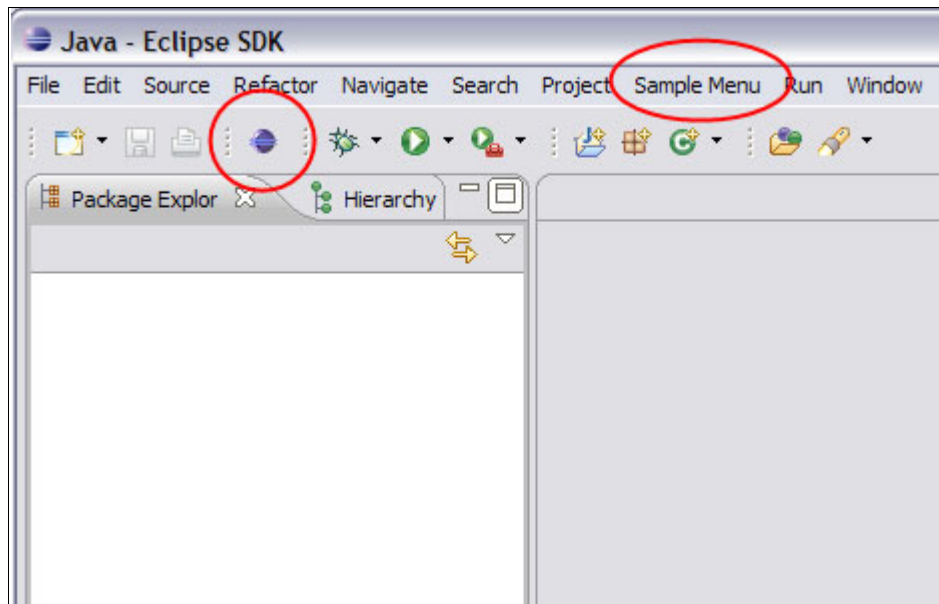
Figure 4-9 HelloWorldOne test
