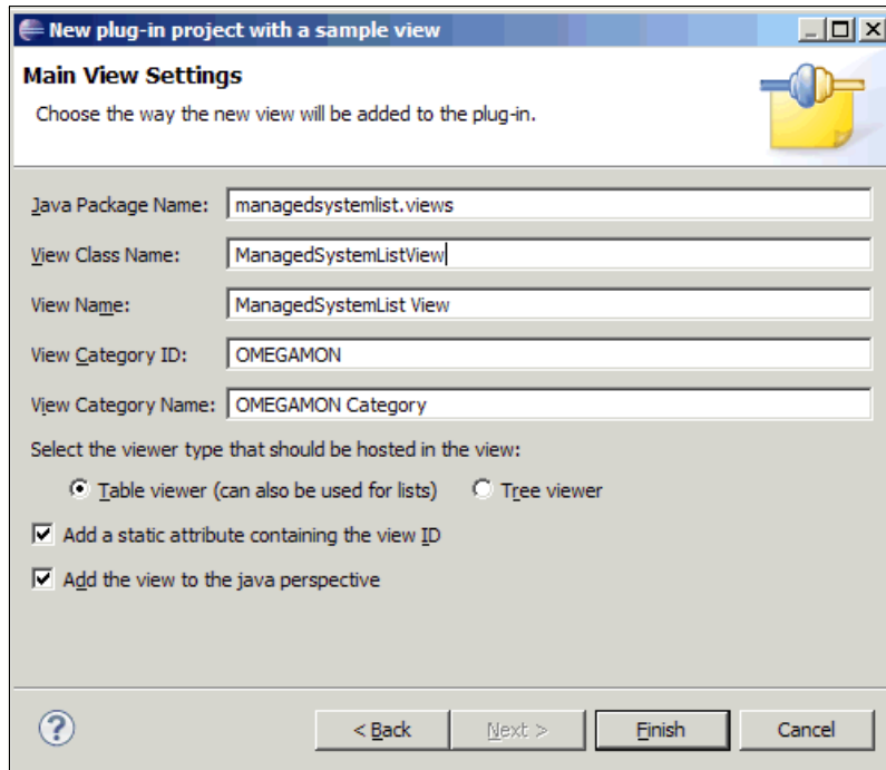
Figure 6-11 Managed System List Main view settings dialog
