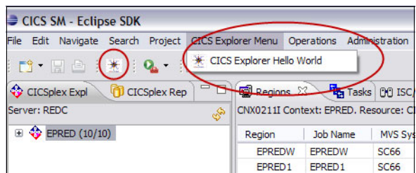
Figure 4-24 Customized ExplorerHelloWorld
