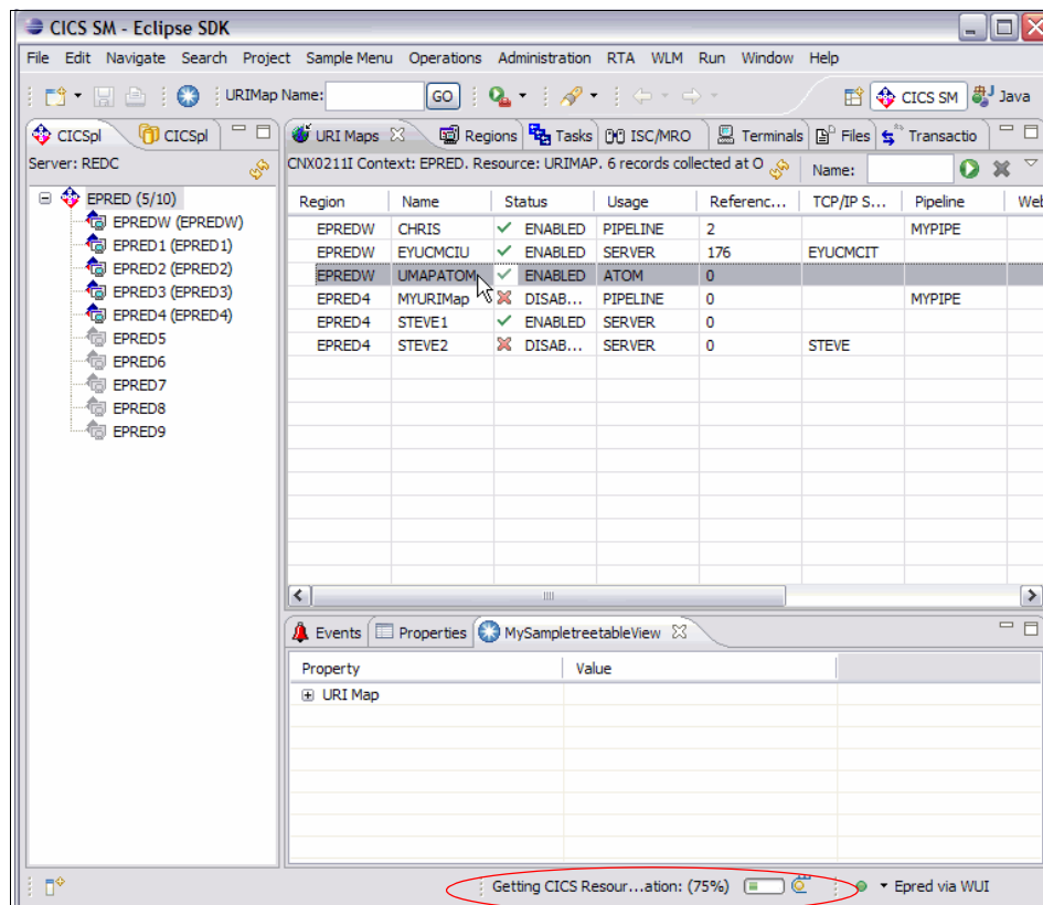
Figure 5-33 Background process indicated with progress bar
