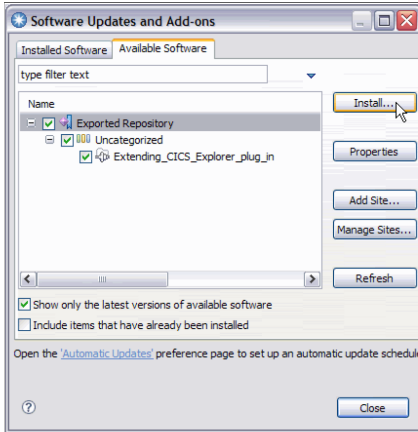
Figure 5-48 Select plug-in
