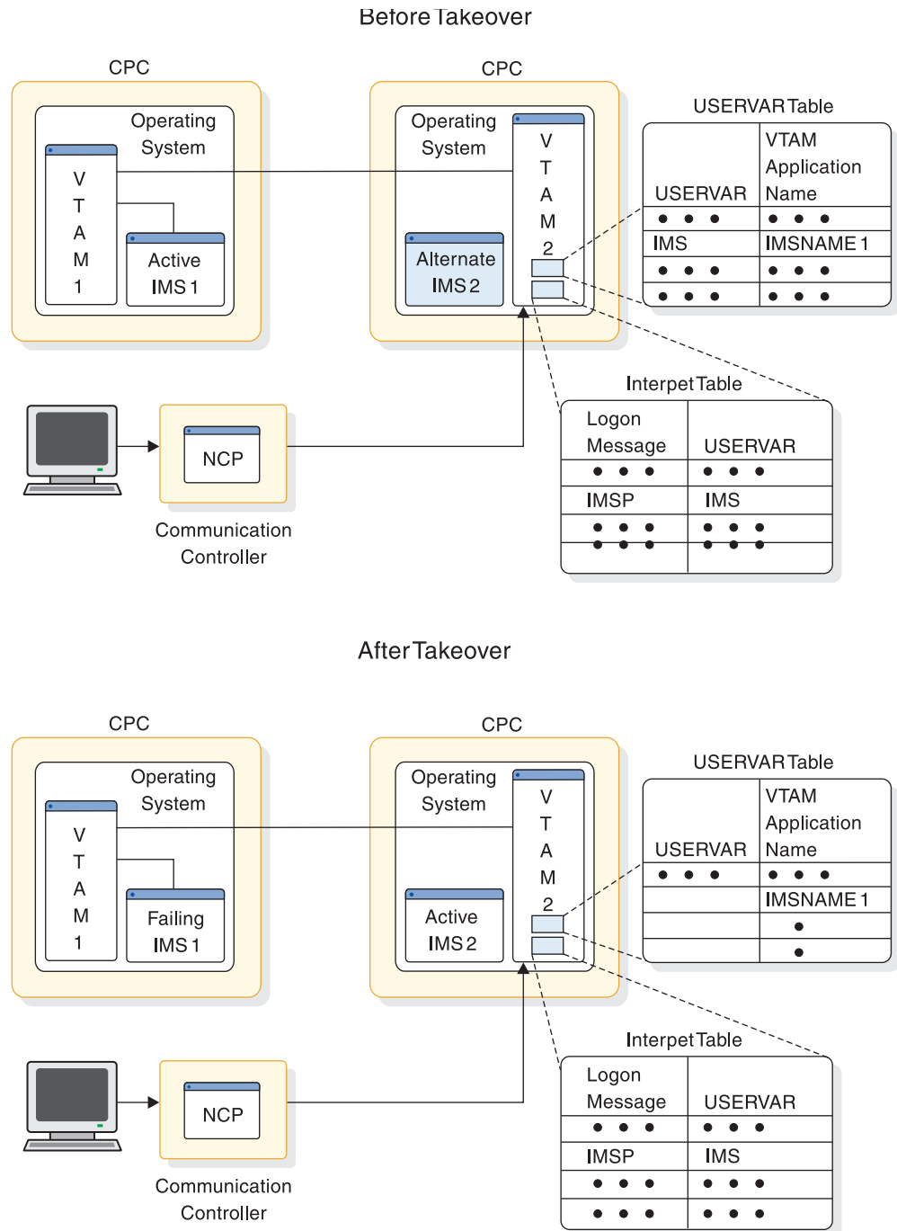
Figure 71. VTAM processing of the logon in an XRF complex that uses USERVAR
