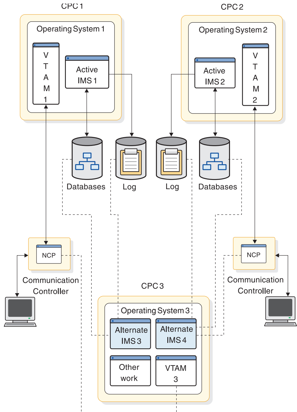
Figure 83. Two XRF complexes in three CPCs
