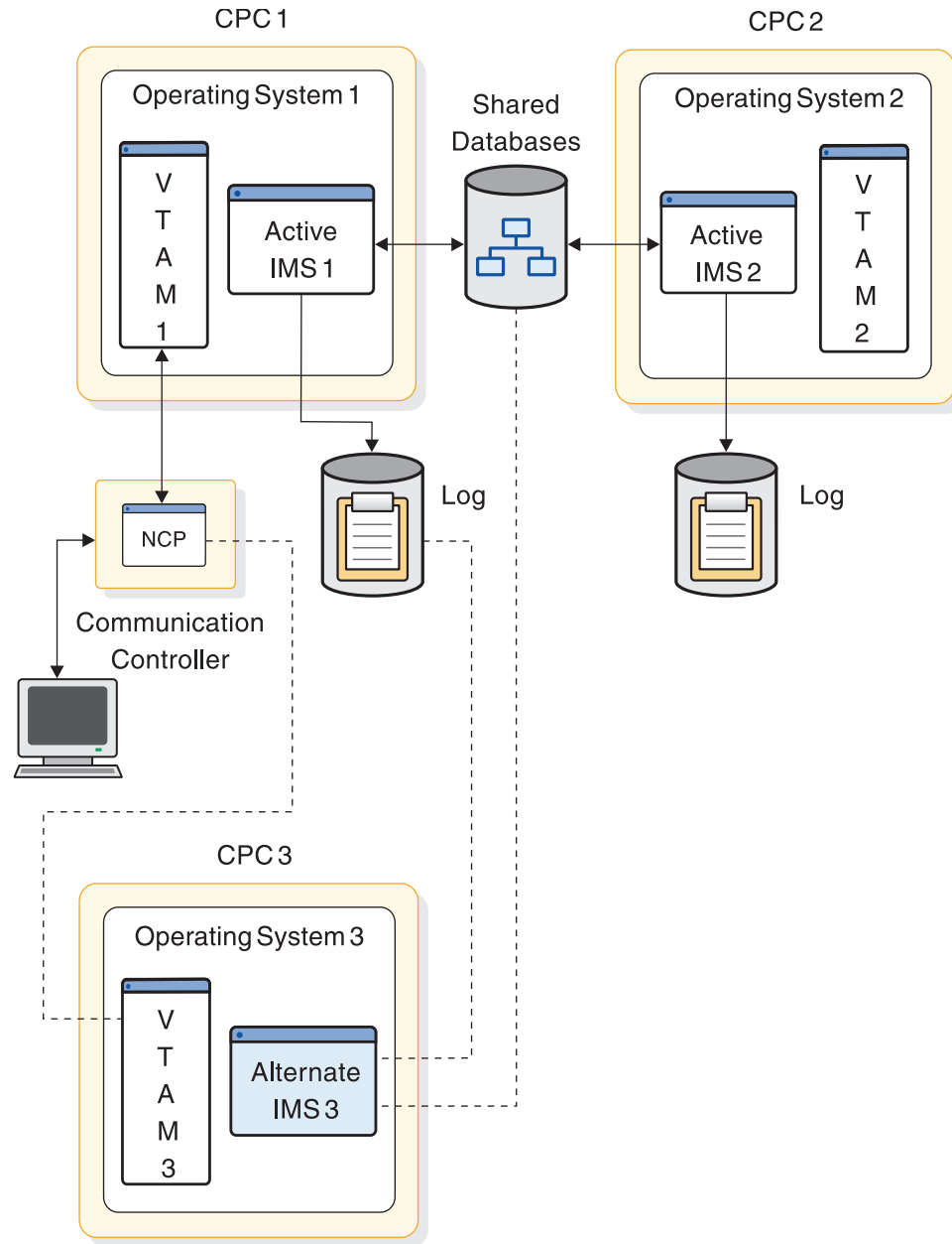
Figure 82. One XRF complex in two CPCs and a non-XRF IMS
