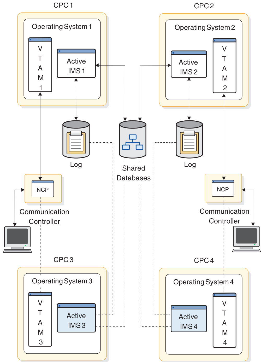
Figure 84. Two XRF complexes in four CPCs
