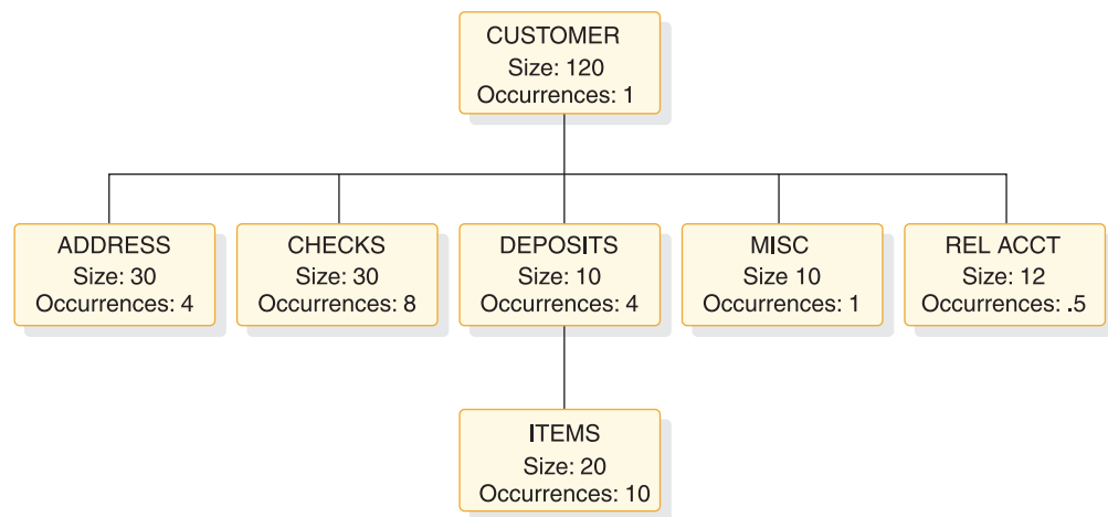
Figure 244. Segment sizes and average segment occurrences
