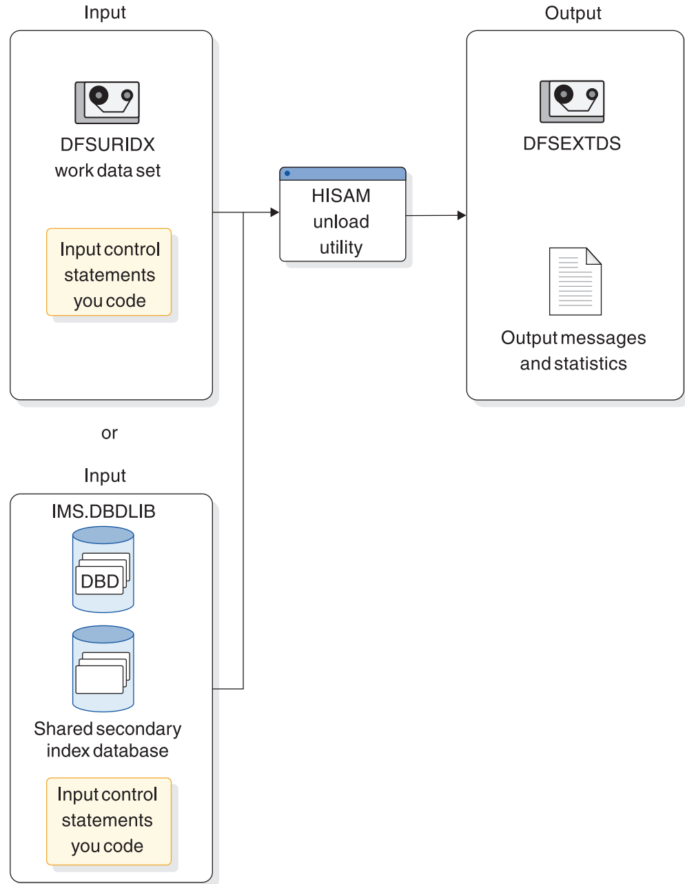
Figure 265. HISAM Reorganization Unload utility used for extract secondary indexing operations
