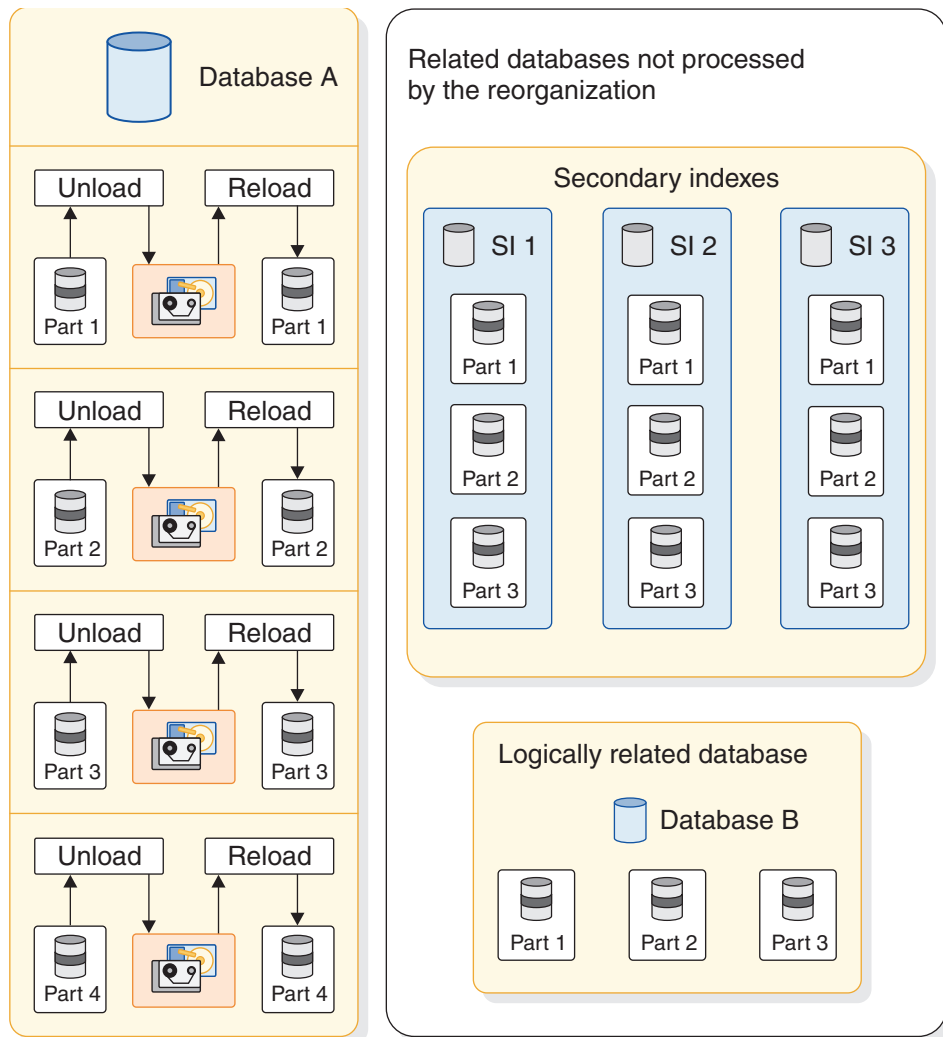
Figure 268. Offline reorganization of a HALDB database
