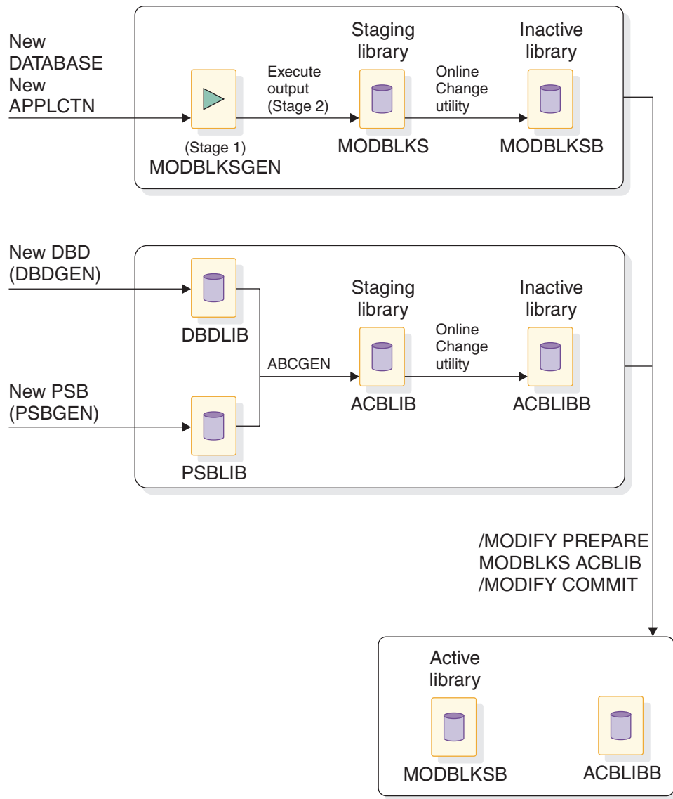
Figure 295. Adding a database using online change
