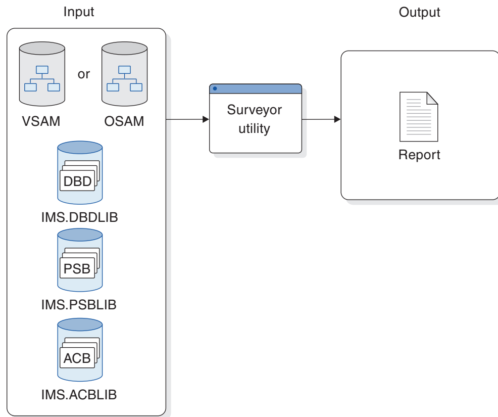
Figure 266. Database Surveyor utility (DFSPRSUR)
