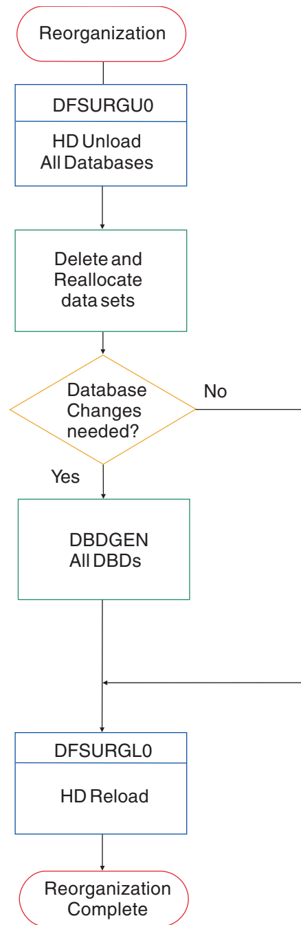
Figure 292. Flow chart of process for modifying a database to use multiple data set groups
