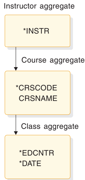
Figure 225. Instructor schedules conceptual data structure
