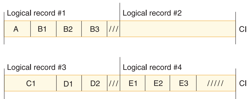
Figure 233. Logical records example with two read operations
