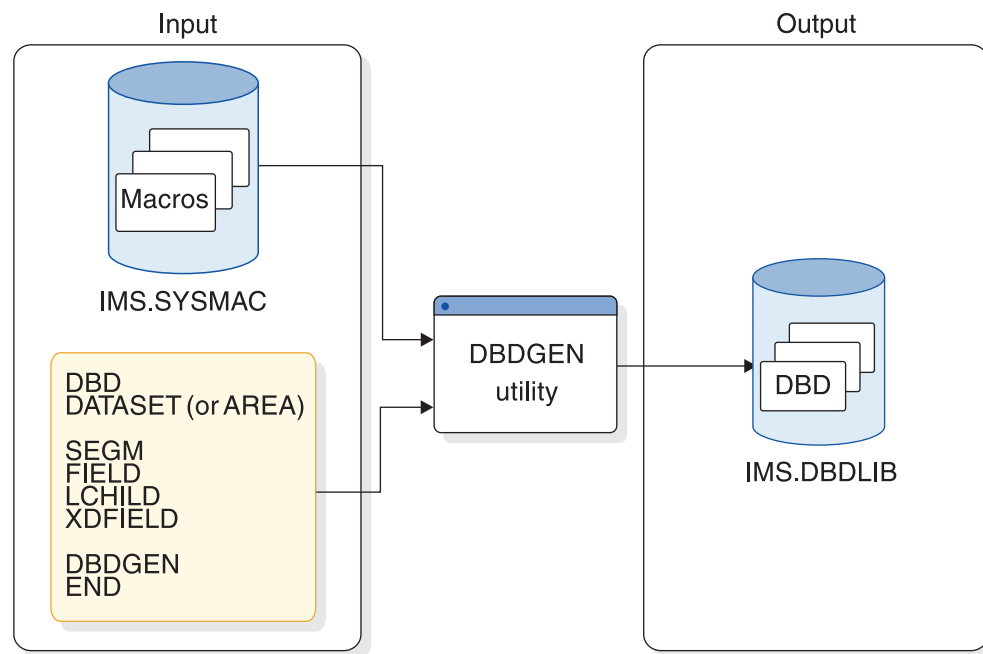
Figure 237. The DBD generation process
