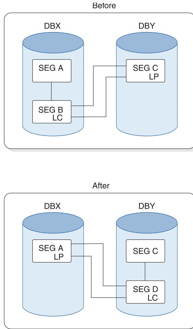
Figure 291. The position change of a real logical child from one logically related database to another
