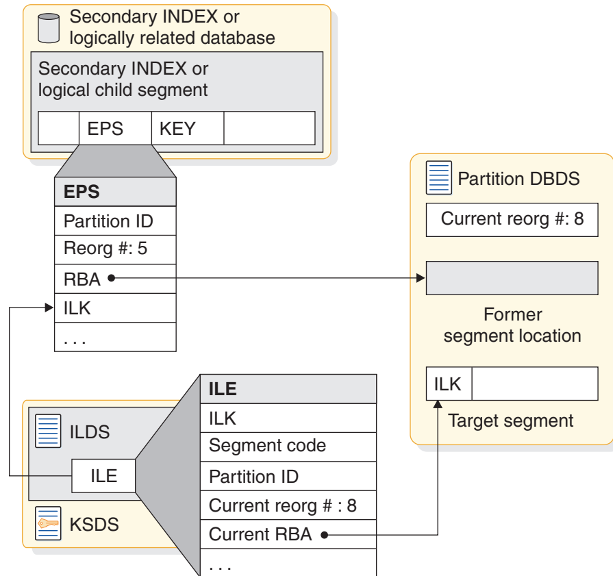
Figure 274. HALDB pointer after a reorganization
