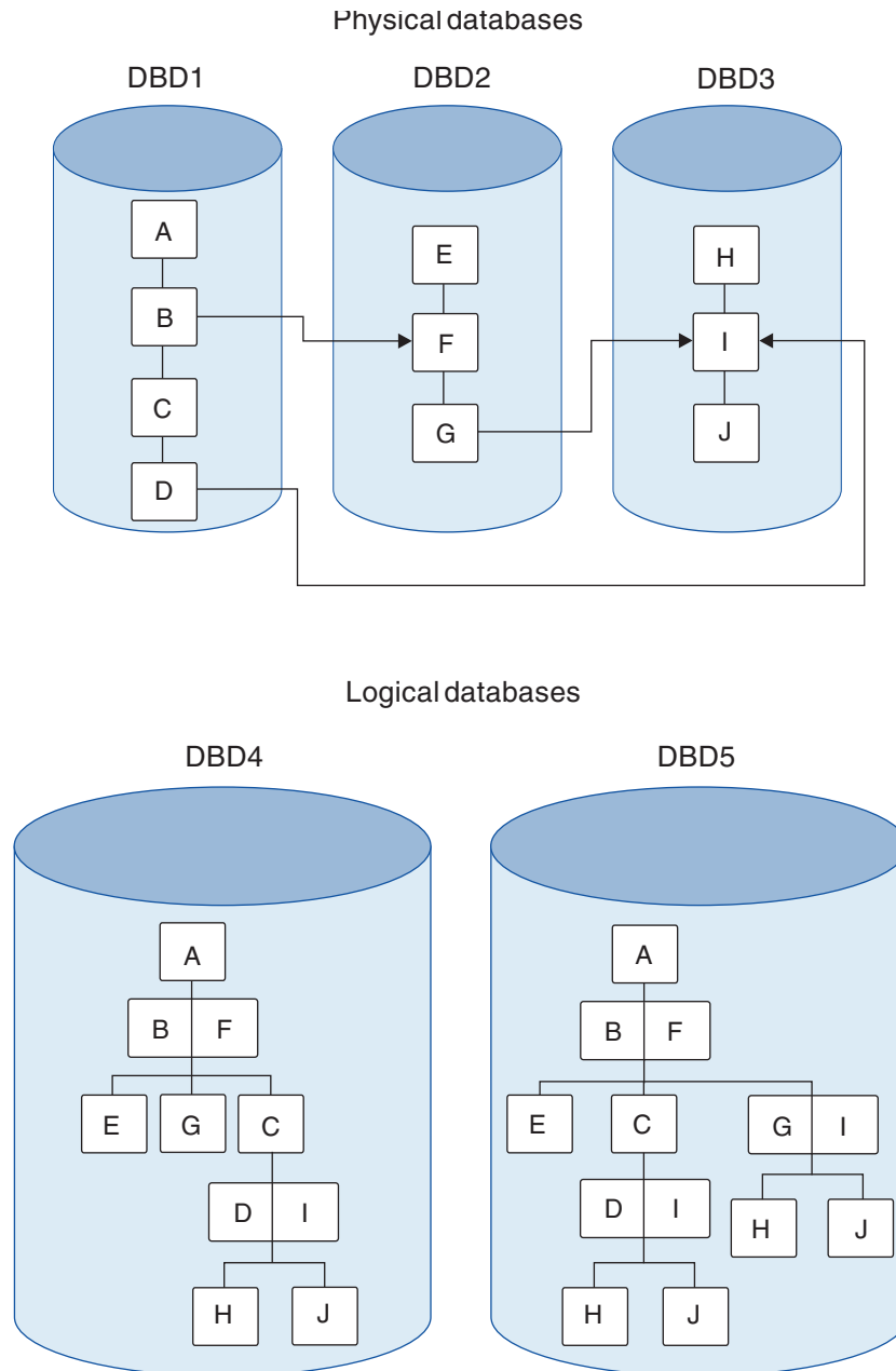
Figure 96. The first logical relationship crossed in a hierarchical path of a logical database
