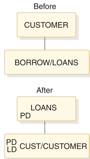
Figure 130. Logical parent, virtual pairing—virtual delete rule example: before and after
