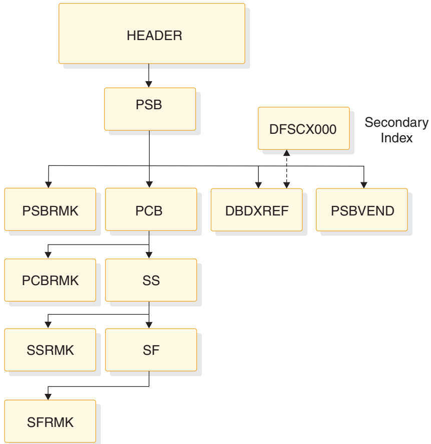
Figure 18. Format of an IMS catalog record for a program specification block
