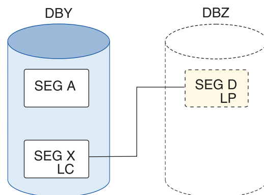
Figure 286. DBY exists, DBZ is to be added
