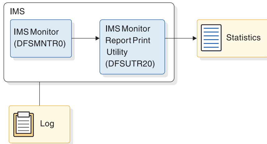
Figure 252. How the IMS Monitor works
