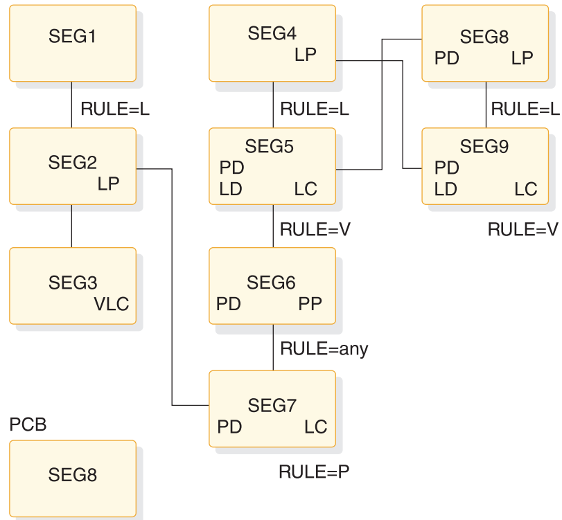
Figure 159. Example of violation of the physical delete rule
