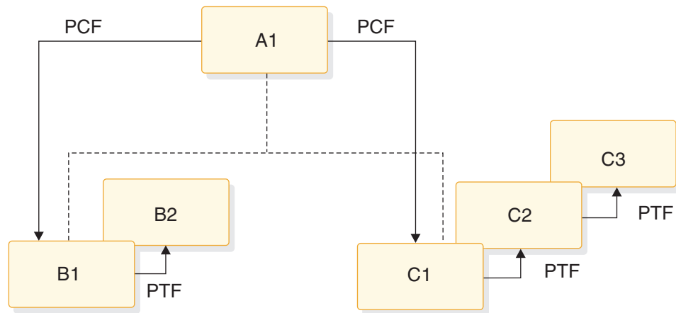
Figure 55. How dependent segments are found using PCF and PTF pointers
