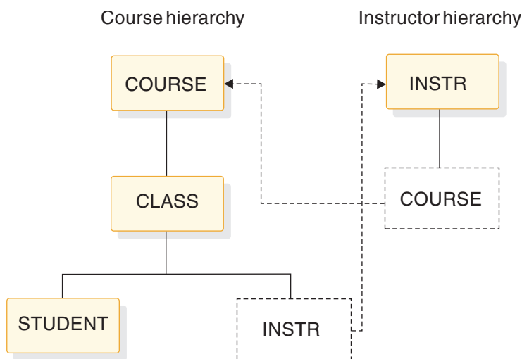
Figure 228. Bidirectional logical relationships
