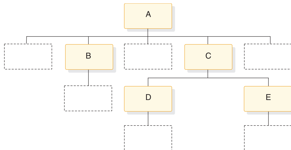
Figure 276. Where segment types can be added in a database record
