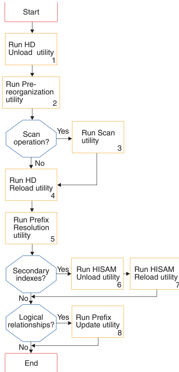
Figure 254. Steps in reorganizing when logical relationships or secondary indexes exist
