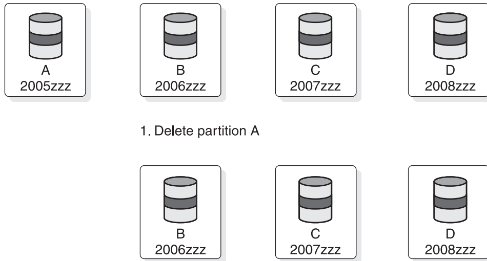
Figure 303. Deleting the partition with the lowest key in a HALDB that uses key range partitioning
