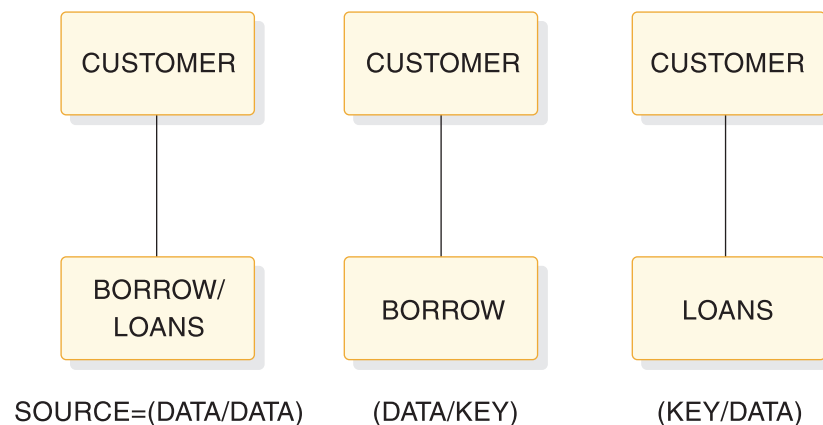
Figure 163. Concatenated segment relationships
