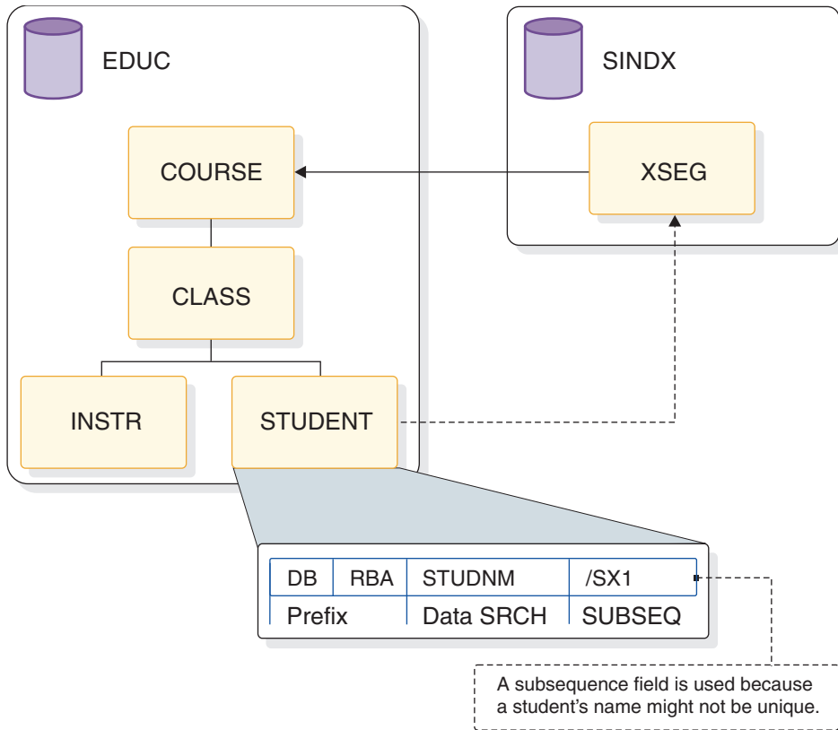
Figure 193. Databases for secondary indexing example
