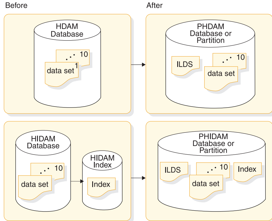
Figure 304. HDAM and HIDAM databases before and after changing to PHDAM and PHIDAM
