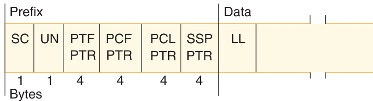
Figure 62. Direct dependent segment format
