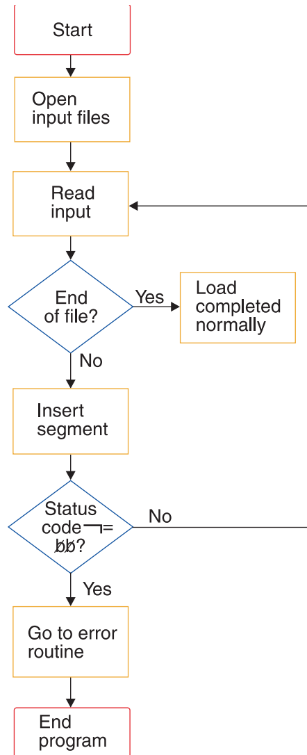
Figure 247. Basic initial load program logic
