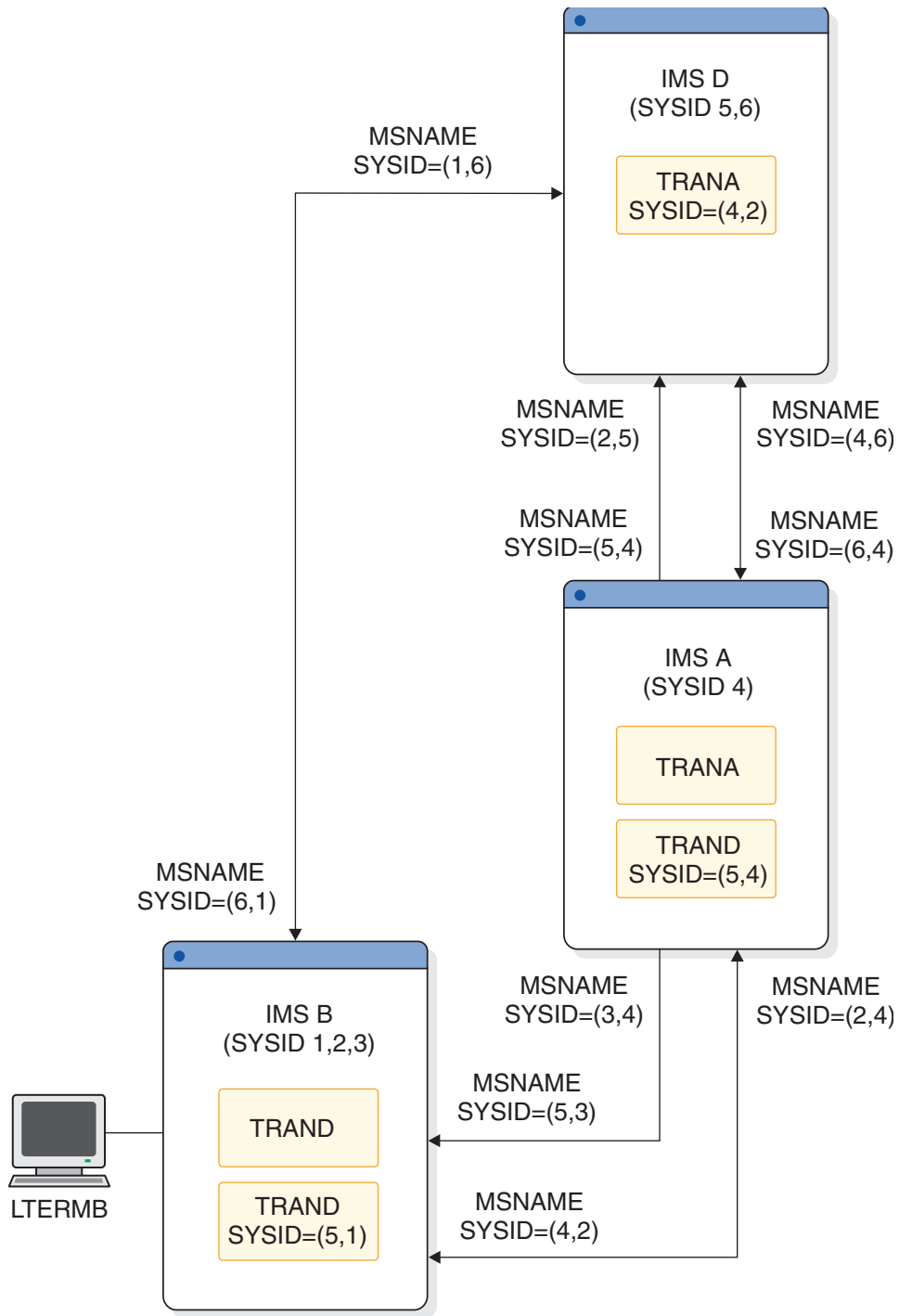
Figure 119. Message routing
