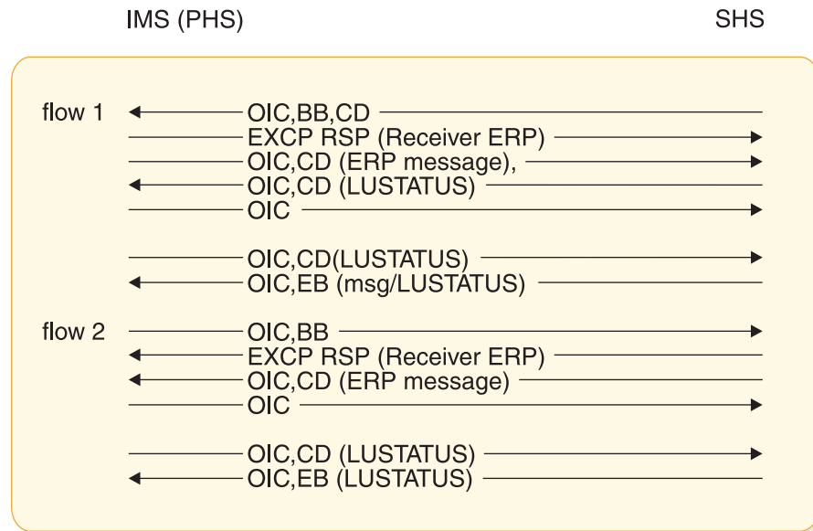
Figure 110. Example of receiver ERP for an IMS component defined as MULT2
