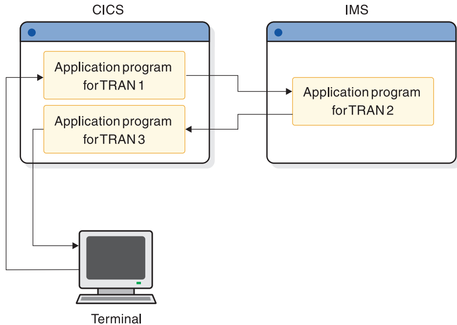
Figure 83. Asynchronous processing with START and RETRIEVE
