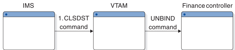
Figure 158. Termination processing
