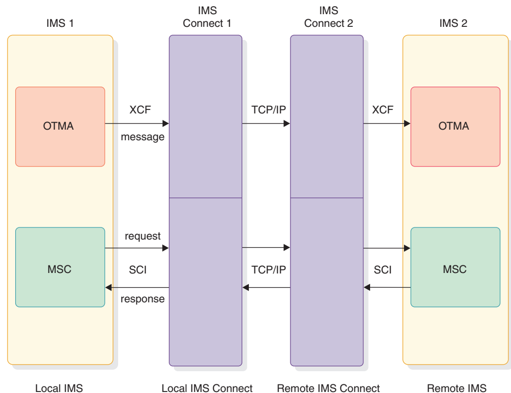
Figure 24. Example configuration for IMS-to-IMS TCP/IP communications
