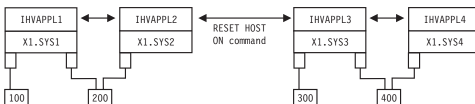
Figure 148. RESET HOST Command: Scenario 2
