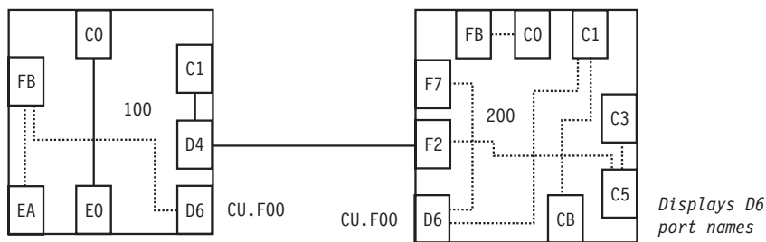
Figure 138. DISPLAY NAME Command: Sample 2
