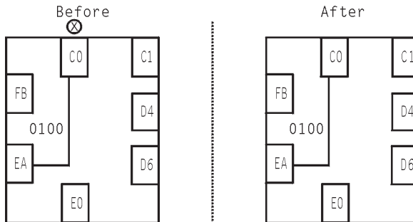
Figure 166. UNBLOCK Command Example
