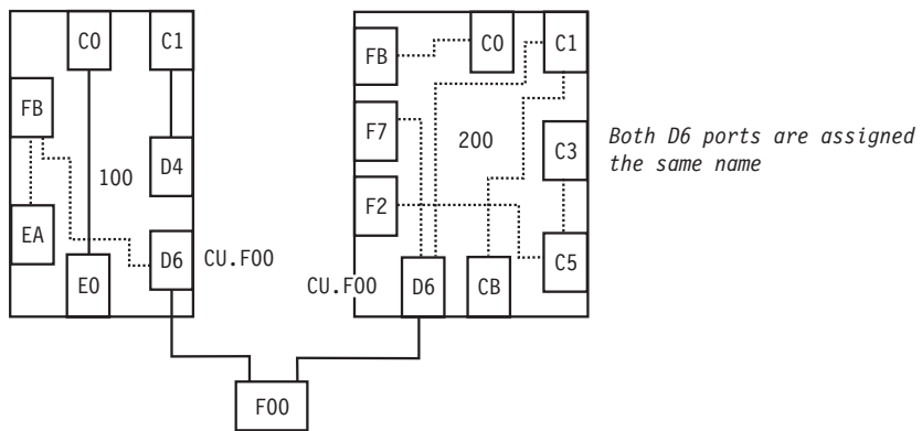
Figure 153. WRITE Command: Sample 2
