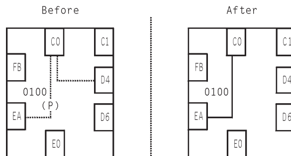
Figure 164. CONNECT Command Example
