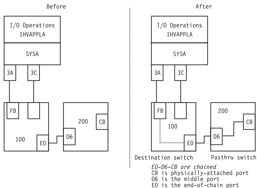
Figure 130. CHAIN Command: Sample 2
