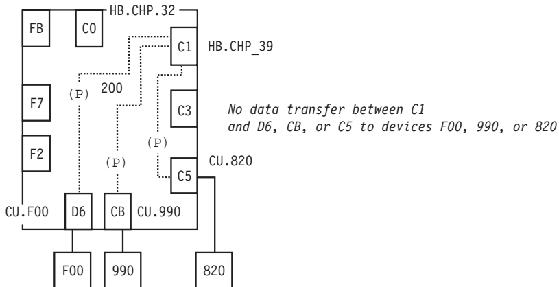
Figure 145. PROHIBIT Command: Sample 2
