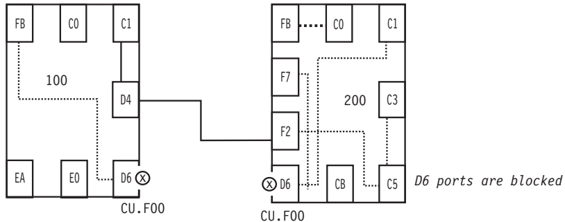
Figure 128. BLOCK Command: Sample 2
