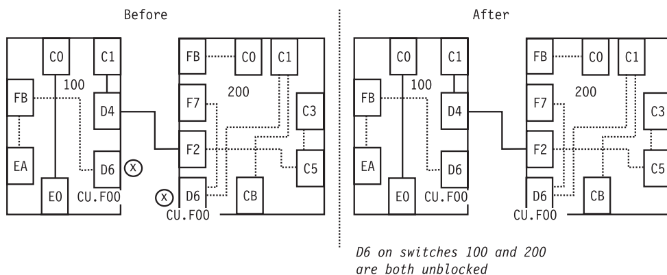
Figure 150. UNBLOCK Command: Sample 2
