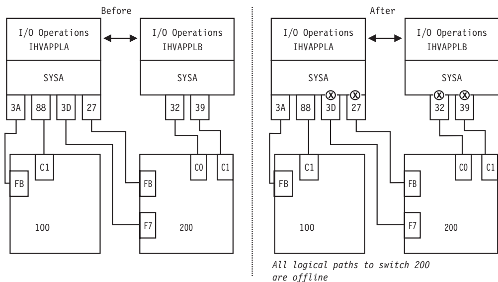
Figure 146. REMOVE SWITCH Command Sample
