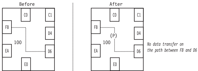
Figure 144. PROHIBIT Command: Sample 1
