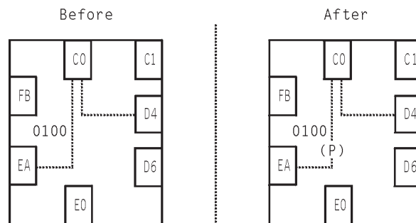
Figure 163. PROHIBIT Command Example
