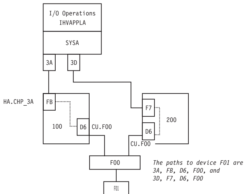
Figure 134. DISPLAY DEV Command Sample
