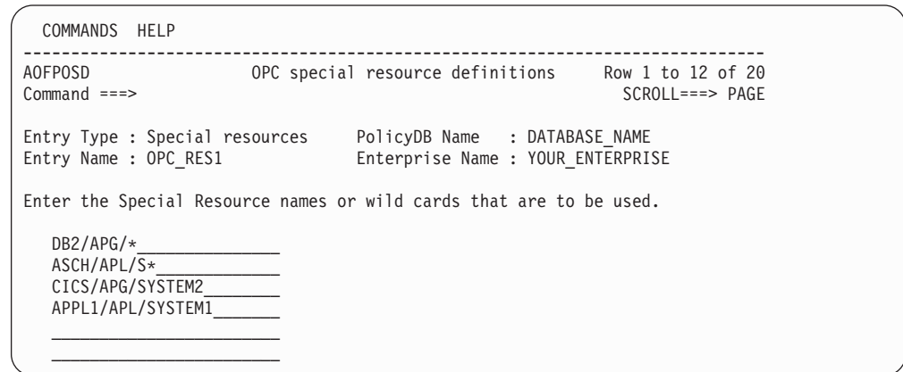
Figure 199. OPC Special Resource Definitions Panel
