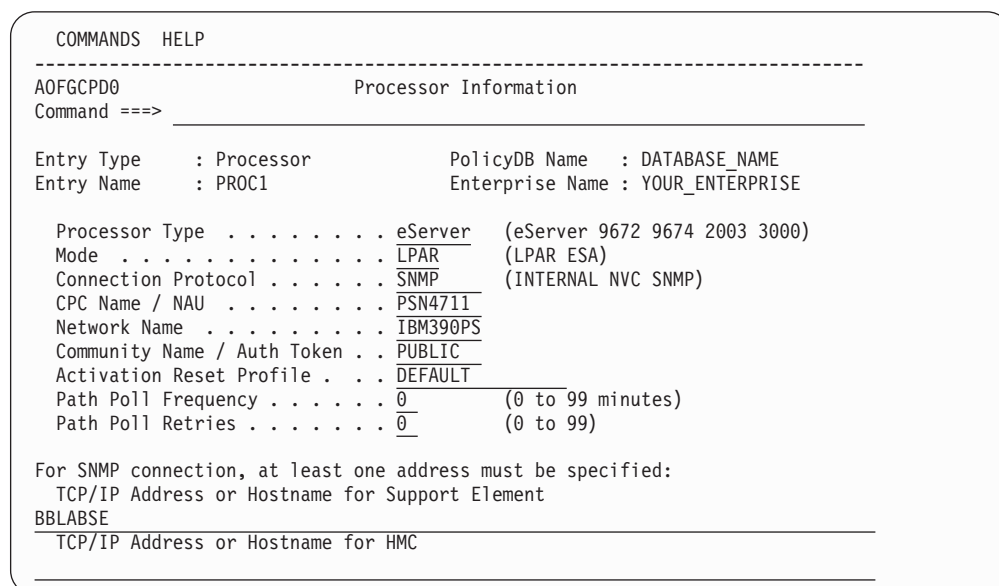
Figure 171. Processor Information Panel
