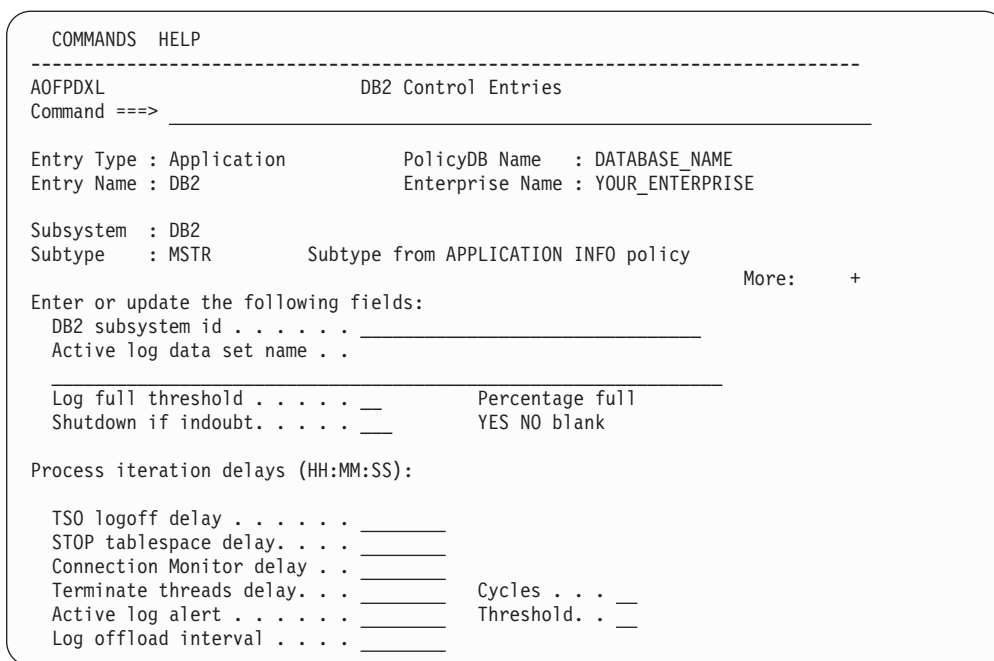
Figure 151. DB2 Control Entries Panel
