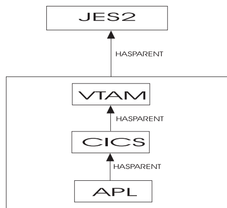
Figure 22. Relationship between Applications and Application Groups
