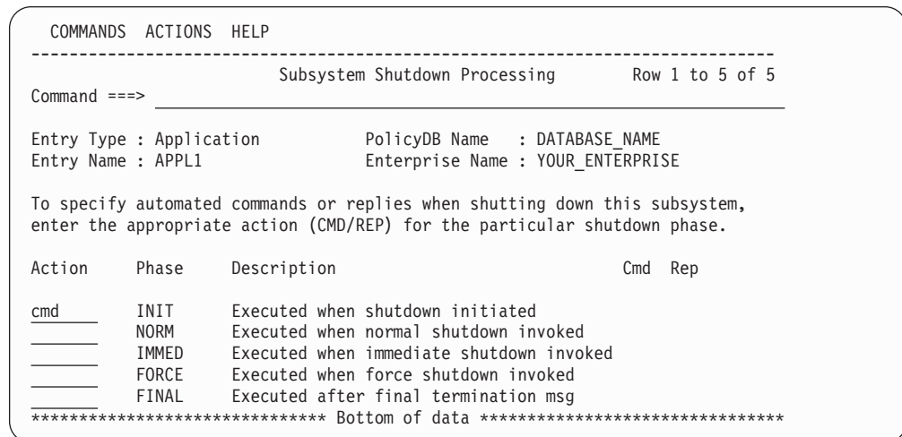
Figure 125. Subsystem Shutdown Processing Panel
