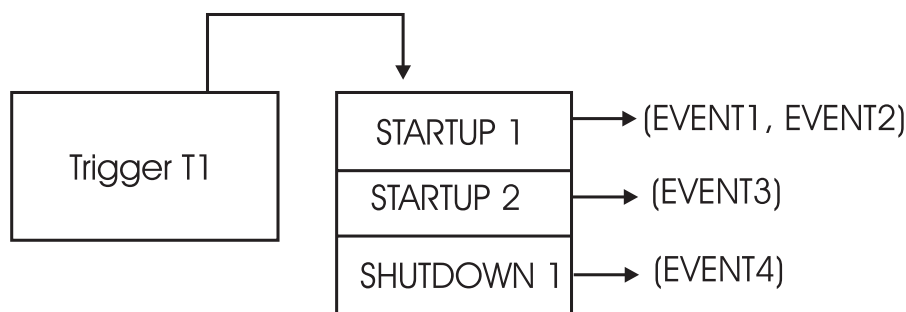
Figure 27. How a Trigger Uses Events
