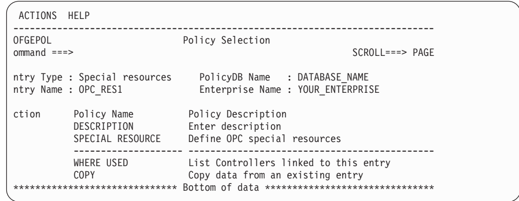
Figure 198. Policy Selection Panel for OPC Special Resources
