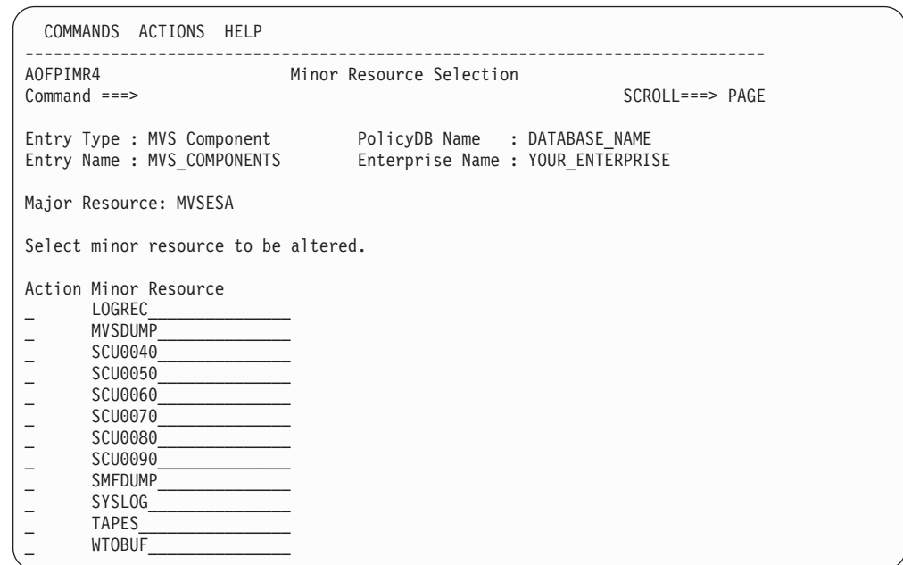
Figure 212. Minor Resource Selection Panel
