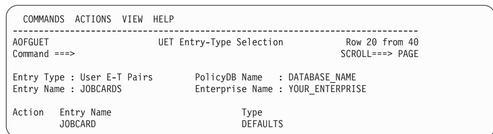
Figure 233. UET Entry-Type Selection Panel
