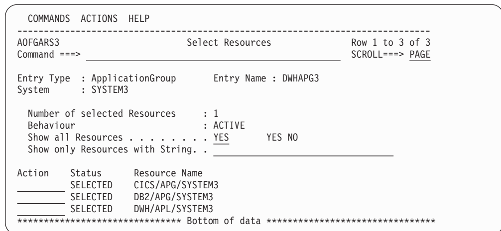
Figure 43. Select Resources Panel for DWHAPG3
