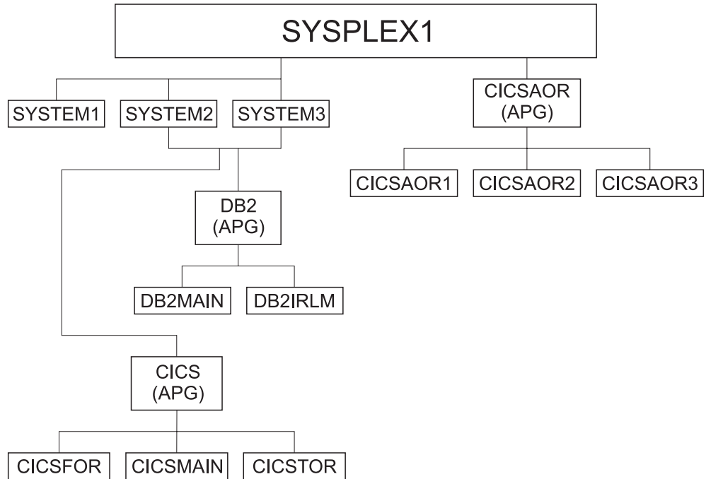
Figure 38. Current Configuration with Applications Linked to DB2
