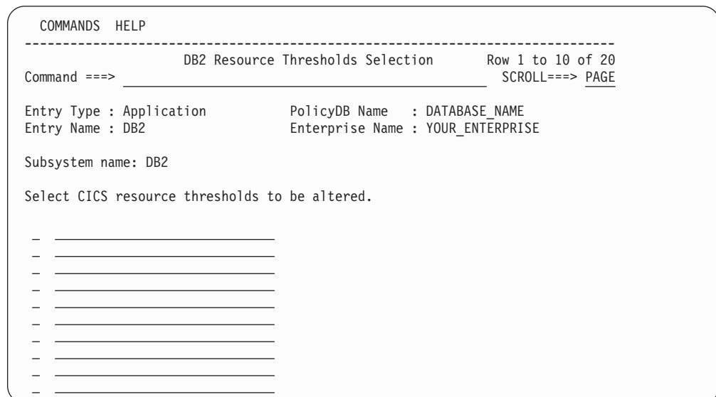
Figure 152. DB2 Resource Thresholds Selection Panel
