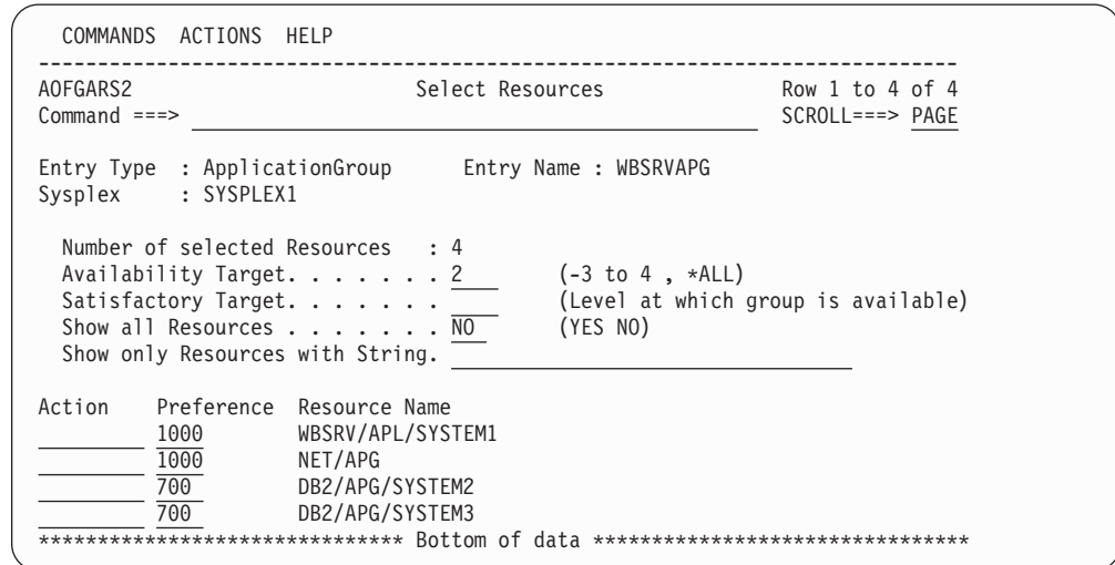
Figure 48. Final Select Resources Panel for WBSRVAPG
