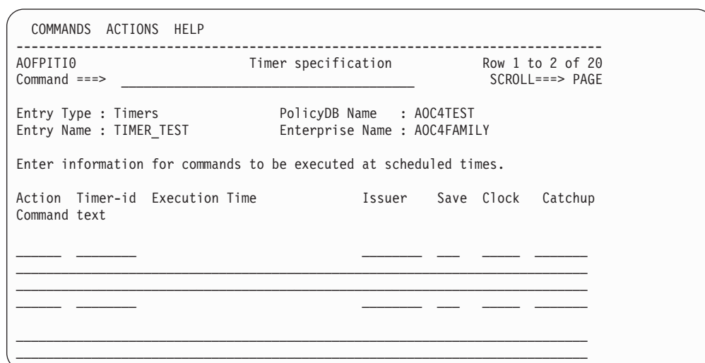
Figure 202. Timer Specification Panel
