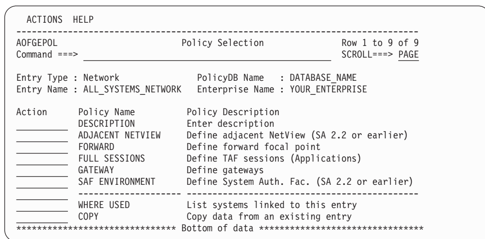
Figure 225. Policy Selection Panel for Network
