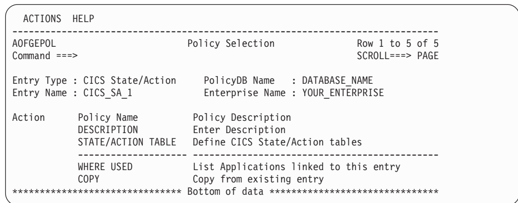
Figure 182. Policy Selection Panel for CICS State/Action Tables
