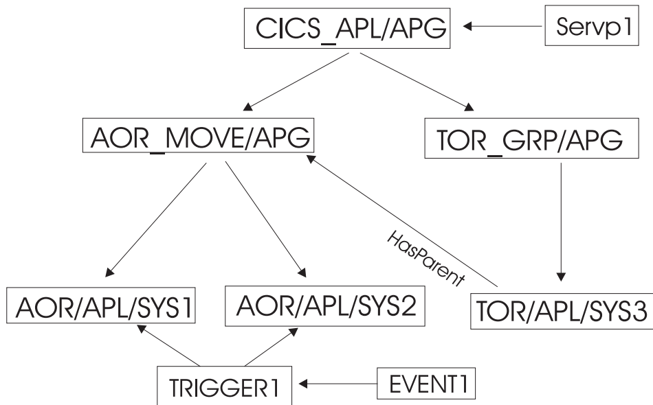
Figure 49. Scenario with Triggers, Events and Service Period
