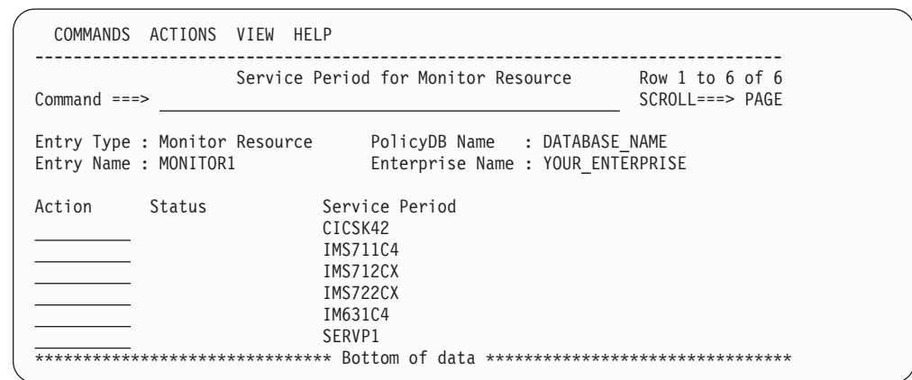
Figure 179. Service Period for Monitor Resource Panel
