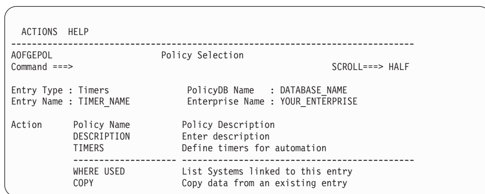
Figure 201. Policy Selection Panel for Timers
