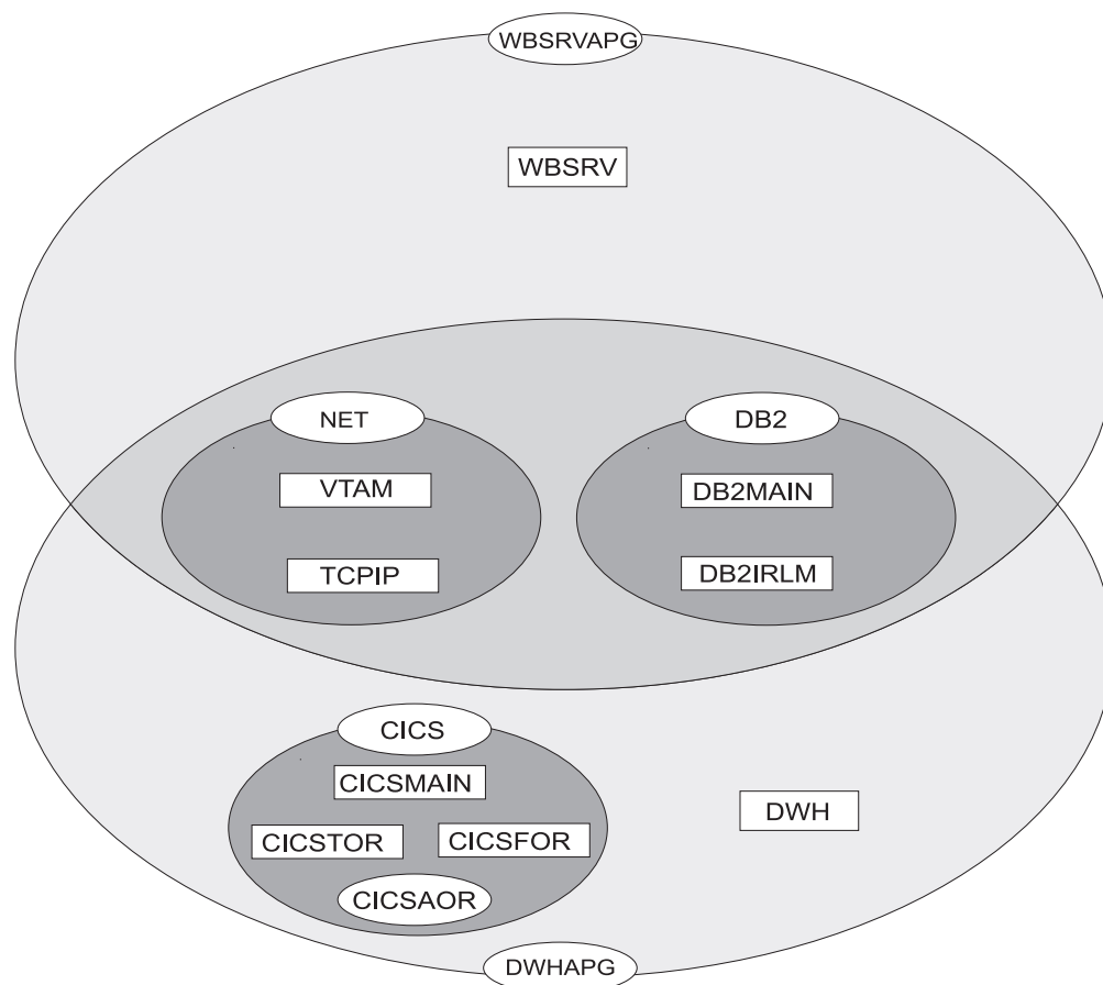
Figure 18. Grouping of Applications into Nested ApplicationGroups
