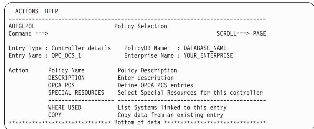
Figure 196. Policy Selection Panel for OPC Controller Details
