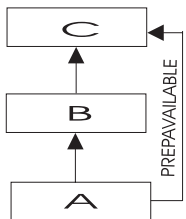
Figure 122. Using STARTUP Policy
