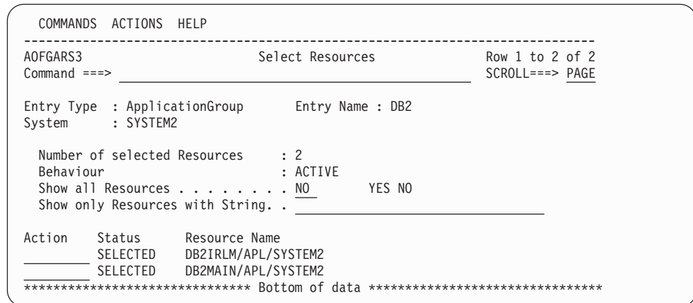
Figure 35. Select Resources Panel for DB2 Application Group
