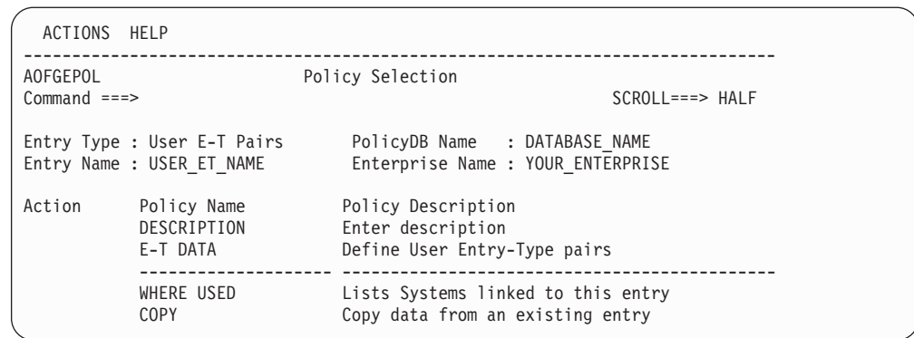
Figure 232. Policy Selection Panel for User E-T Pairs
