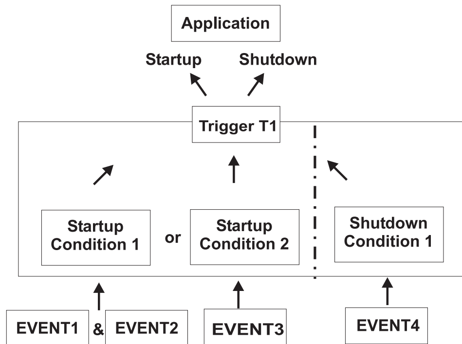
Figure 28. Triggers, Events and Conditions
