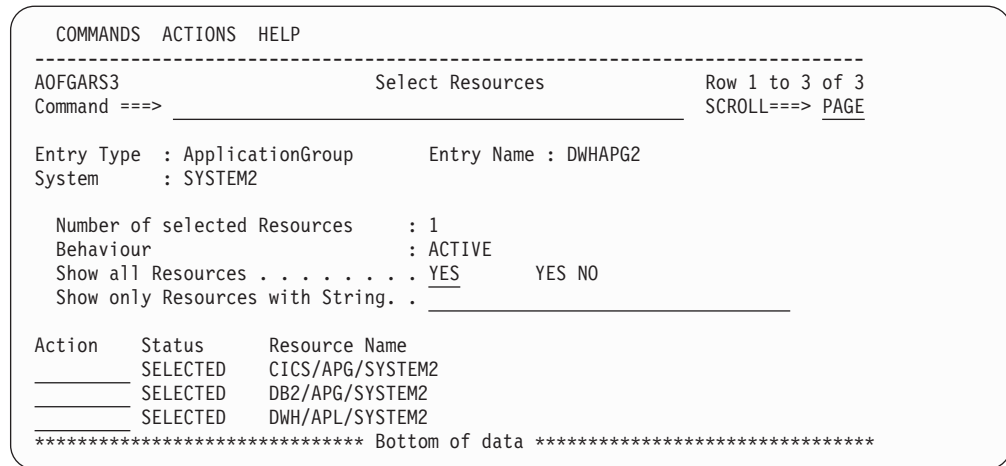
Figure 42. Select Resources Panel for DWHAPG2
