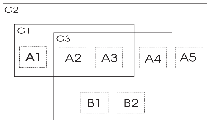
Figure 16. Example of Aggregating Applications into Application Groups
