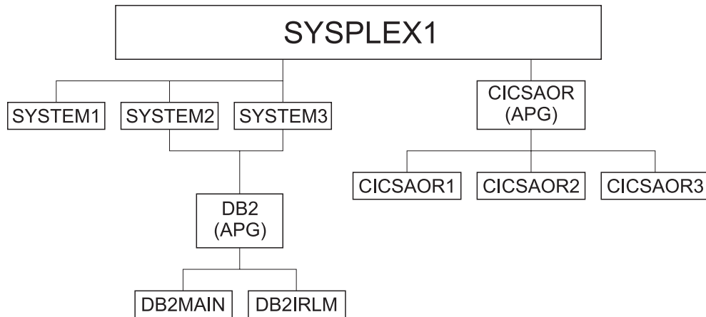
Figure 33. Current Configuration with Applications Linked to DB2
