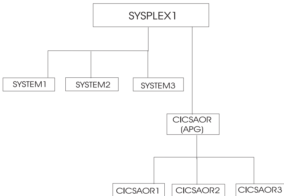
Figure 30. Current Configuration with Applications CICSAOR1 through CICSAOR3
