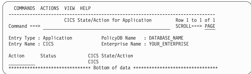
Figure 148. CICS State/Action for Application Panel
