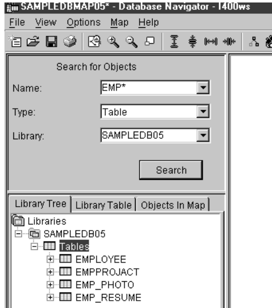
Figure 17. Advance search using the Locator pane
