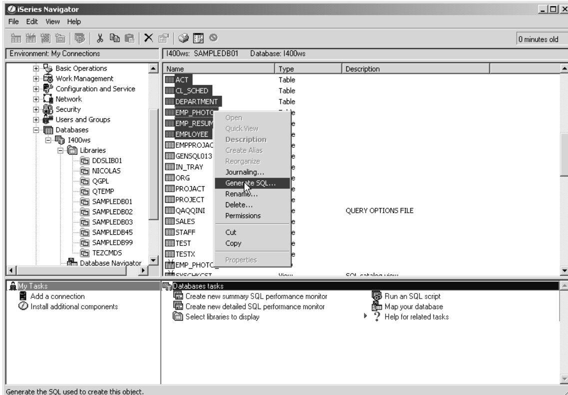
Figure 54. Selecting objects from the library to generate SQL
