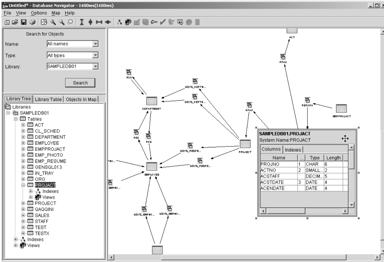
Figure 45. Expanding the table in a map
