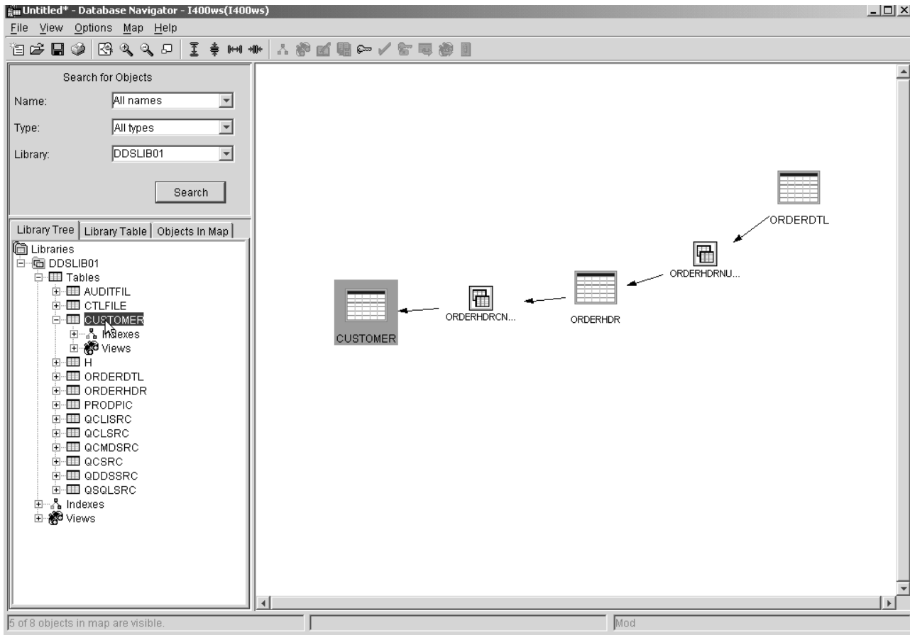
Figure 87. Map of DDSLIB01
