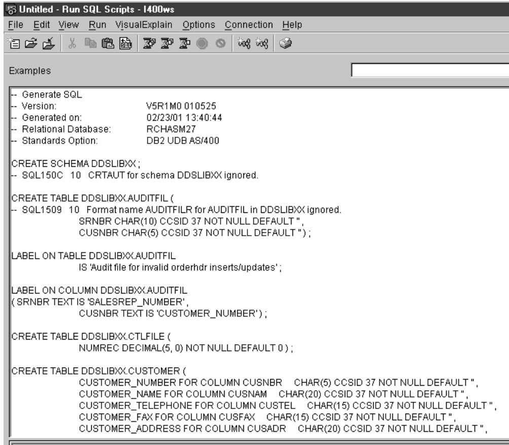
Figure 84. Exploring SQL script generated from a physical file
