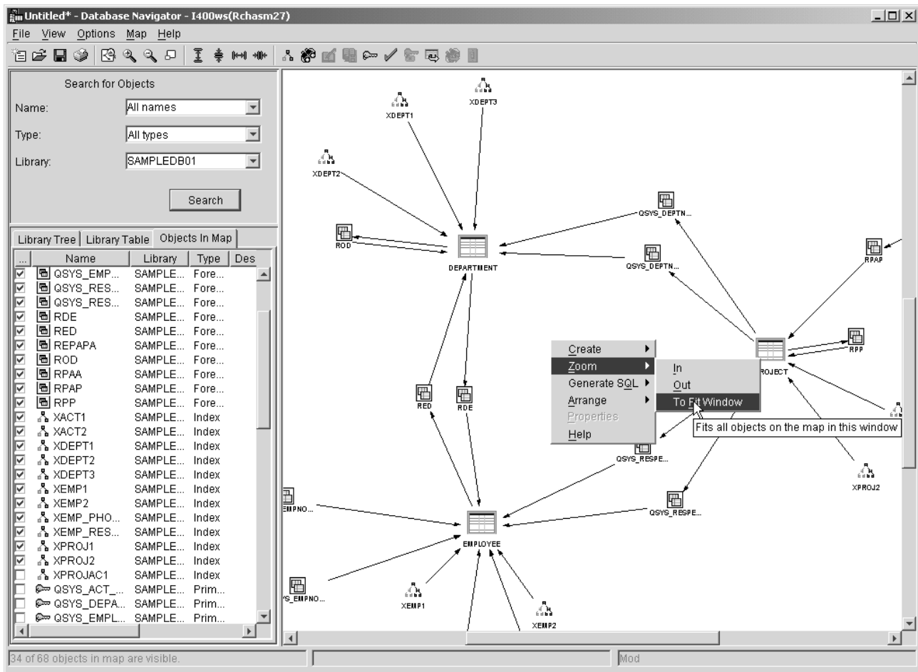
Figure 22. Selecting To Fit Window
