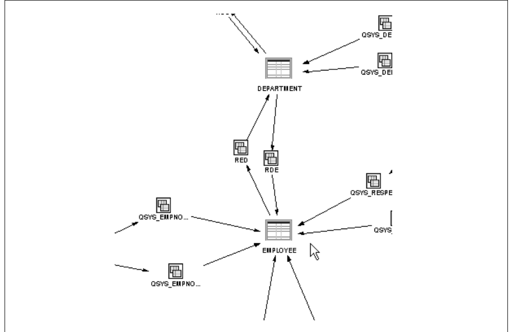
Figure 77. Showing a Referential Constraints Key in the map
