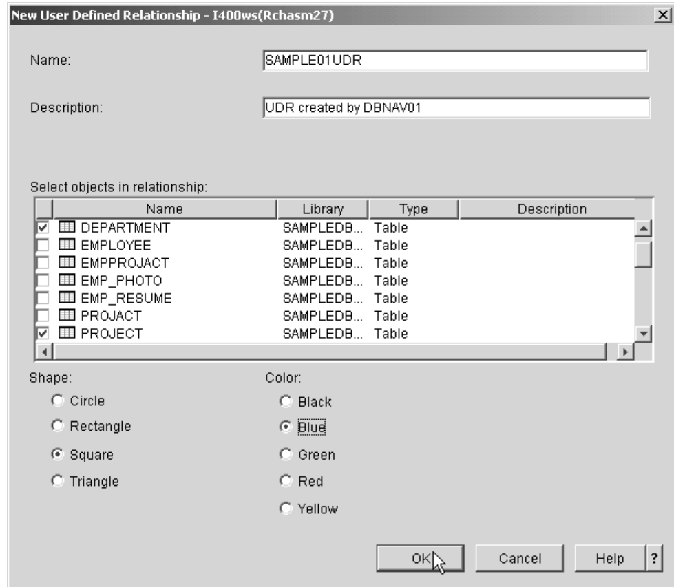
Figure 48. Creating a user-defined relationship
