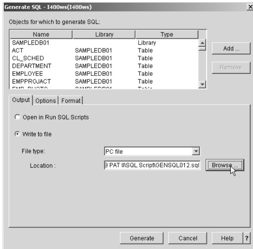
Figure 61. Selecting Generate SQL to PC
