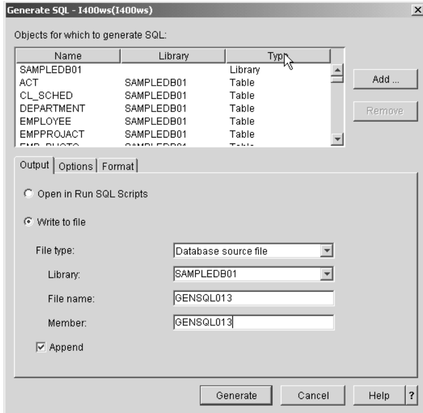
Figure 68. Generating SQL to the iSeries server
